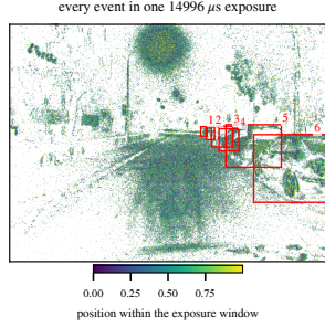
Figure 7. Every event inside one published 14996 \mu\text{s} exposure window of zurich_city_09_a, colored by its position within that window, with that frame’s released boxes numbered left to right. The frame is the median-dispersion one of 602 eligible candidate frames with at least six qualifying boxes, not the largest.
