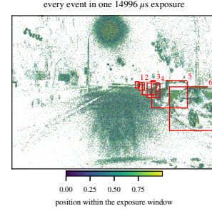
Figure 3. Every event inside one published 14\,996\,\mu\text{s} exposure window of zurich_city_09.a , colored by its position within that window, with that frame's released boxes numbered left to right. The frame is the median-dispersion one of 602 eligible candidate frames with at least six qualifying boxes, not the largest.
