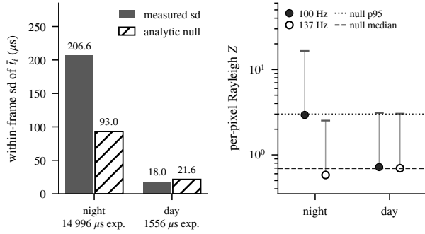
Figure 2. Left: within-frame dispersion of \bar{t}_i against its analytic null in the two exposure strata, 1134 frames of zurich_city_09.a at 14\,996\,\mu\text{s} and 20 frames of interlaken_00.c at 1556\,\mu\text{s} . The daytime frames are selected by retaining frames with at least three qualifying boxes. Right: per-pixel Rayleigh statistic Z = R^2/N at 100 Hz and at 137 Hz for the same two sequences, median with a whisker to the ninety-fifth percentile, against the \text{Exp}(1) null. Both contrasts run in the same direction, and Main Sec. 4.4 reports the controls applied to that dispersion.
