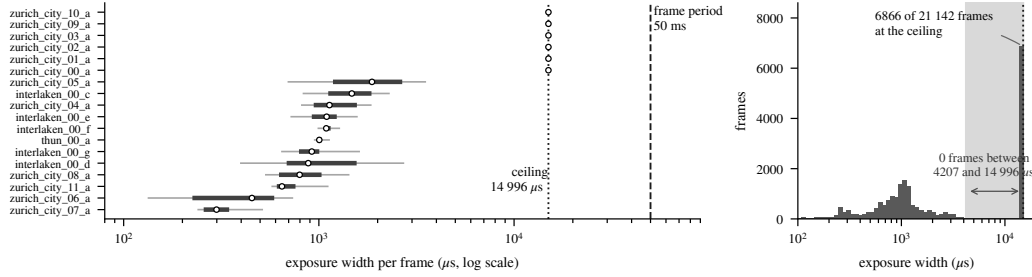
Figure 6. Published per-frame exposure width across the eighteen DSEC training sequences whose exposure files resolve: per sequence (left, log axis, median, interquartile range and 5–95 % band, against the fixed 50 ms frame period) and pooled over 21 142 frames (right). 32.5 % of frames sit at the auto-exposure ceiling of 14 996 \mu s and zero fall between the largest non-ceiling width of 4207 \mu s and that ceiling, separating the two exposure regimes. The six ceiling sequences are those measured in Sec. 16.
