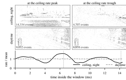
Figure 7. Top: 350 \mu s slices of the ceiling-exposure sequence zurich.city_09_a and of the daytime control, at the peak and trough of the ceiling sequence's own event rate inside its densest published exposure window. Bottom: that rate in 350 \mu s bins, each sequence normalized to its own mean. The ceiling rate moves by a factor of 3.0 between its extremes, the daytime rate by 1.1.
