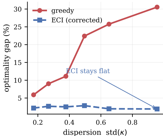
(b) Gap grows with dispersion
