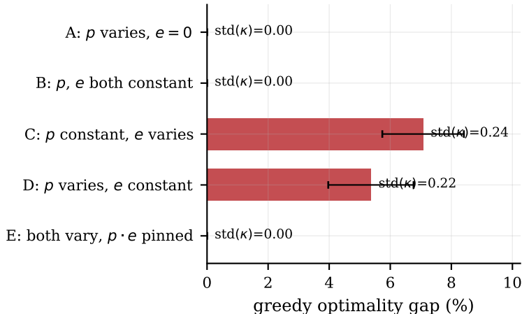
(a) Greedy fails iff \kappa = p e varies
