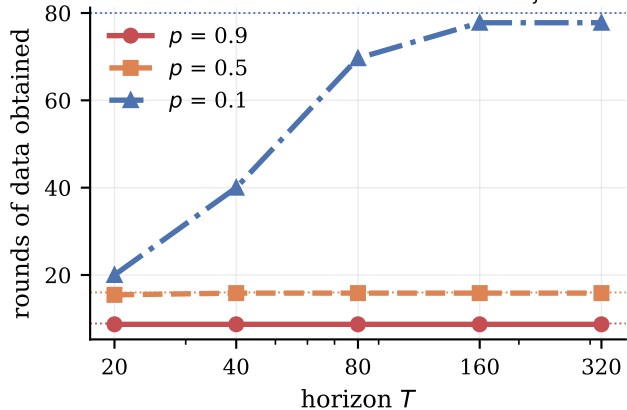
(b) Sample budget caps at \sum_j 1/p_j
