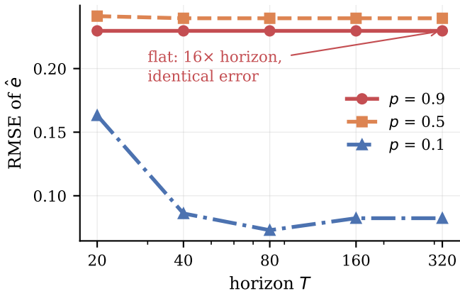
(a) More horizon buys nothing
