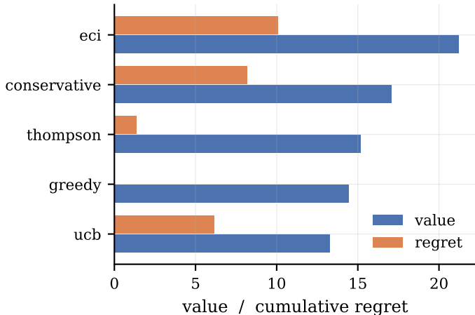
(b) Rankings are reversed ( \text{std}(e)=1.5 )
