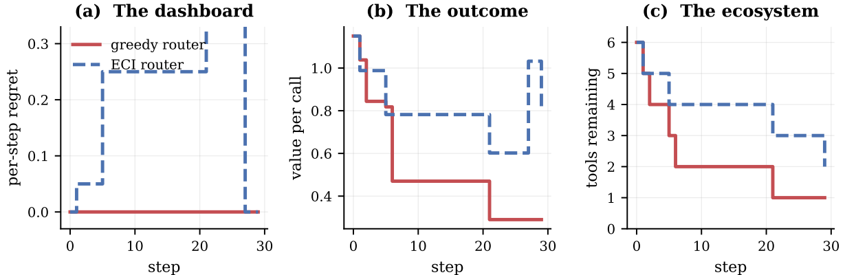
Figure 5: A single routing session, identical seed and tool set. (a) The metric: greedy’s per-step regret is zero throughout, while the corrected router accrues visible regret. (b) Value per call: the router with worse regret delivers more. (c) Surviving tools: the router with worse regret preserves more of the ecosystem. The visible regret in (a) is the price of preservation , and the standard metric records it as a defect.
