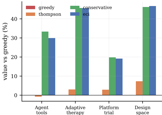
(a) Correction pays in every domain
