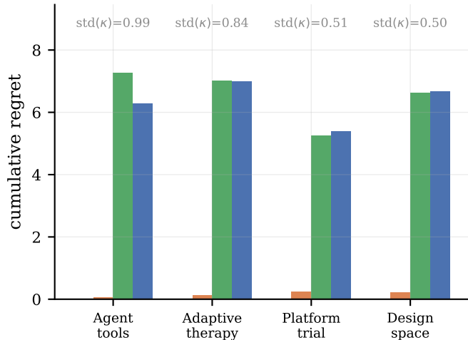
(b) Greedy reports zero regret everywhere
