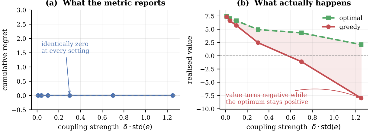
Figure 1: The central phenomenon. (a) Greedy’s cumulative regret against the best-available-arm benchmark, computed exactly: identically zero at every coupling strength, because greedy never fails to pull the best arm currently available. (b) Realised value on the same instances. The shaded region is the loss. At strong coupling the zero-regret policy finishes net-negative while the optimum stays positive. Averages over 20 instances, n = 6 , T = 10 , exact dynamic programming.
