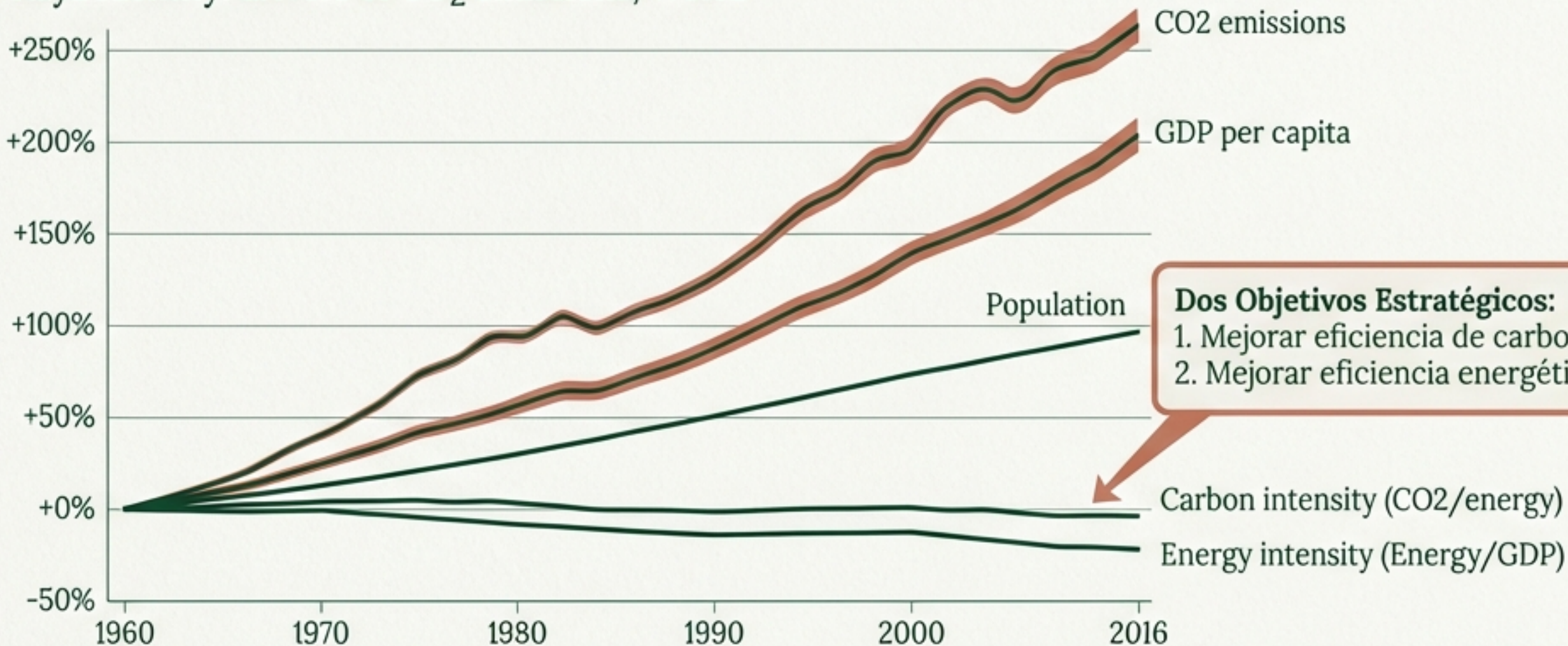
Kaya Identity: drivers of CO 2 emissions, World
