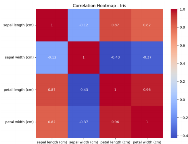
Figure 2: Correlation heatmap – Iris
