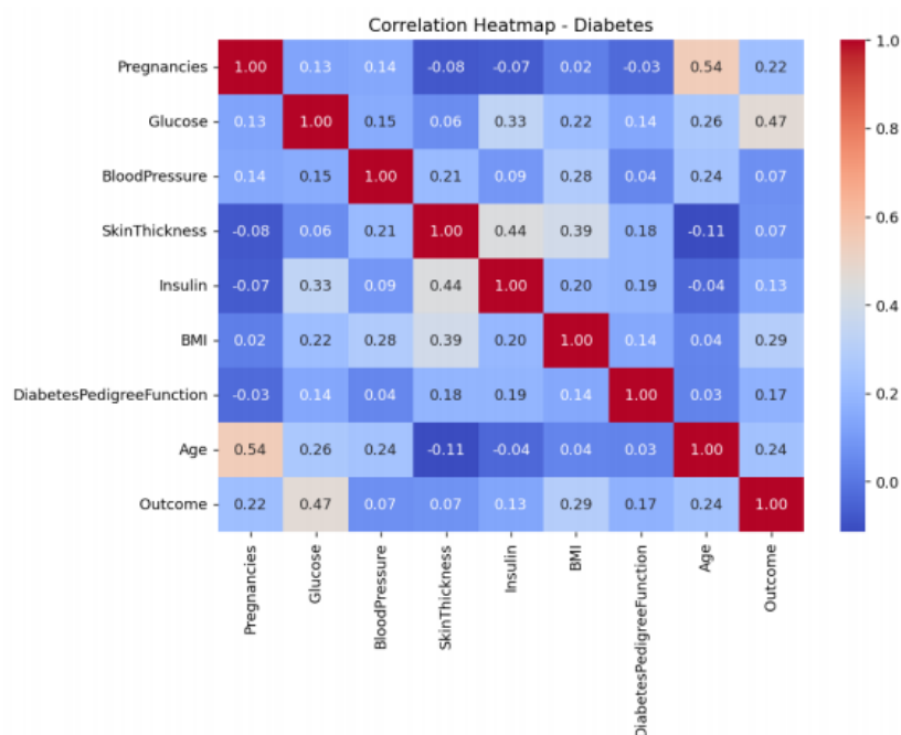
Figure 8: Correlation heatmap – Diabetes
