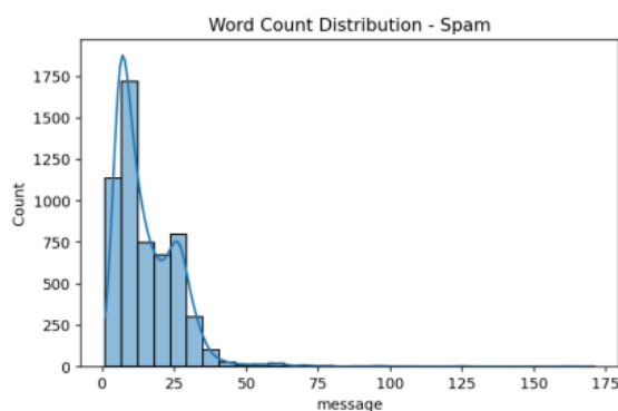
Figure 15: Word count distribution – Spam
