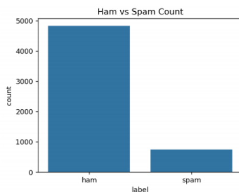
Figure 13: Ham vs. spam class distribution
