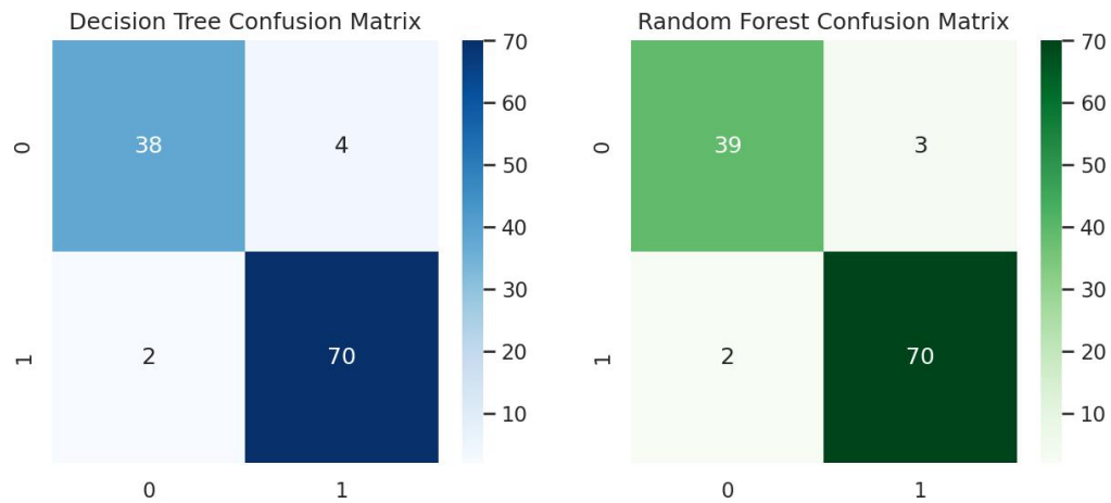
Figure 3: Confusion Matrix – Baseline Decision Tree(On left) and Tuned Random Forest(On Right)
