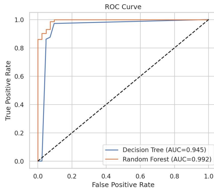
Figure 7: ROC Curve – Decision Tree vs. Random Forest
