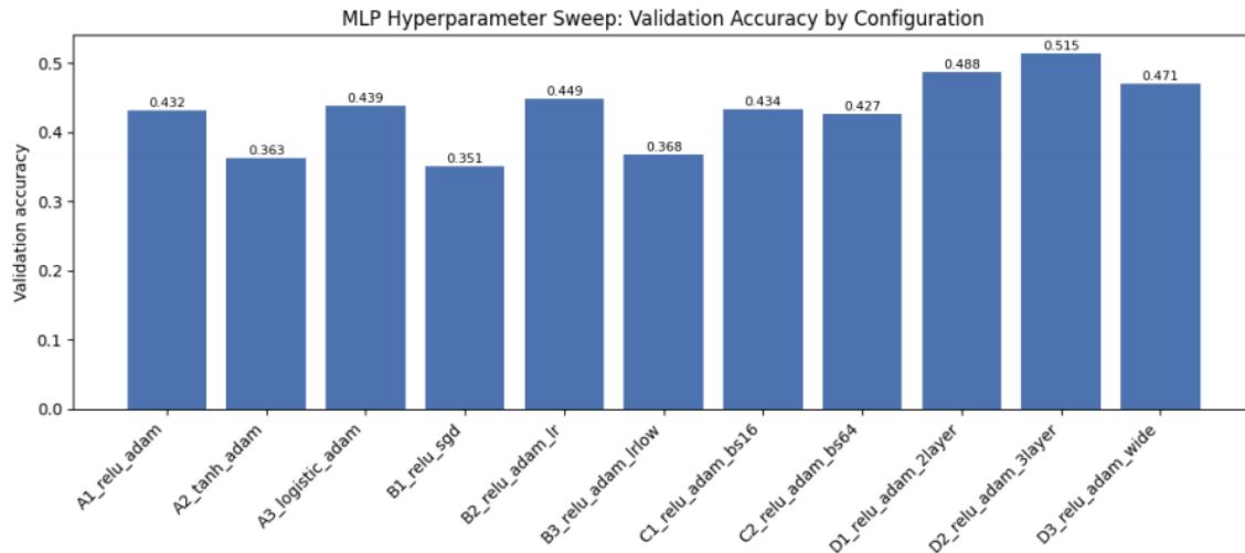
Figure 2: Validation accuracy across the 11-configuration hyperparameter sweep.
