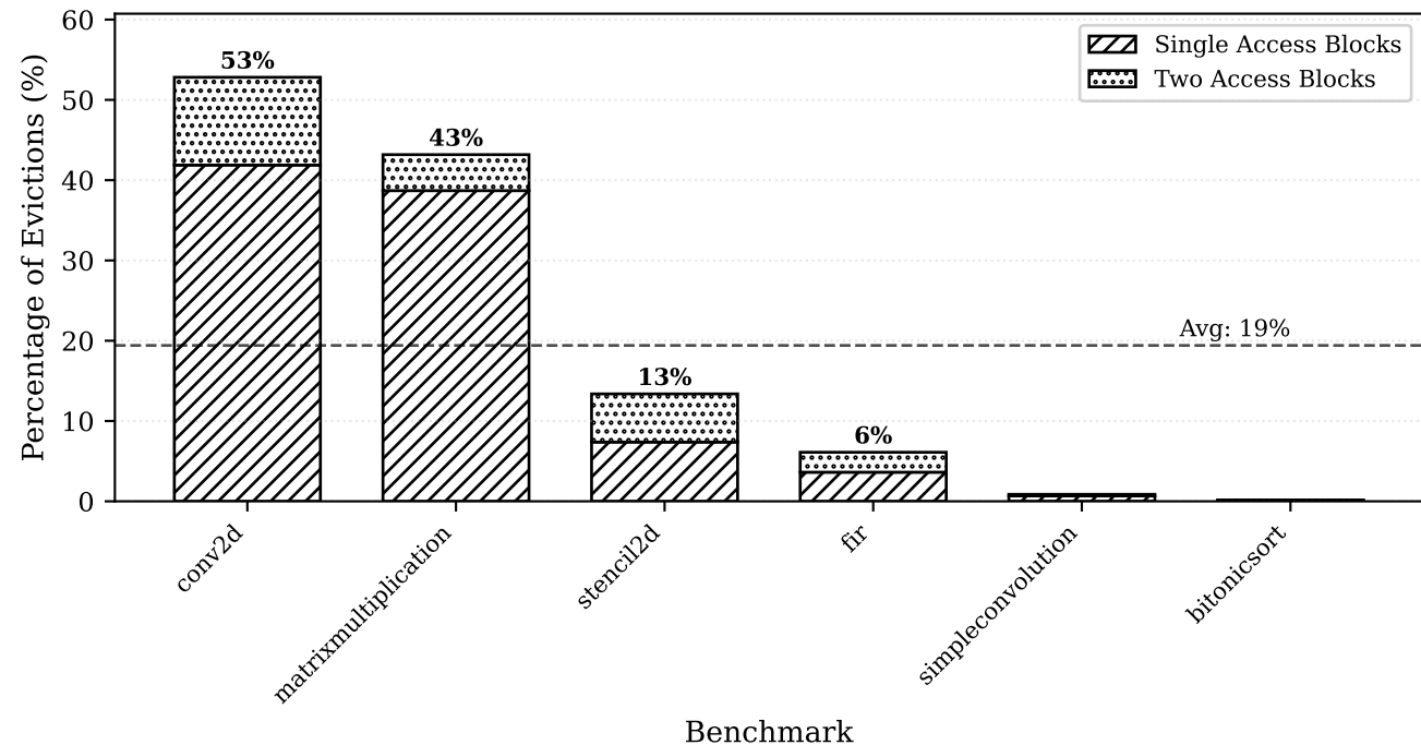
L1 Cache Dead Block Prediction Potential
