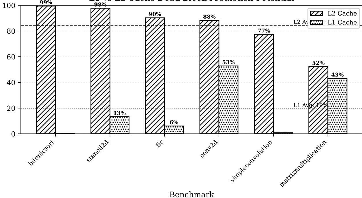
L1 vs L2 Cache Dead Block Prediction Potential
