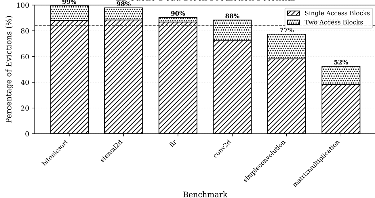
L2 Cache Dead Block Prediction Potential
