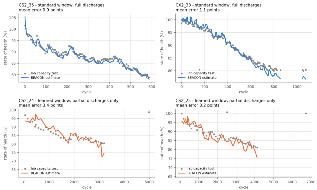
Figure 5.2: SOH from voltage, current and time against every laboratory capacity test. Top: two constant-current cells, fixed window (mean error 0.9 and 1.1 points). Bottom: two cells of real partial cycling, learned window, estimate from partial discharges only (3.4 and 3.2 points).
