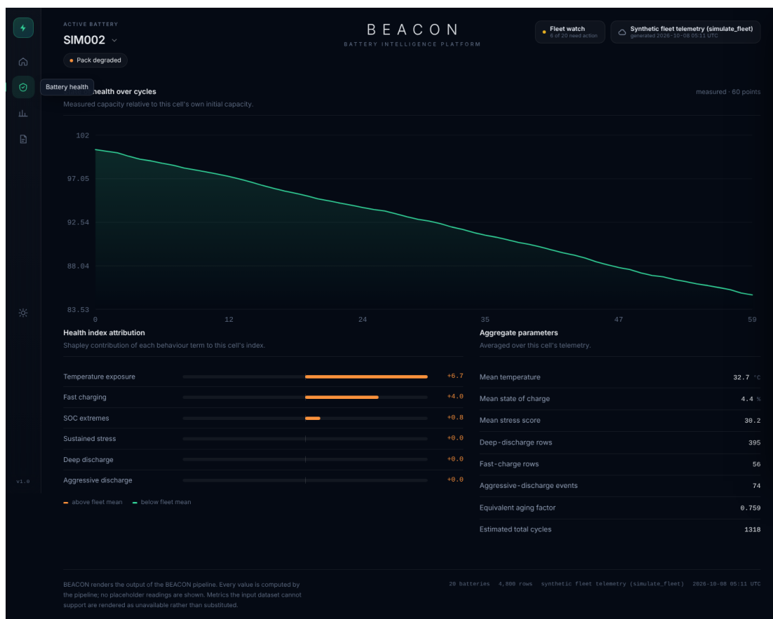
Figure 4.4: Battery health screen: state of health over cycles for one battery, the attribution of its health index to behaviour terms, and its aggregate usage parameters (synthetic fleet).
