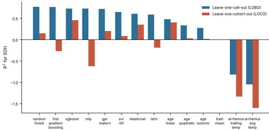
Figure 5.1: LOBO and LOCO R^2 for SOH for every scored method on the 31-cell NASA benchmark (data: benchmark_results.csv ). Skill measured across cells does not carry over to a new protocol.
