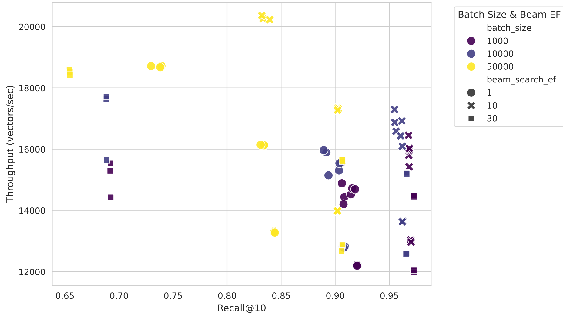
Hybrid GPU-HNSW: Pareto Frontier
