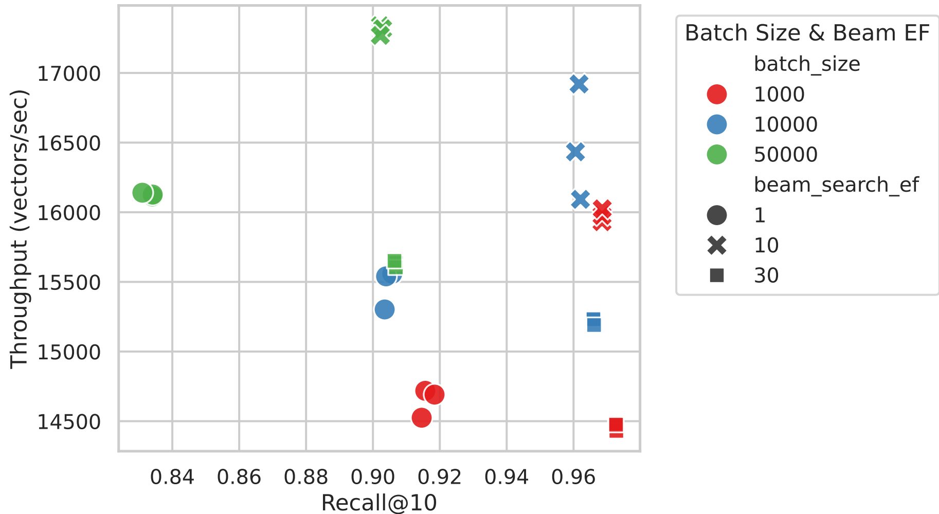
Throughput vs. Recall Trade-off (ef_construction = 200)
