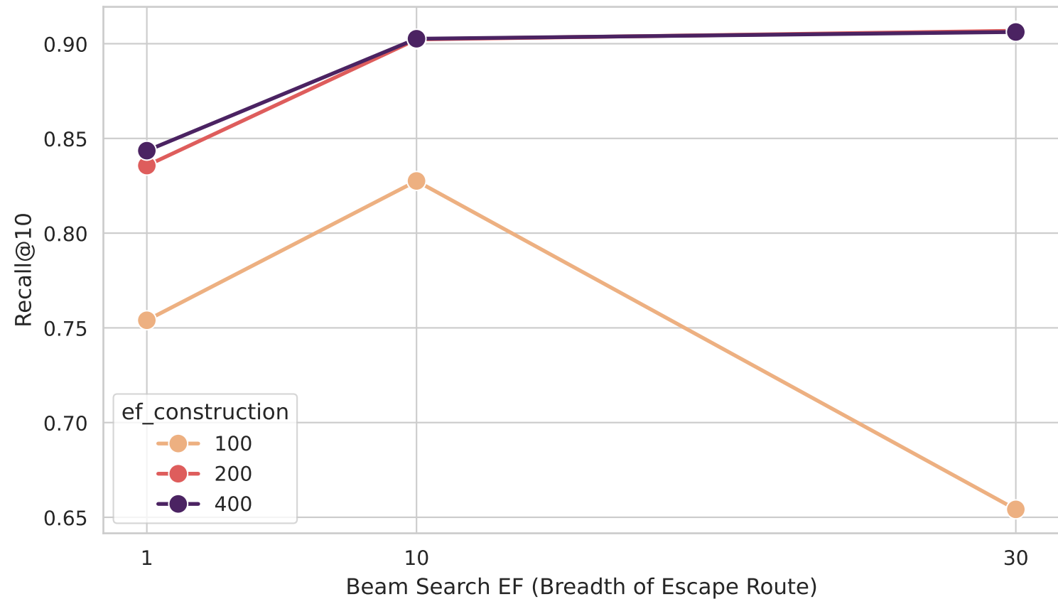
Ablation Study: Beam Search Width vs. Recall (Batch=50K)
