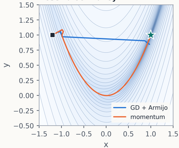
Rosenbrock valley
