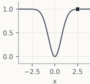
plateau: crawling
