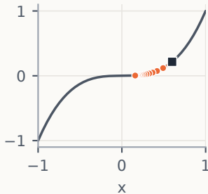
saddle: stuck
