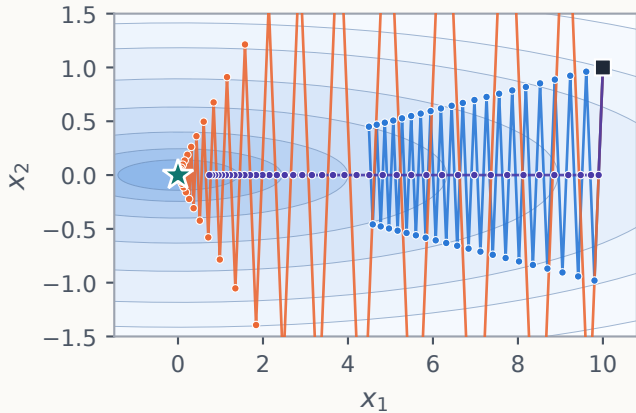
first 40 iterates
