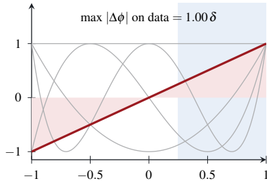
Chebyshev: global support
