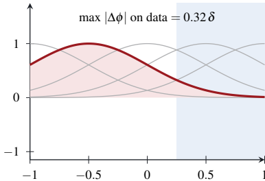
Gaussian RBF: fast decay
