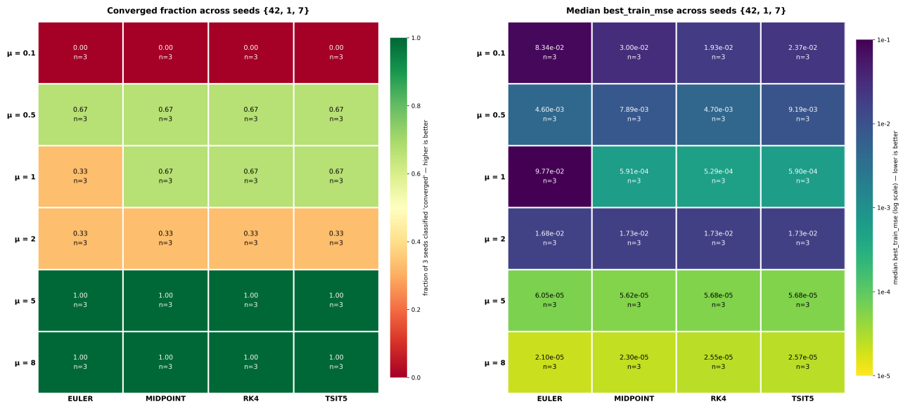
Figure 18. Converged fraction (left) and median training MSE (right) over 3 seeds, all 4 solvers \times 6 \mu (72 cells). The two agree everywhere: low converged-fraction cells are exactly the cells with elevated median error.
