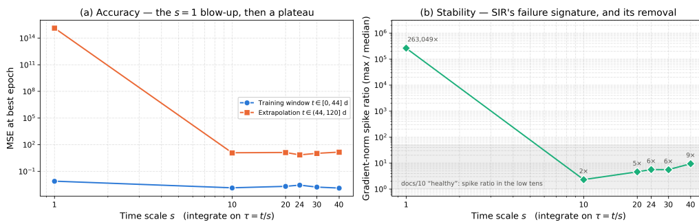
Figure 22. Time-rescaling sweep: accuracy and gradient-spike ratio vs. the rescaling factor.
