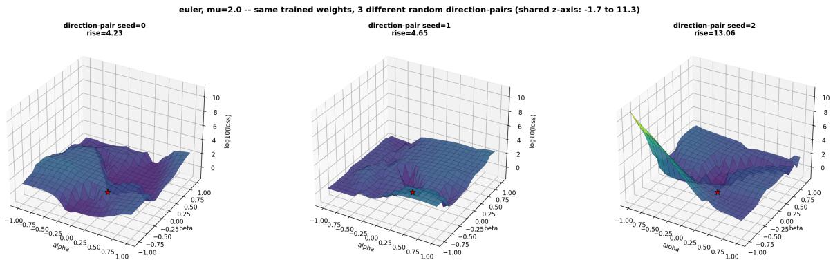
Figure 14. Euler, \mu = 2.0 (trapped): the training-loss surface around the trained weights, viewed under three independent random direction-pairs. The basin near the trained point (the marked star) is broad and shallow in all three views; the third panel's steep spike on the far side is the outlier direction discussed below, not the basin itself.
