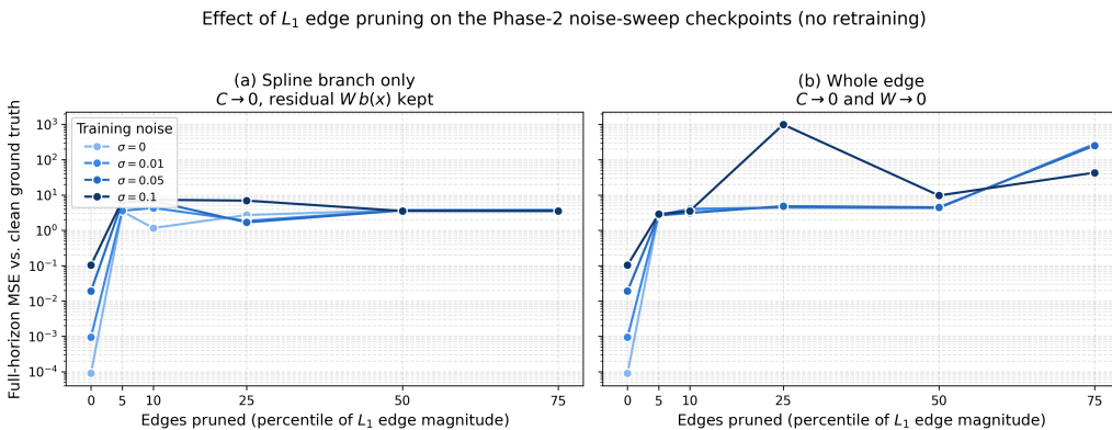
Figure 21. Full-horizon MSE vs. edge-pruning fraction, all four noise levels.
