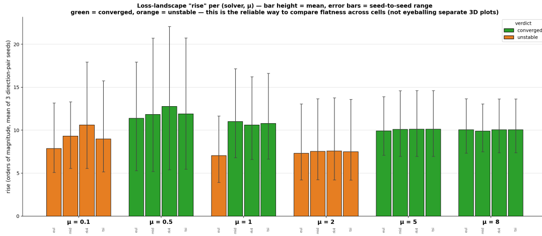
Figure 17. Mean rise per (solver, \mu ), 3-seed average with seed-to-seed range as error bars, colored by verdict.
