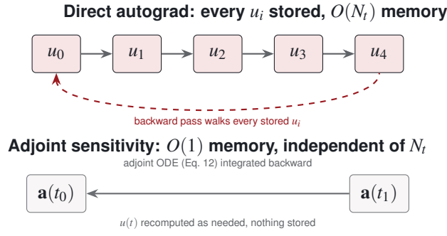
Figure 4. Direct autograd (top) keeps every intermediate state u_i in memory so the backward pass can reuse it, giving O(N_t) memory. Adjoint sensitivity (bottom) instead solves the backward-time equation of Equation 12, recomputing u(t) as needed rather than storing it, giving O(1) memory regardless of N_t .
