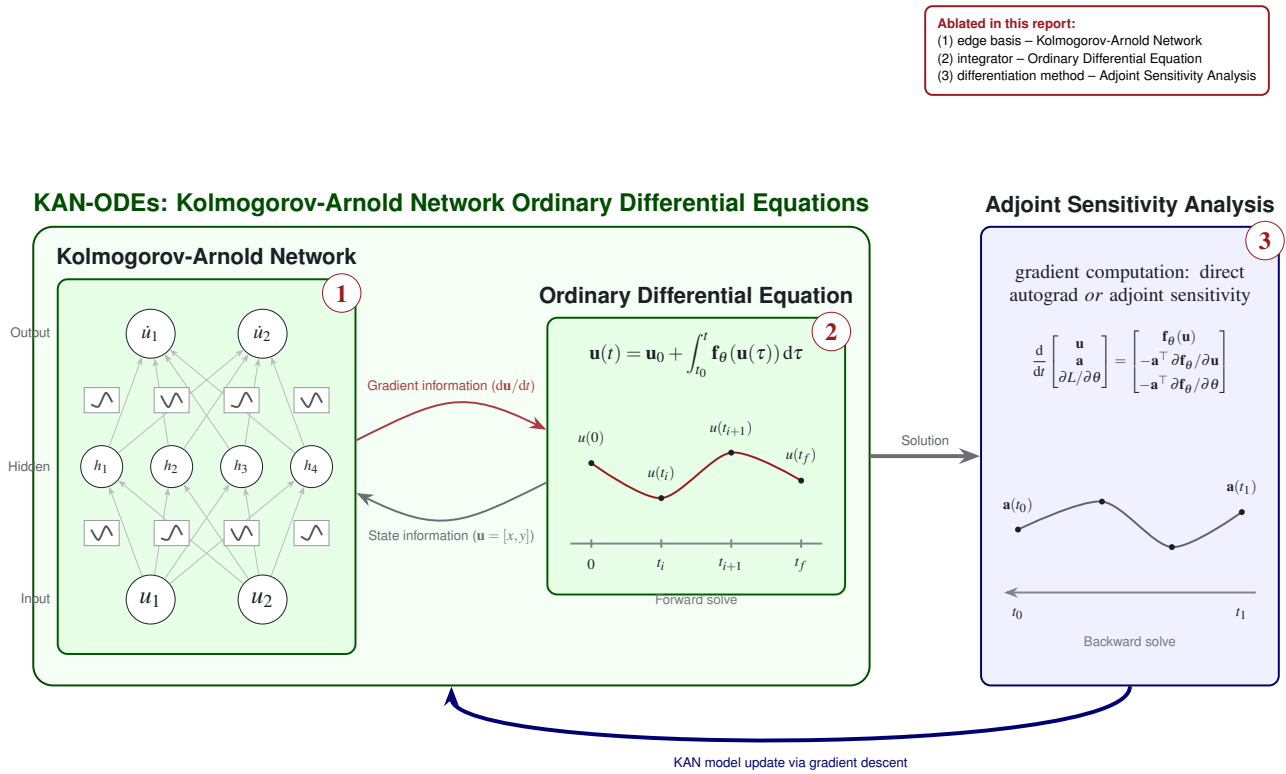
Figure 1. The KAN-ODE training loop, redrawn in the style of the base paper’s own architecture figure [5]. The legend at top right lists this report’s three ablated components and which block of the diagram each corresponds to.
