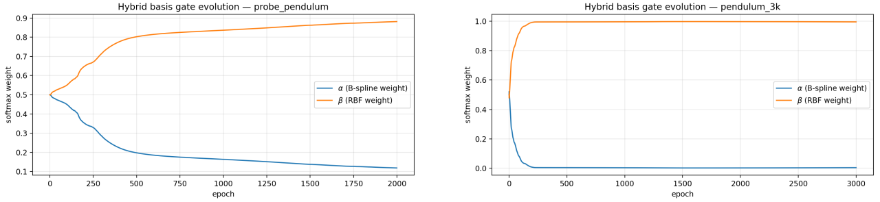
Figure 9. Left: the 2000-epoch probe run’s gate trace, showing the slow drift toward RBF that motivated the gate-learning-rate fix. Right: the gate trace for the 3000-epoch pre-overfitting-optimum run discussed below, settling to \beta \approx 0.996 .
