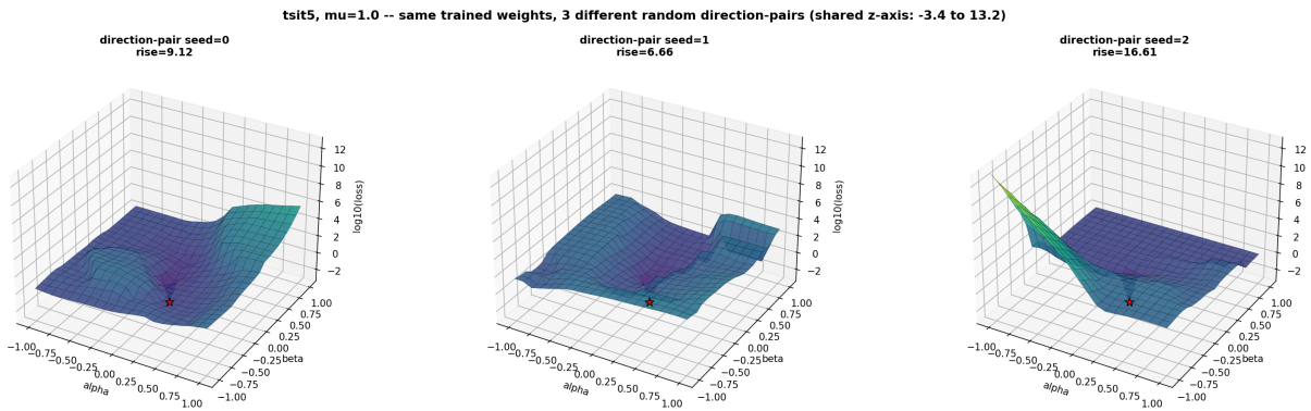
Figure 16. Tsit5, \mu = 1.0 (converged): the basin around the trained point is visibly narrower and drops noticeably lower, in every one of the three direction-pairs, than either trapped case above.
