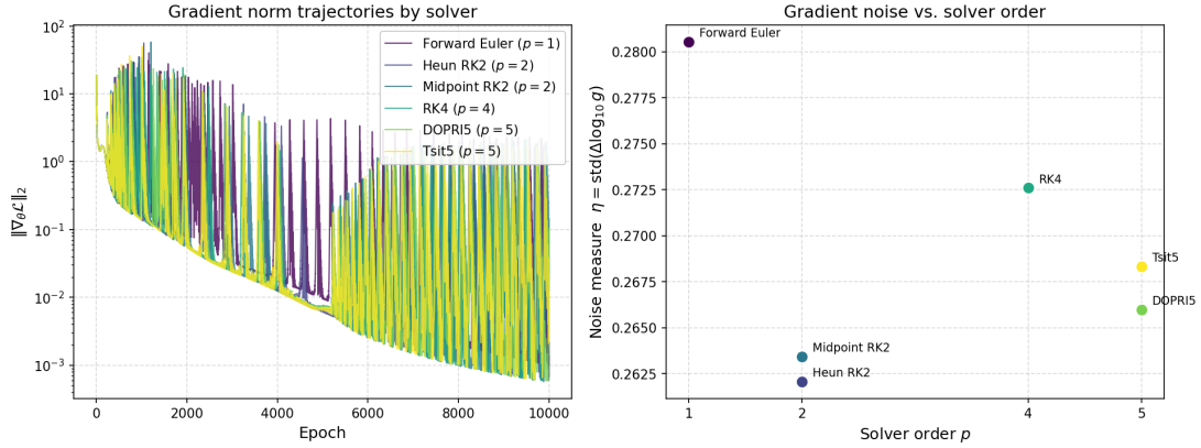
Figure 6. Gradient-norm traces, all six solvers: large sustained spike bursts (one to two orders of magnitude above the local median) dominate every trace, including Tsit5, independent of solver order.
