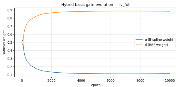
Figure 8. Learned \alpha/\beta gate evolution: Lotka-Volterra settles into a genuine partial blend (left); the pendulum gate converges to \approx 98\% RBF by epoch 250 (right), well before the overfitting onset discussed below.
