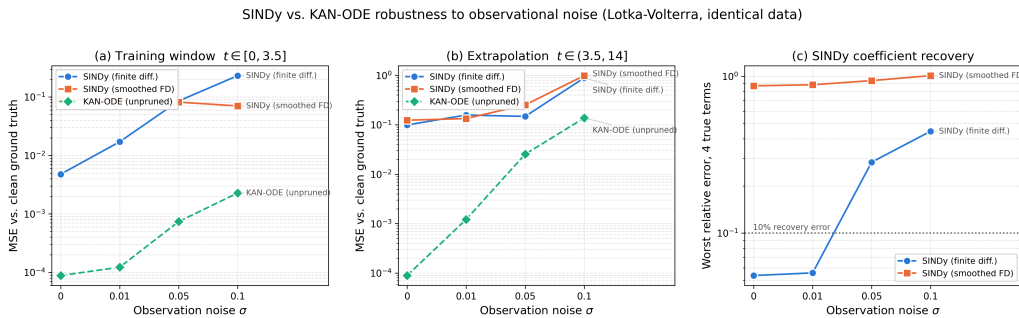
Figure 19. Training and extrapolation MSE vs. noise level, both methods.
