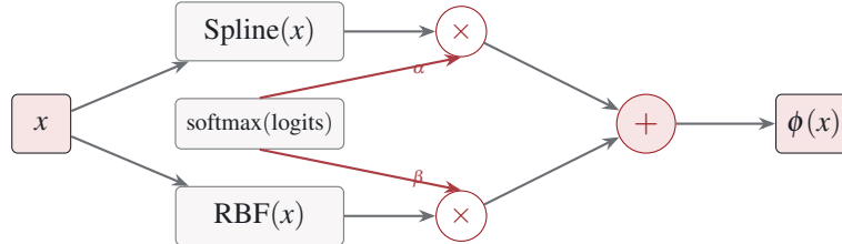
Figure 7. The hybrid-basis edge of Equation 14: every edge evaluates both bases in parallel, and a shared softmax gate produces the scalar weights \alpha, \beta that multiply each basis’s output before they are summed into \phi(x) – the choice of basis is a trained quantity, not a decision fixed at construction time.
