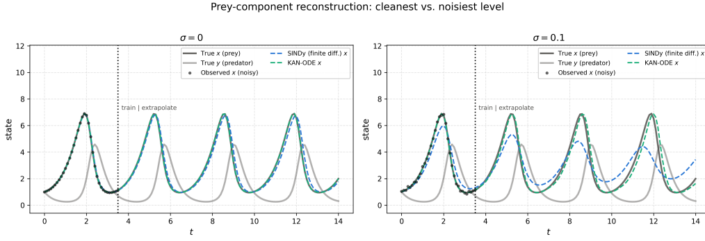
Figure 20. Reconstructed trajectories at \sigma = 0 and \sigma = 0.1 : sparse regression loses amplitude under noise; KAN-ODE keeps amplitude but drifts in phase.
