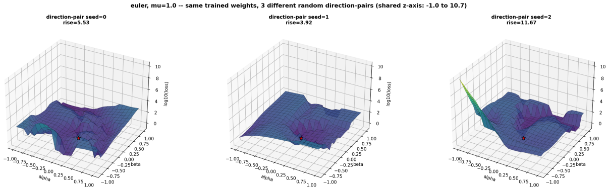
Figure 15. Euler, \mu = 1.0 (also trapped): the same broad, shallow basin shape recurs at a different damping value under the same solver.
