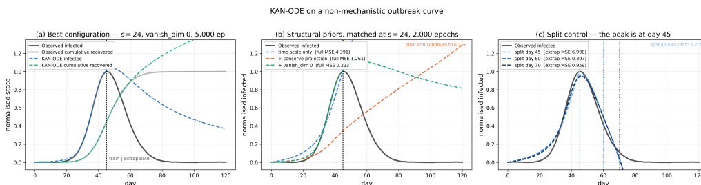
Figure 44. Outbreak-curve fit: default split (runaway), the vanishing-field-gate arm, and the fifteen-day-later split control.
