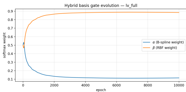
Figure 29. Learned \alpha/\beta gate evolution: Lotka-Volterra settles into a genuine partial blend (left); the pendulum gate reaches \approx 99.5\% RBF by epoch 250 and ends at 98% (right); it settles well before the overfitting onset discussed below.
