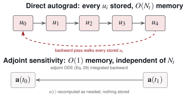
Figure 7. Direct autograd (top) keeps every intermediate state u_i in memory so the backward pass can reuse it, giving O(N_t) memory. Adjoint sensitivity (bottom) instead solves the backward-time equation of Equation 29, recomputing u(t) as needed rather than storing it, giving O(1) memory regardless of N_t .
