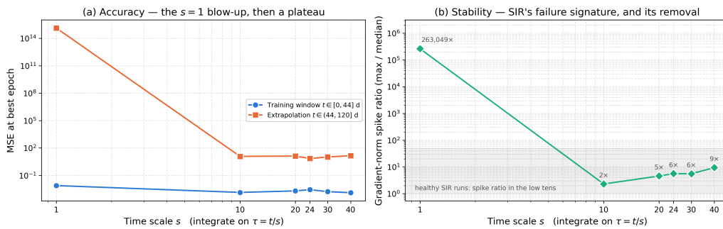
Figure 23. Time-rescaling sweep: accuracy and gradient-spike ratio vs. the rescaling factor.
