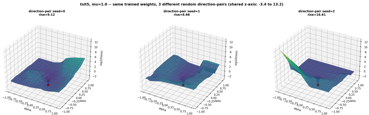
Figure 17. Tsit5, \mu = 1.0 (converged): the basin around the trained point is visibly narrower and drops noticeably lower, in every one of the three direction-pairs, than either trapped case above.
