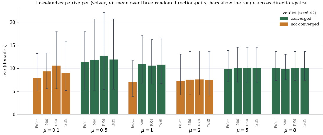
Figure 18. Mean rise per (solver, \mu ) over three random direction-pairs, with the range across direction-pairs as error bars, colored by the seed-42 verdict.
