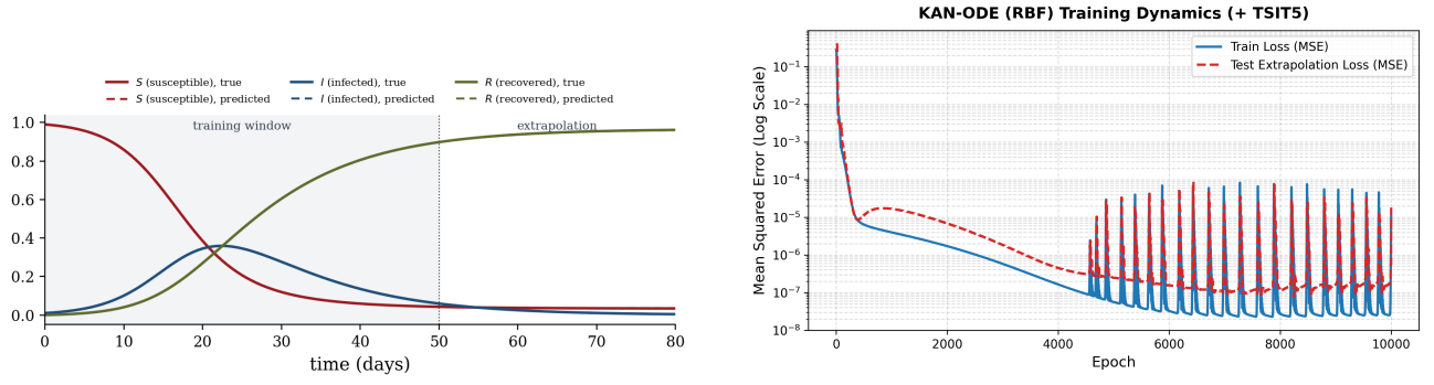
Figure 6. SIR with all three fixes (right-hand column of Table 11). Left: the predicted S , I , R (dashed) lie on top of the true curves (solid) over the whole horizon, including the end of the outbreak after day 50. Right: training and full-horizon loss curves, with no gradient overflow.
