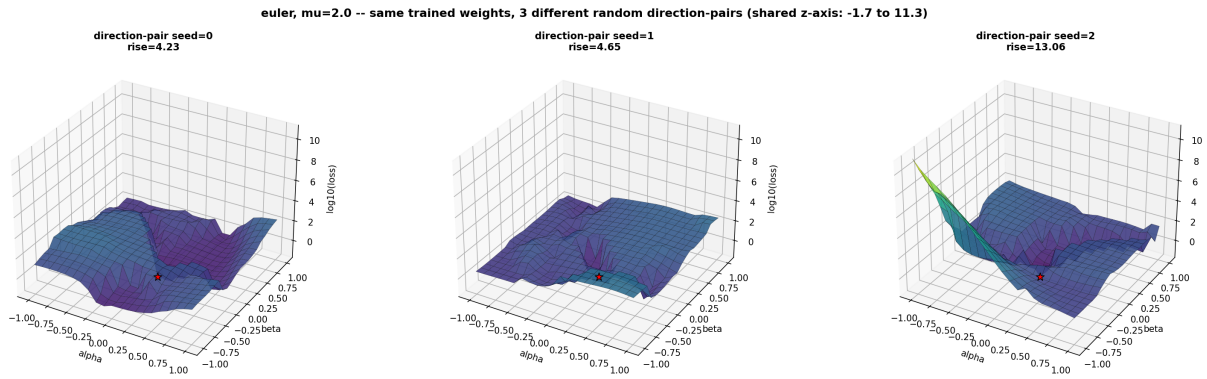
Figure 15. Euler, \mu = 2.0 (trapped): the training-loss surface around the trained weights, viewed under three independent random direction-pairs. The basin near the trained point (the marked star) is broad and shallow in all three views; the third panel's steep spike on the far side is the outlier direction discussed below, not the basin itself.
