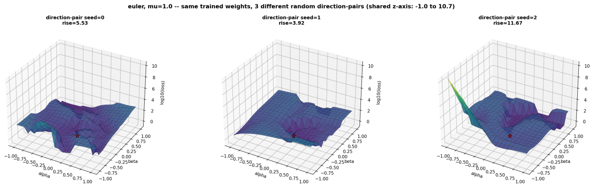
Figure 16. Euler, \mu = 1.0 (also trapped): the same broad, shallow basin shape recurs at a different damping value under the same solver.
