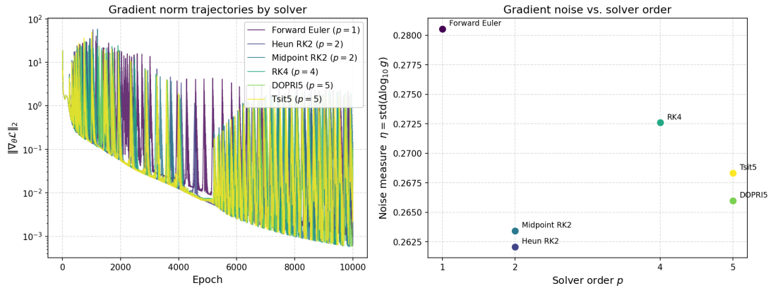
Figure 9. Gradient-norm traces, all six solvers: large sustained spike bursts (one to two orders of magnitude above the local median) dominate every trace, including Tsit5, independent of solver order.
