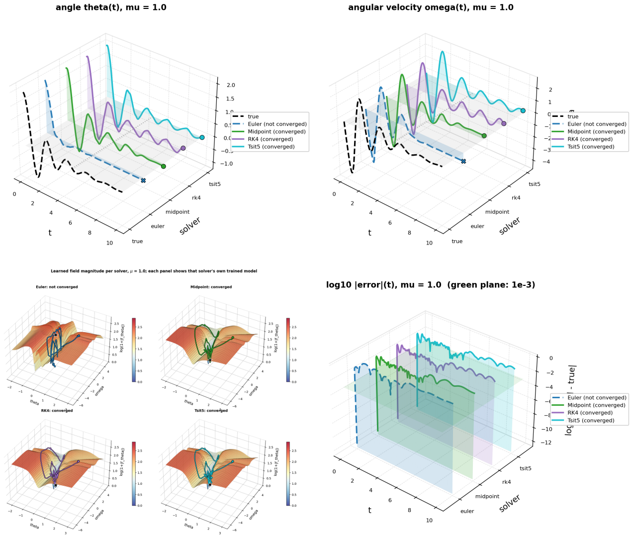
Figure 26. \mu = 1.0 , all four solvers (seed 42), in the same layout. Only Euler's predicted angle departs visibly from the true one; the other three track it closely.
