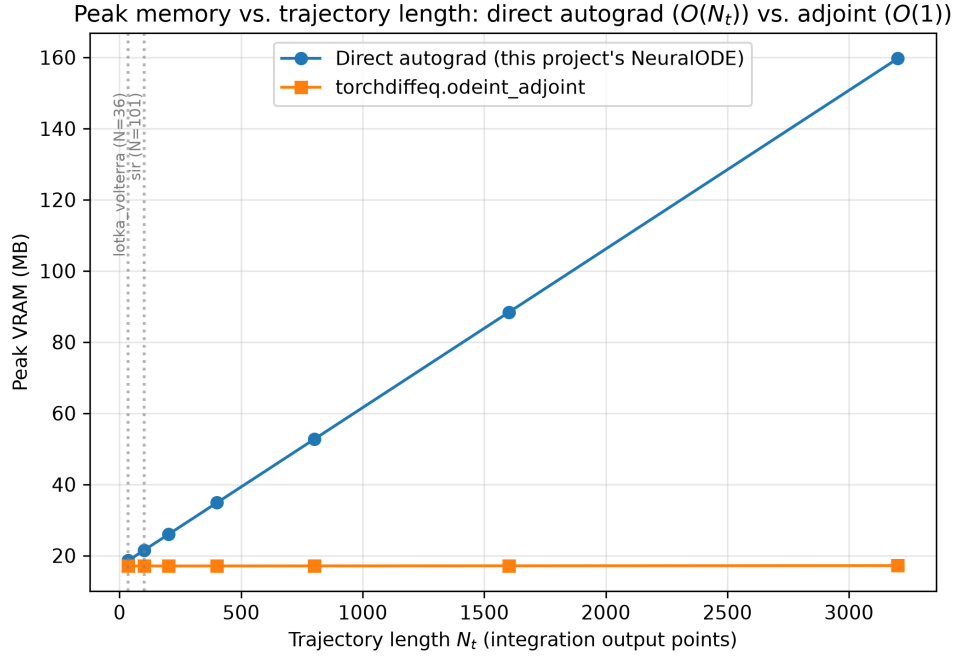
Figure 8. Peak memory vs. trajectory length N_t \in \{36, \dots, 3201\} : direct autograd grows linearly ( \approx 0.045 MB per output point); adjoint stays flat (0.7% increase over an 89\times length increase).
