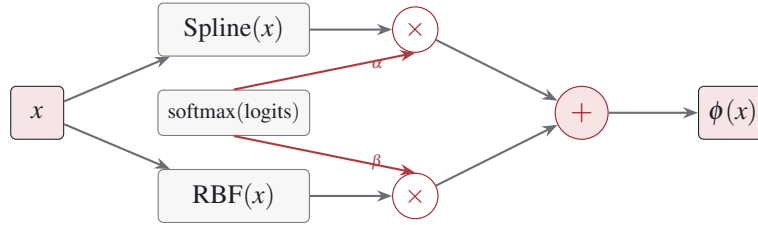
Figure 10. The hybrid-basis edge of Equation 31: every edge evaluates both bases in parallel, and a shared softmax gate produces the scalar weights \alpha, \beta that multiply each basis’s output before they are summed into \phi(x) – the choice of basis is a trained quantity, not a decision fixed at construction time.
