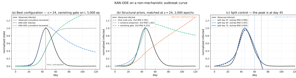
Figure 24. KAN-ODE on the synthetic, non-mechanistic outbreak curve. Left: the best configuration ( s = 24 , vanishing gate on I , 5,000 epochs). Middle: the structural priors compared at s = 24 and 2,000 epochs. Right: moving the train/test split from day 45 to day 60 or 70.
