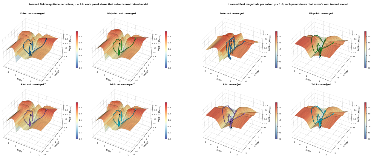
Figure 14. Learned vector-field landscape |f_\theta(\theta, \omega)| , per solver’s own trained model. Left ( \mu = 2.0 ): every solver’s true equilibrium (star) sits partway up a slope, while a separate, lower point nearby is where each trajectory actually settles. Right ( \mu = 1.0 ): Euler’s star sits high on a ridge, well apart from where its trajectory spirals down and rests; for the other three solvers, star and resting point coincide at the valley floor.
