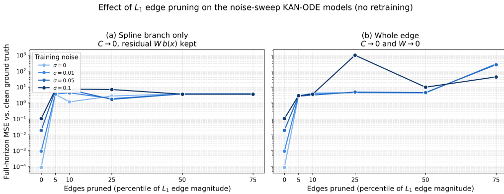
Figure 22. Full-horizon MSE vs. edge-pruning fraction for the noise-sweep KAN-ODE models, all four noise levels, pruned without retraining.
