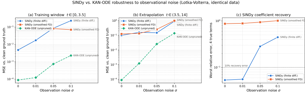
Figure 20. Training and extrapolation MSE vs. noise level, both methods.
