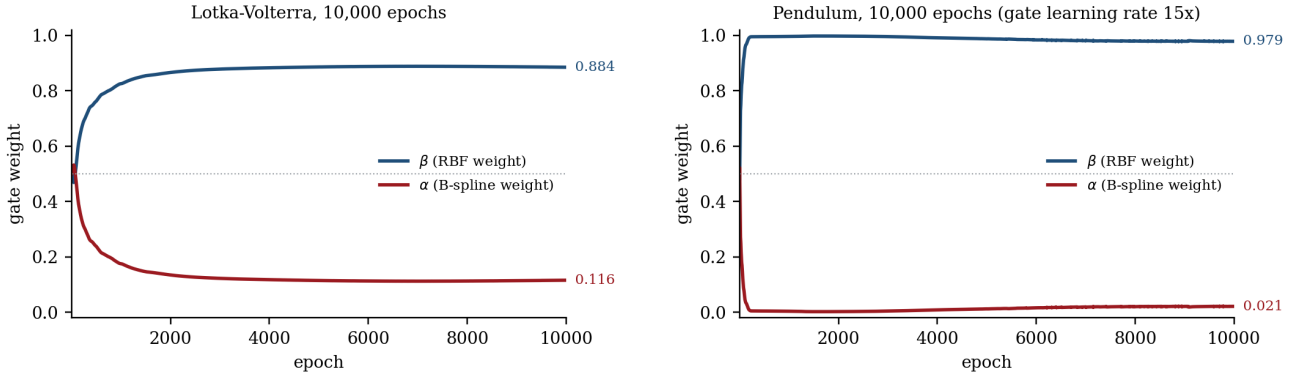
Figure 11. Learned gate weights over training. Left: Lotka-Volterra settles at \alpha = 0.116 , \beta = 0.884 . Right: the pendulum gate reaches \beta = 0.995 by epoch 250 and peaks at 0.998 near epoch 1600, then drifts slowly back to 0.979 over the rest of the run, the same period in which the model overfits (discussed below).
