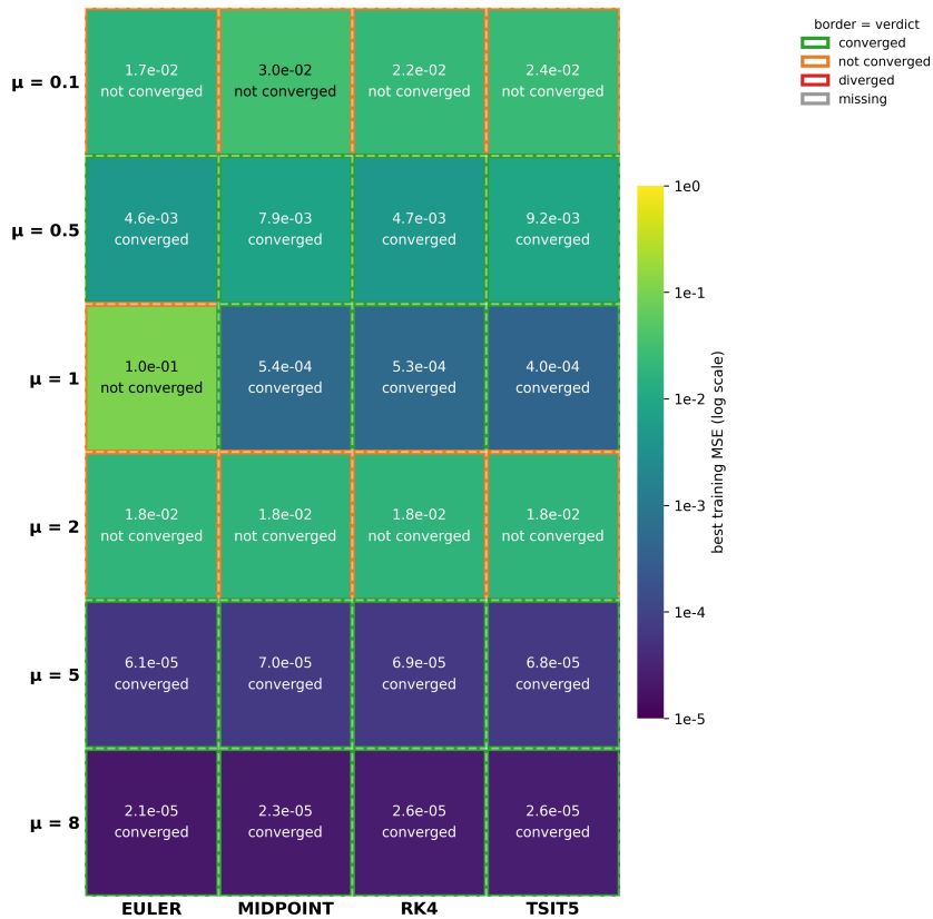
Figure 13. Verdict map of the 24-cell single-seed sweep ( \Delta t = 0.05 , two substeps). Each cell shows its best training MSE and verdict under the rule above; the border color repeats the verdict.
