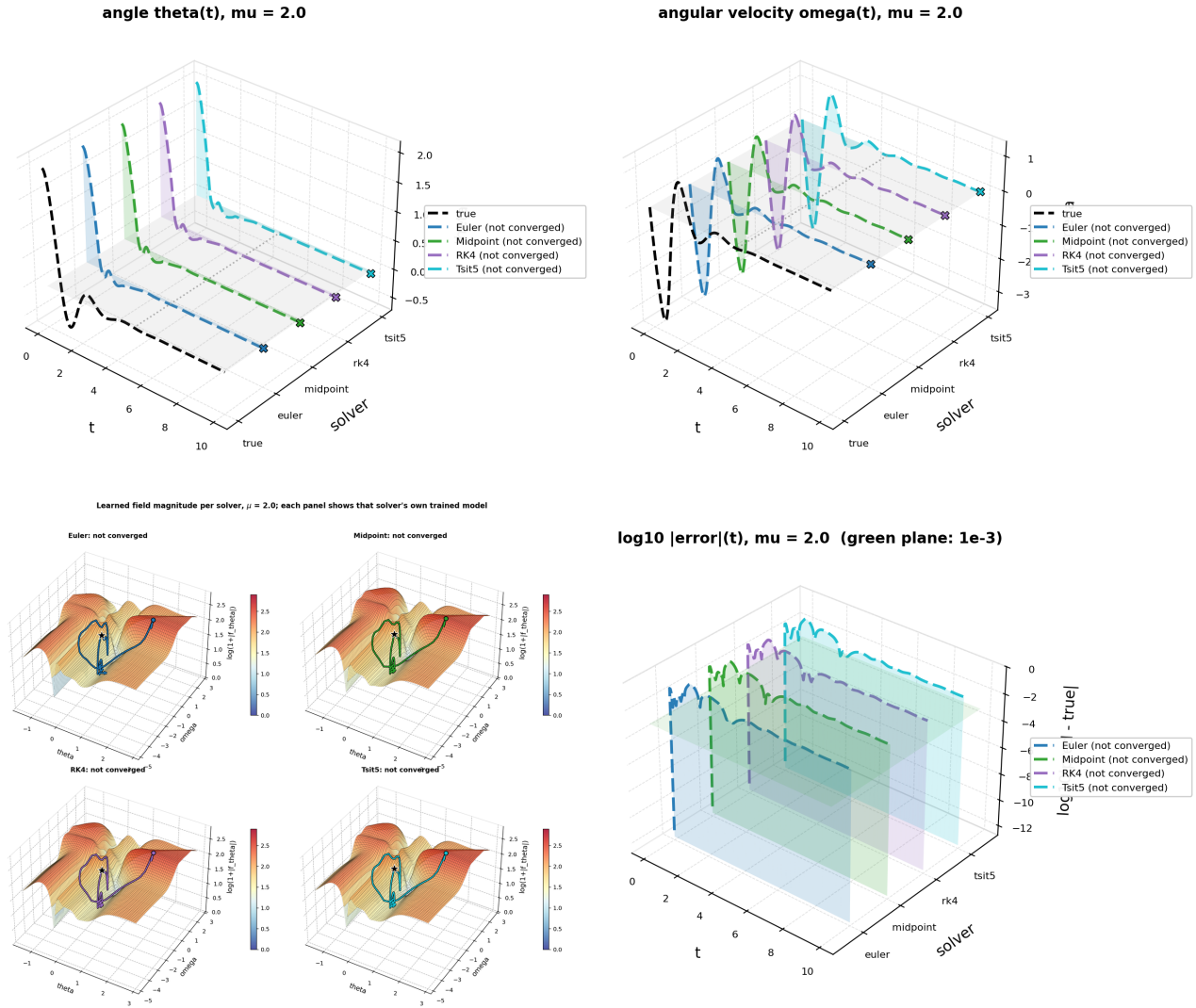
Figure 25. \mu = 2.0 , all four solvers (seed 42). Every model settles onto the same wrong trajectory, which ends at the learned spurious equilibrium of Table 20.
