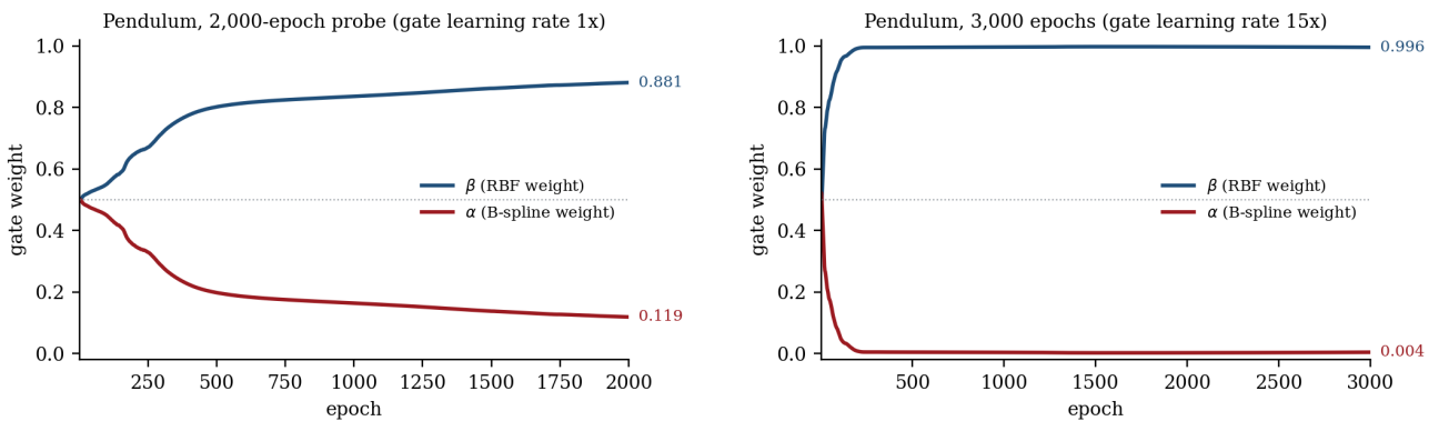
Figure 12. Left: the 2,000-epoch pendulum probe at the base gate learning rate, whose gate drifts toward RBF only slowly ( \beta = 0.881 at the end), which motivated the faster gate rate. Right: the 3,000-epoch pendulum run at the faster gate rate discussed below, settling at \beta = 0.996 .
