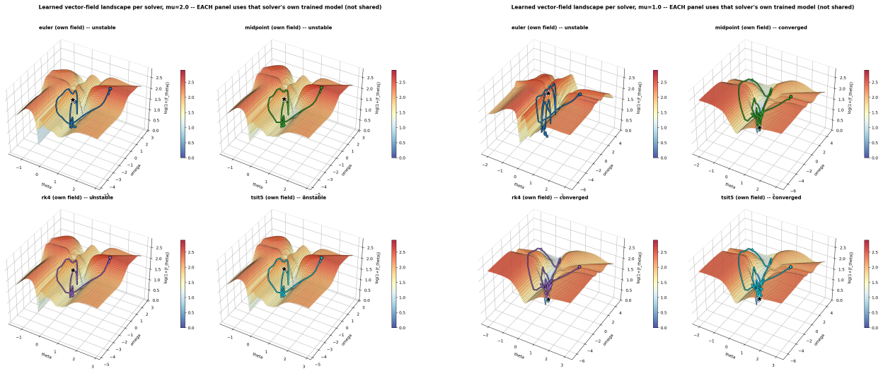
Figure 34. Learned vector-field landscape |f_{\theta}(\theta, \omega)| , per solver's own trained model. Left ( \mu = 2.0 ): every solver's true equilibrium (star) sits partway up a slope, while a separate, lower point nearby is where each trajectory actually settles. Right ( \mu = 1.0 ): Euler's star sits high on a ridge, well apart from where its trajectory spirals down and rests; for the other three solvers, star and resting point coincide at the valley floor.
