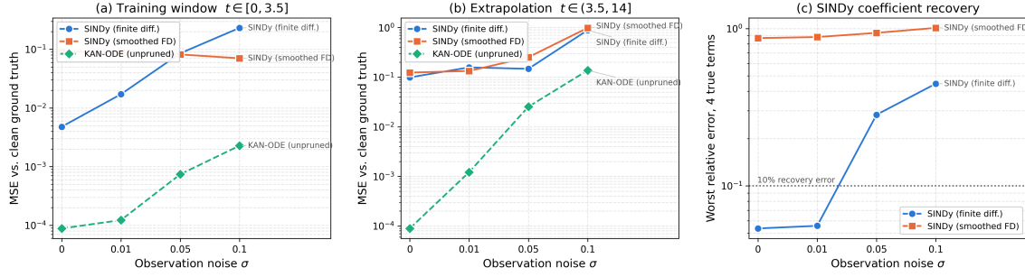
Figure 40: Training and extrapolation MSE vs. noise level, both methods.
