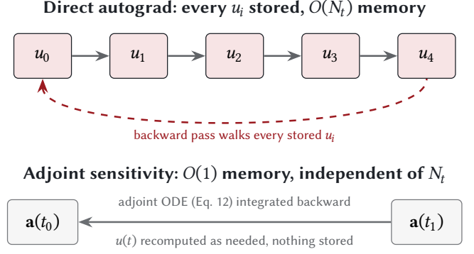
Figure 4: Direct autograd (top) keeps every intermediate state u_i in memory so the backward pass can reuse it, giving O(N_t) memory. Adjoint sensitivity (bottom) instead solves the backward-time equation of Equation 12, recomputing u(t) as needed, giving O(1) memory regardless of N_t .
