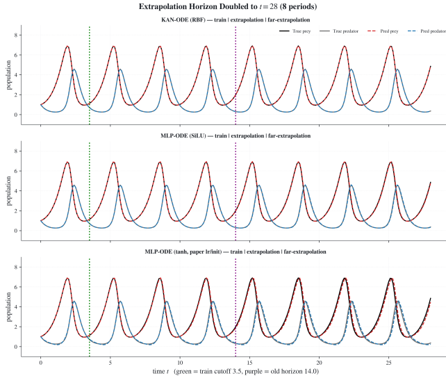
Figure 8: Predicted against true populations out to t = 28 for the three models, with no retraining. KAN-ODE and SiLU-MLP are visually indistinguishable from the truth. The paper’s tanh MLP under its own learning rate and initialization (bottom, fourth column of Table 6) follows the training window and the first periods closely, then runs slightly slow and lags visibly by the far window [14, 28].
