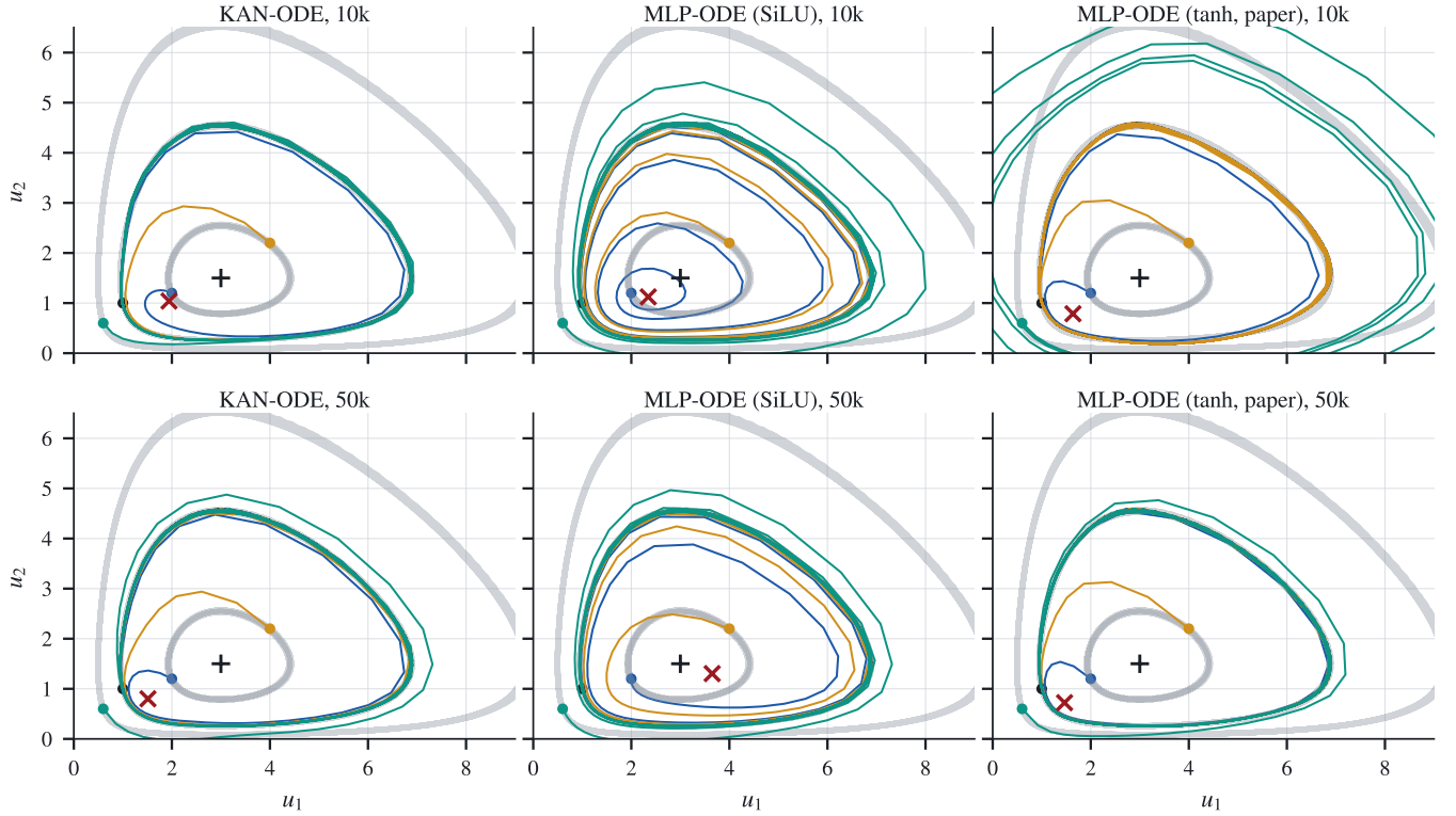
Figure 18: Trajectories of each learned field from four initial conditions (coloured dots) over t \in [0, 40] , against the four corresponding true orbits (grey). Red crosses mark the learned equilibria, black plus signs the true one. Columns: KAN-ODE, SiLU MLP-ODE, and the paper’s tanh MLP-ODE under the paper’s own learning rate and initialization; rows: 10^4 and 5 \times 10^4 epochs. Every learned field attracts all four onto the training orbit except the 10^4 -epoch tanh MLP, under which the trajectory from (0.6, 0.6) diverges.
