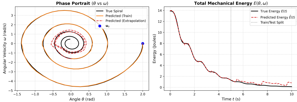
Figure 27: Fixed pendulum ( \mu = 0.5 , t_{\text{train}} = 5 ): phase portrait (left) and total mechanical energy E(\theta, \omega) (right). Inside the training window the predicted energy follows the true curve closely; past the split at t = 5 it stays above the truth and rises on 40 of 200 predicted steps, the under-damping described in the text.
