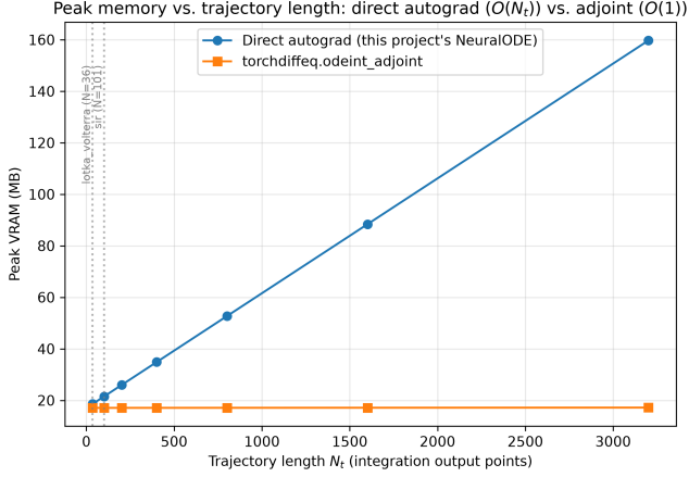
Figure 28: Peak memory vs. trajectory length N_t \in \{36, \dots, 3201\} : direct autograd grows linearly ( \approx 0.045 MB per output point); adjoint stays flat (0.7% increase over an 89 \times length increase).
