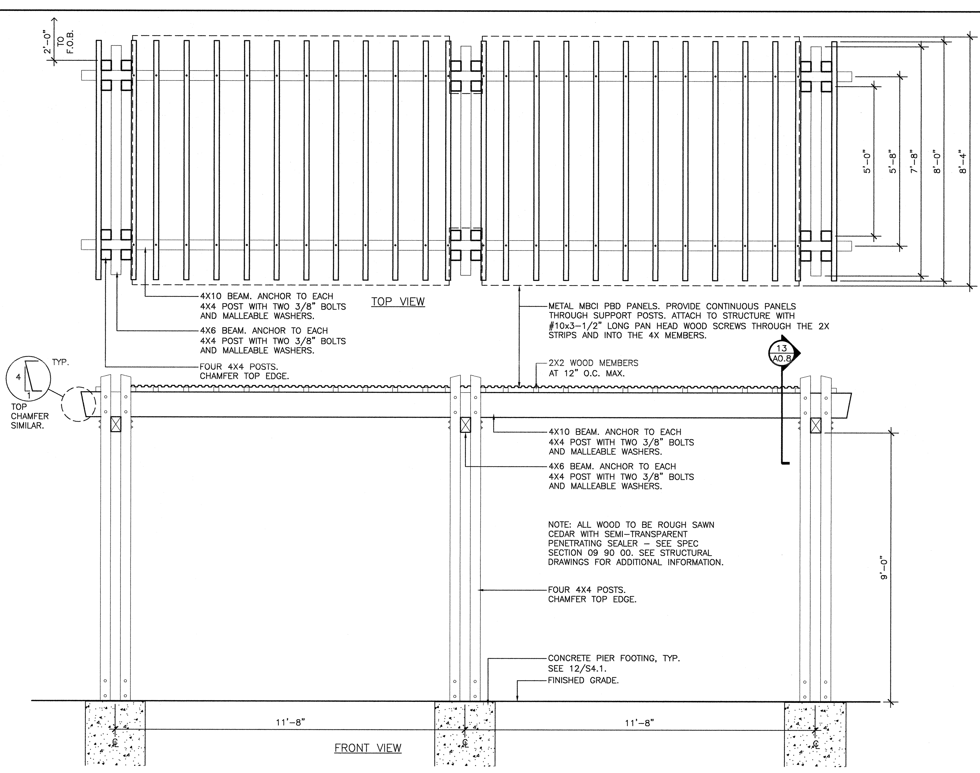
3 PERGOLA— NORTH STAFF ENTRANCE SCALE: 1/2" = 1'-0"
