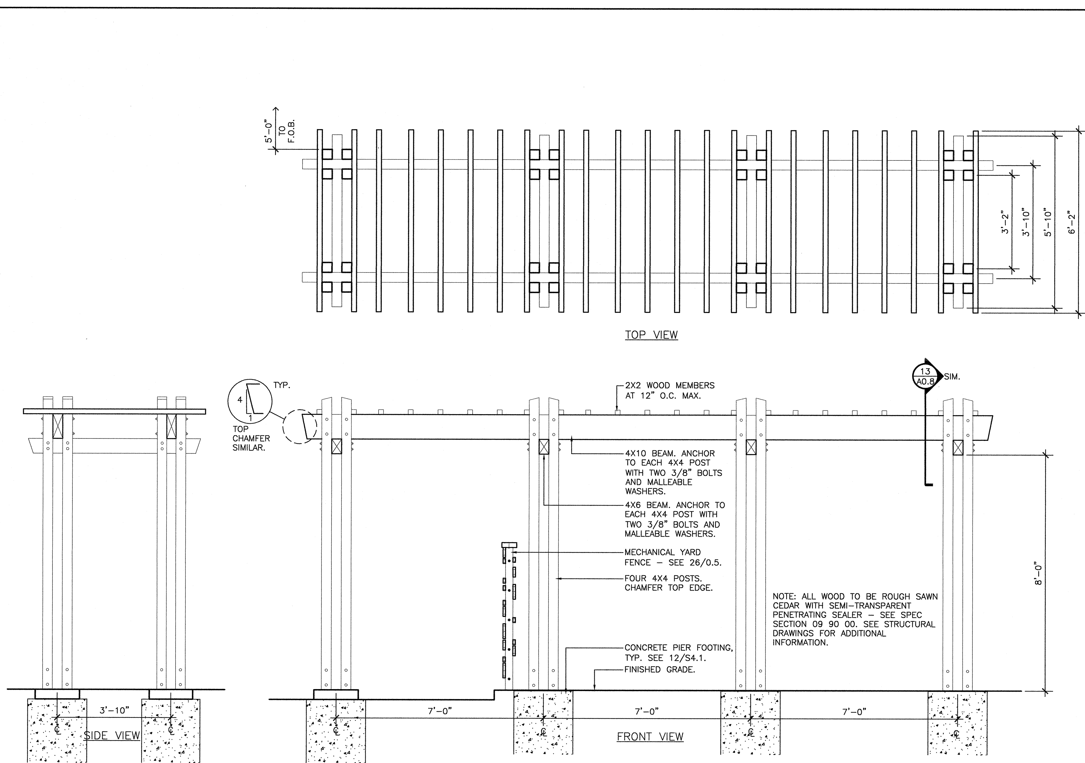
2 PERGOLA— WEST MECH. SERVICE YARD (TYP. OF TWO) SCALE: 1/2" = 1'-0"
