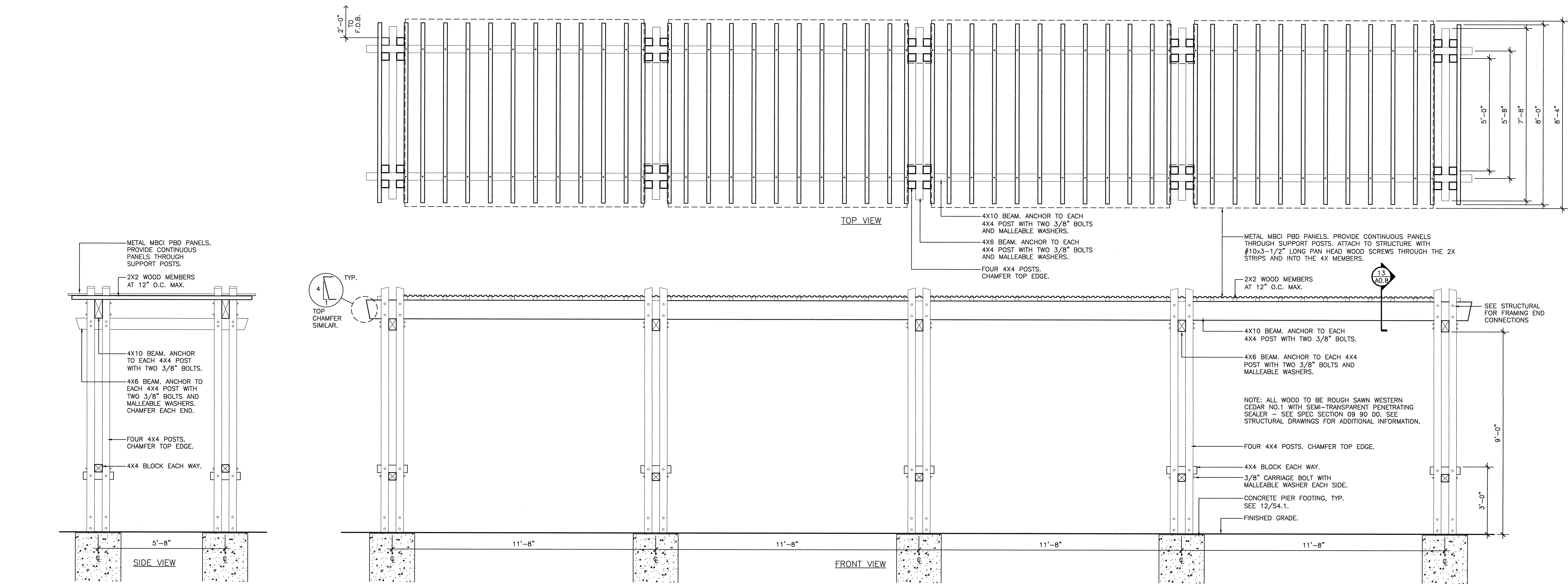
1 PERGOLA— EAST COMMUNITY ROOM SCALE: 1/2" = 1'-0"
