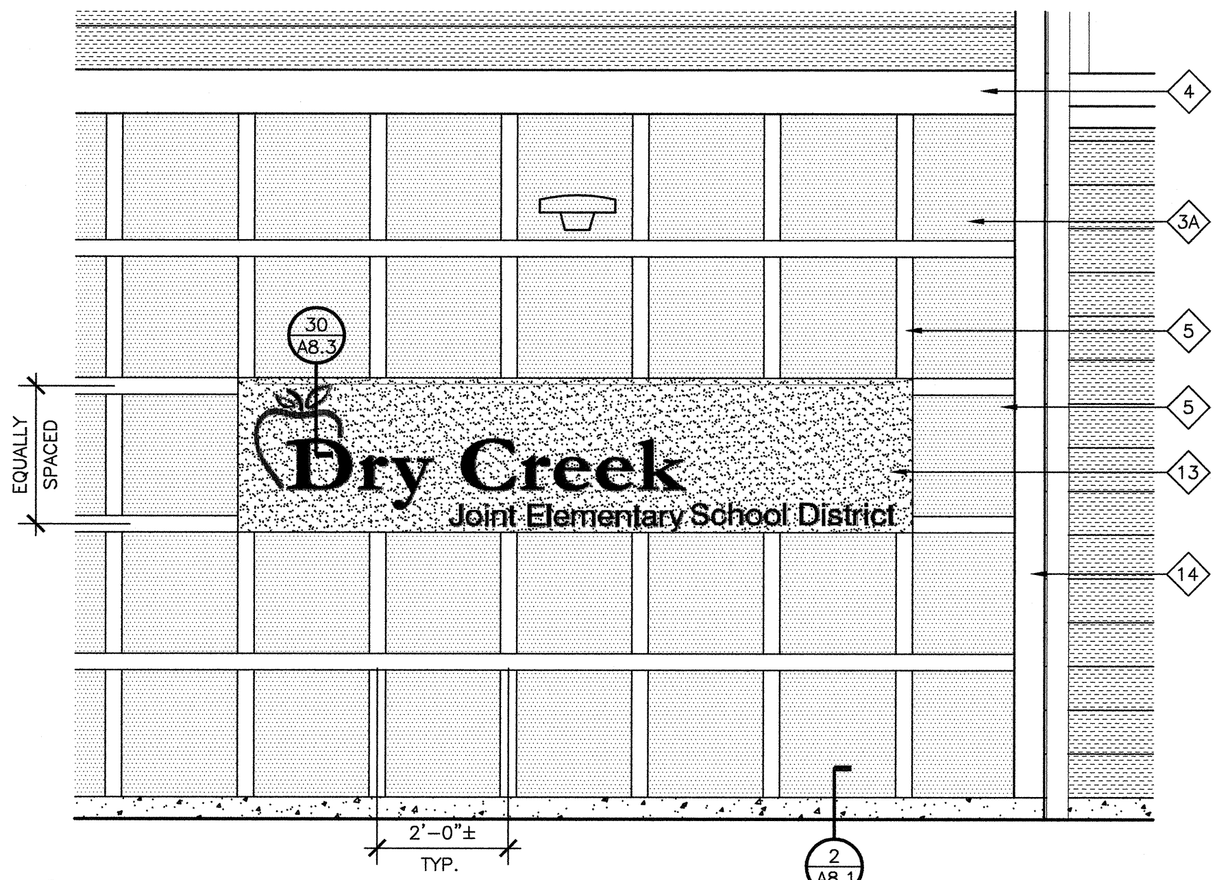
6 Partial Enlarged Elevation
