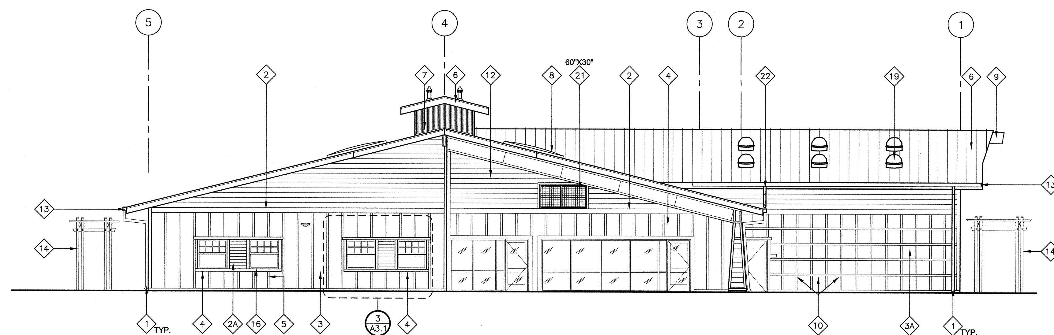
2 South Exterior Elevation SCALE: 1/8" = 1'-0"
