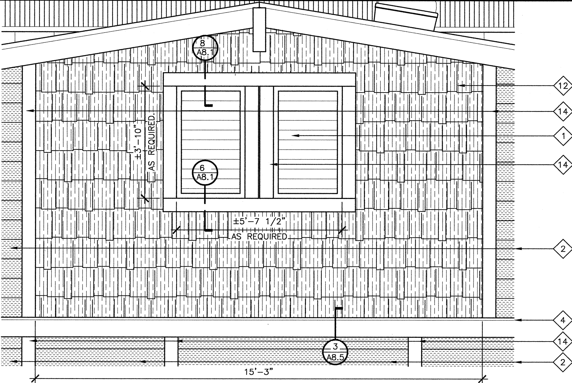
4 Partial Enlarged Elevation
