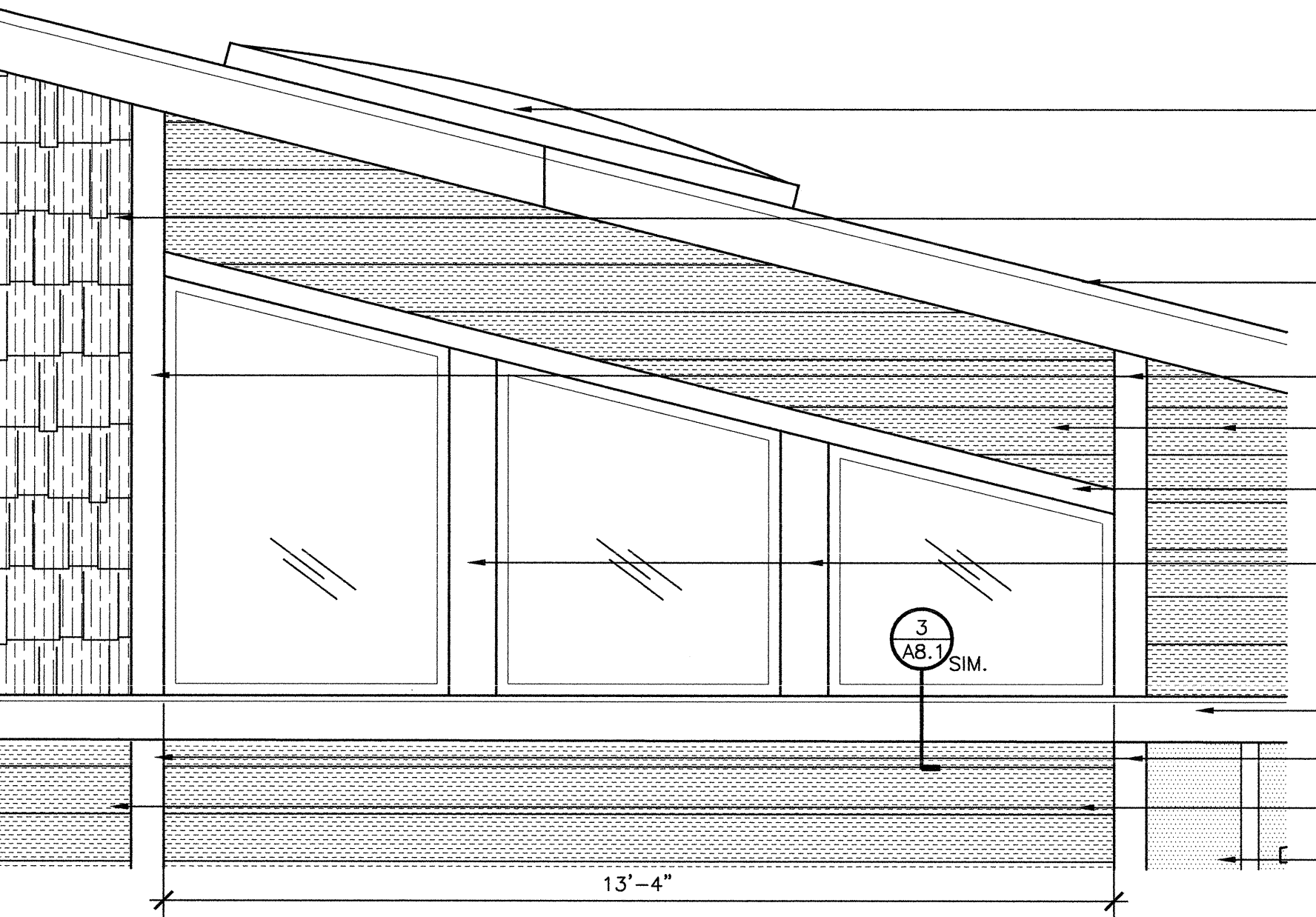
5 Partial Enlarged Elevation
