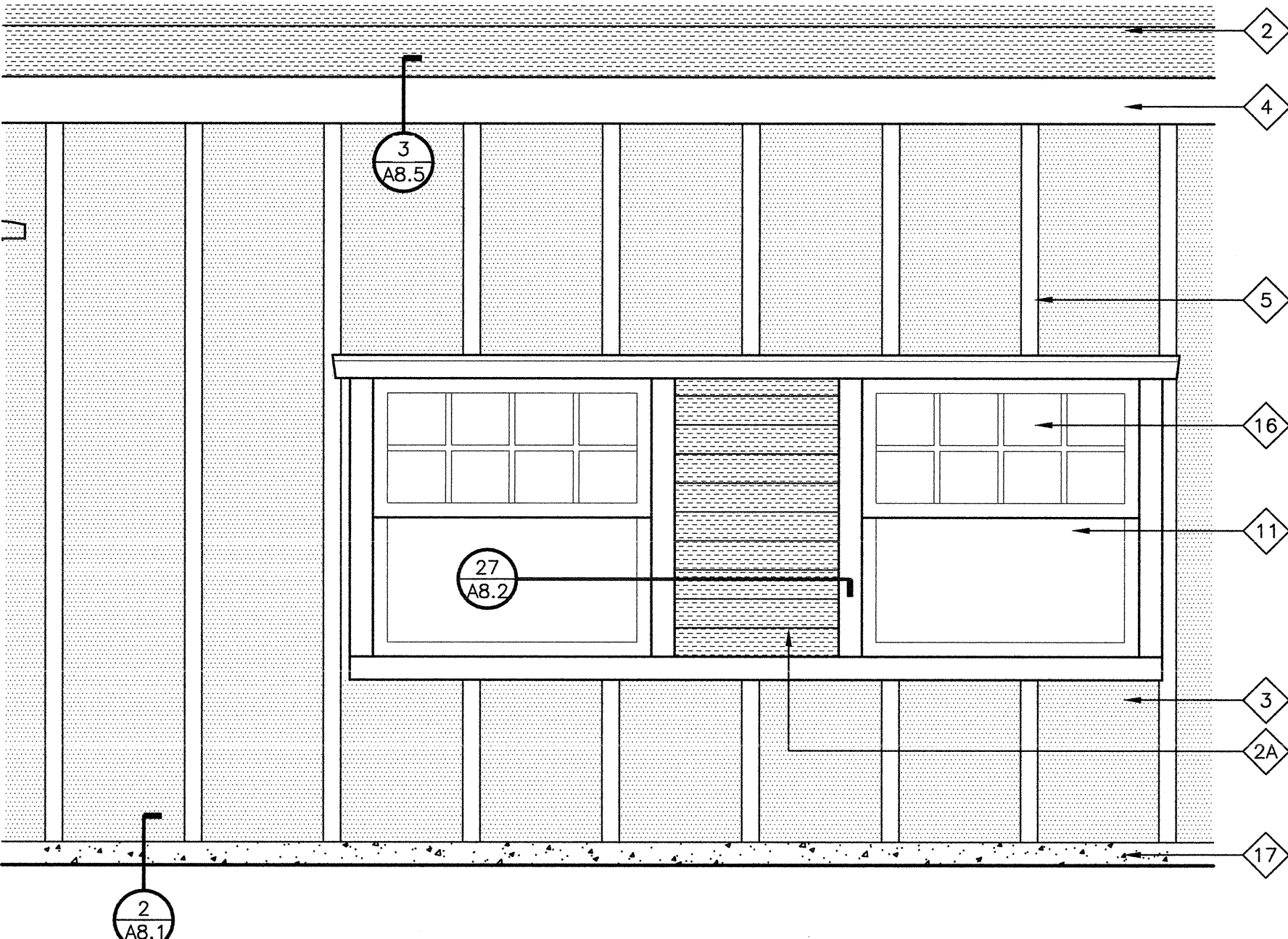
3 Partial Enlarged Elevation
