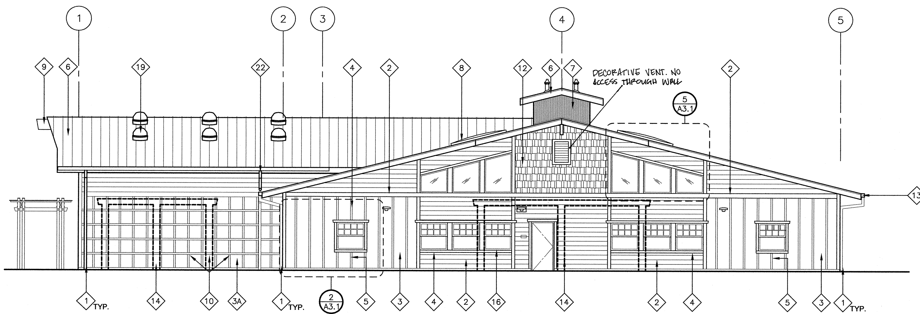
1 North Exterior Elevation SCALE: 1/8" = 1'-0"
