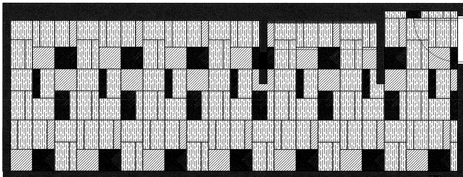
2 Restroom Floor Pattern Plan SCALE: 1/4" = 1'-0"
