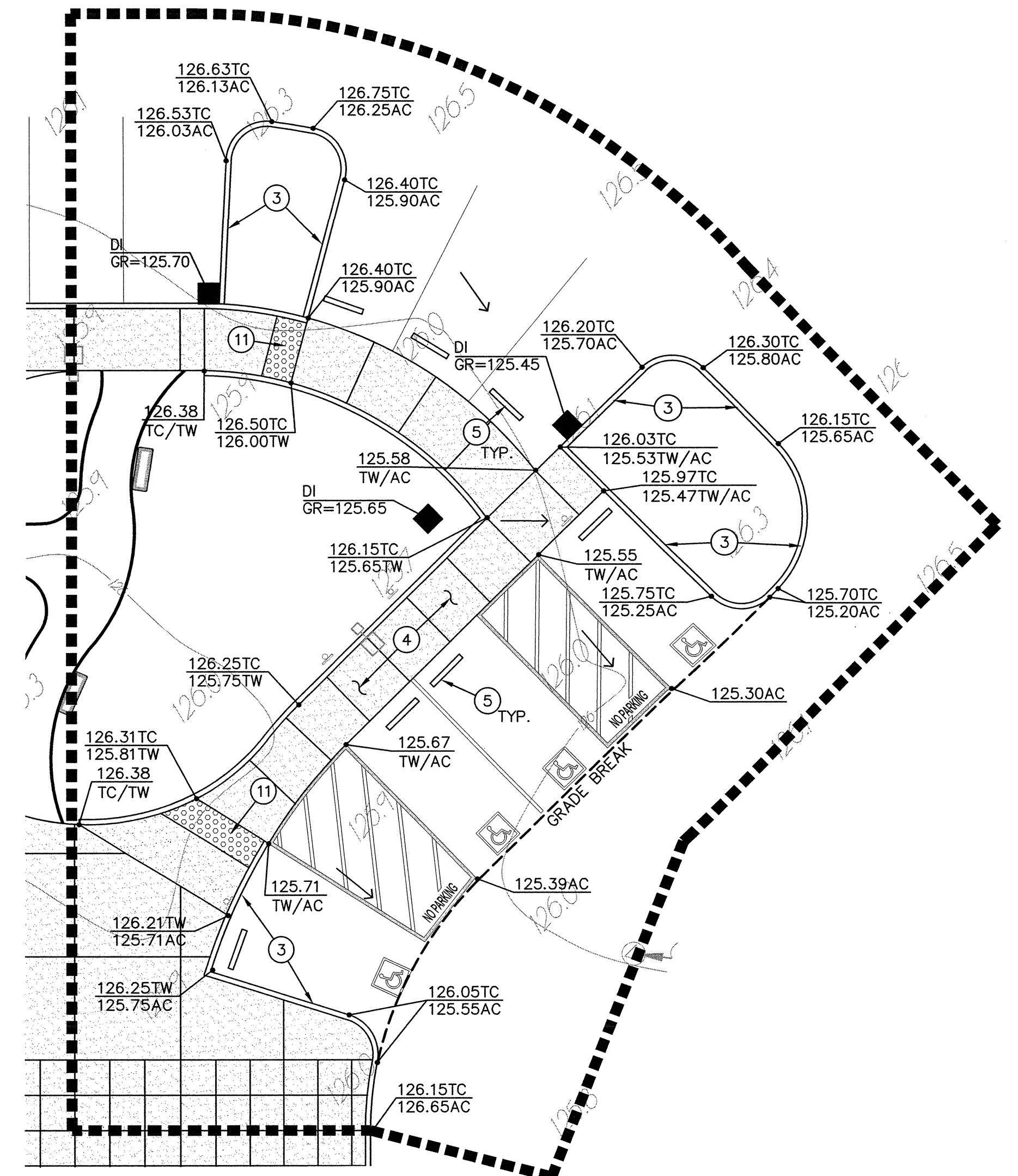
DETAIL "A"
