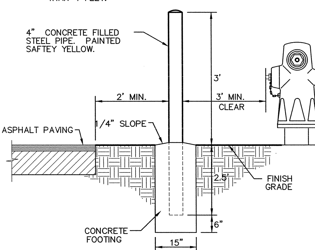
3 C6.1 PIPE BOLLARD NO SCALE
