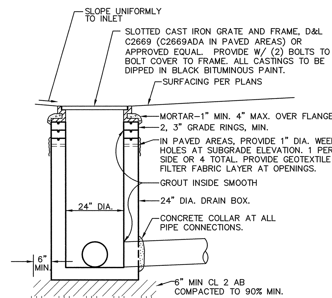
13 C6.1 DROP INLET NO SCALE
