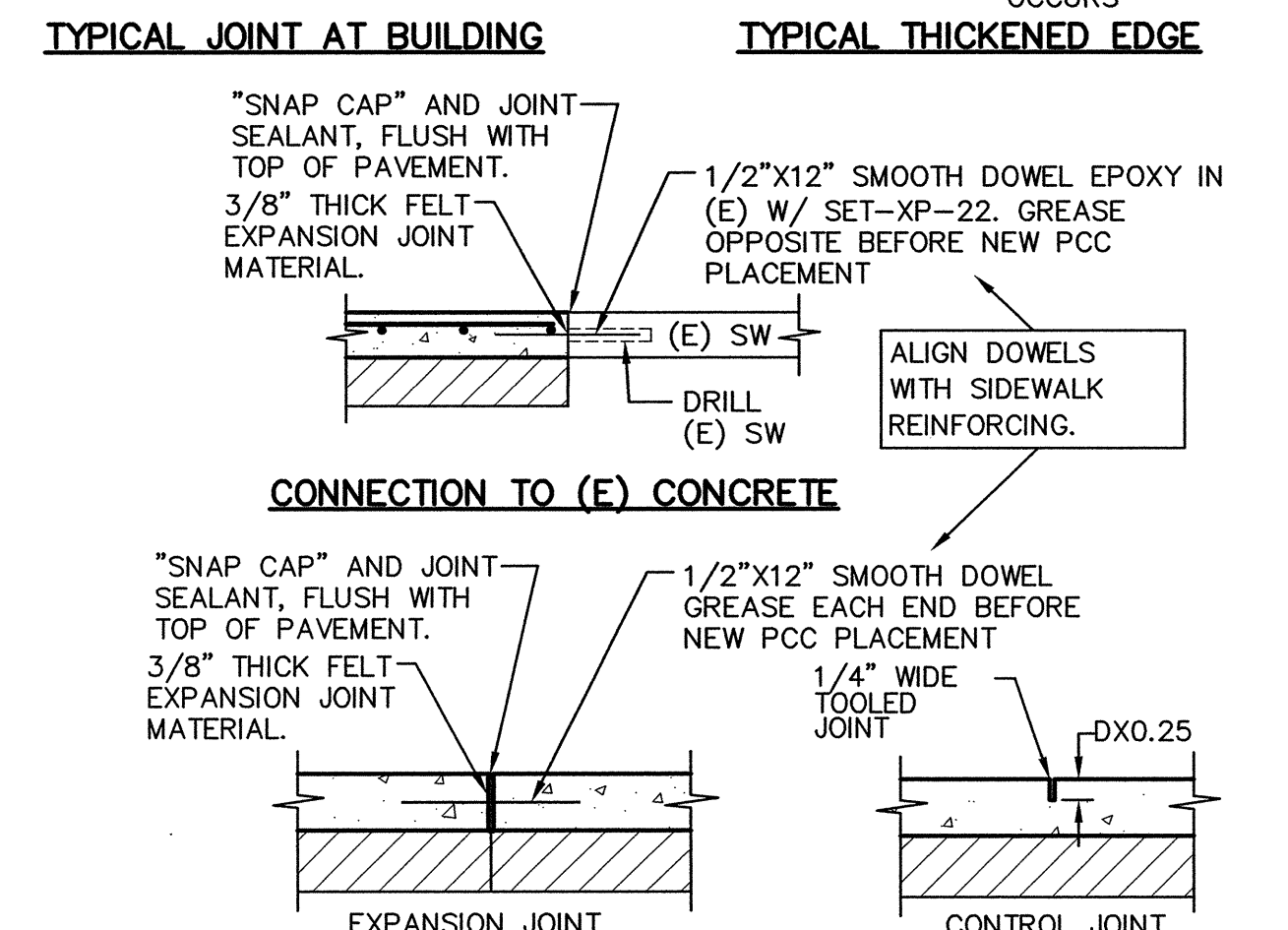
2 C6.1 CONCRETE SIDEWALK NO SCALE
