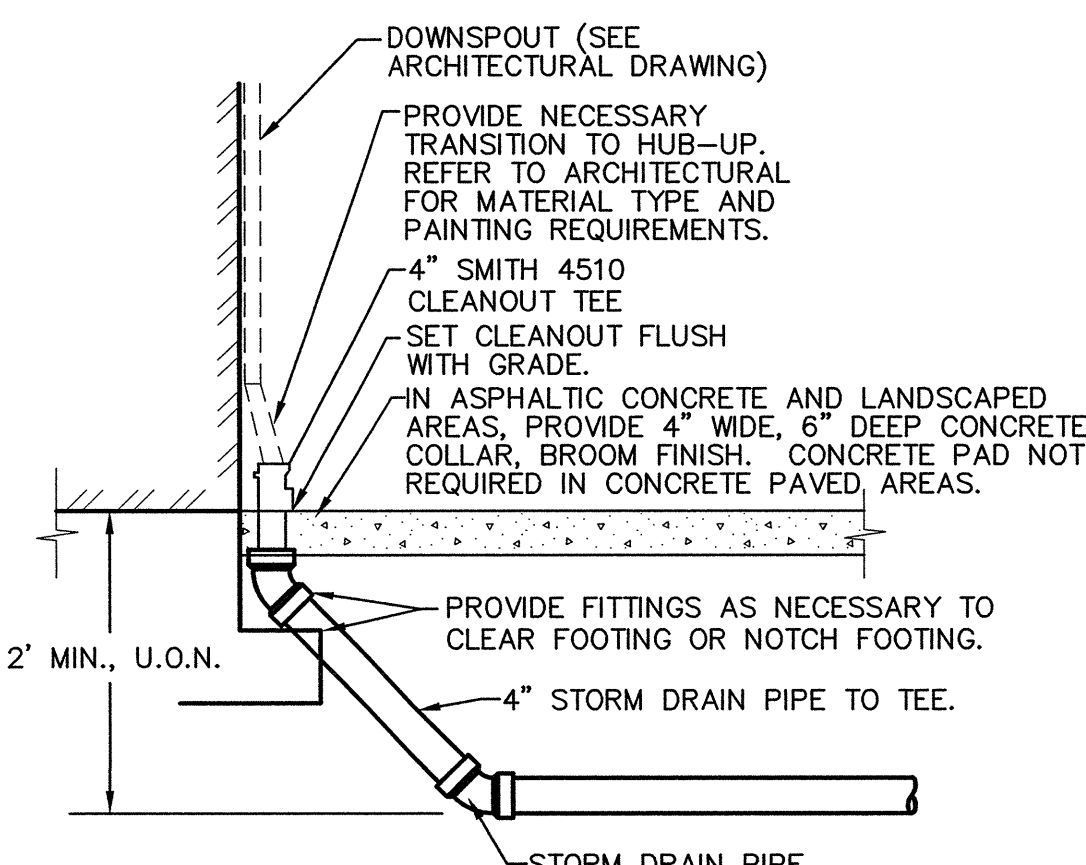
15 C6.1 DOWNSPOUT DETAIL NO SCALE
