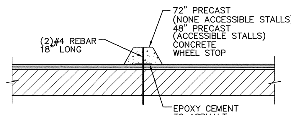
17 C6.1 CONCRETE WHEEL STOP NO SCALE
