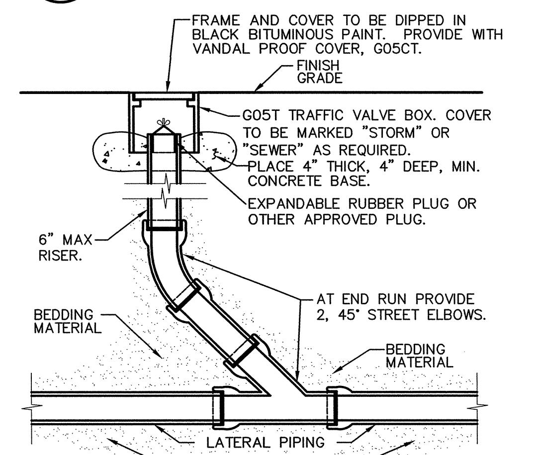
4 C6.1 CLEANOUT NO SCALE
