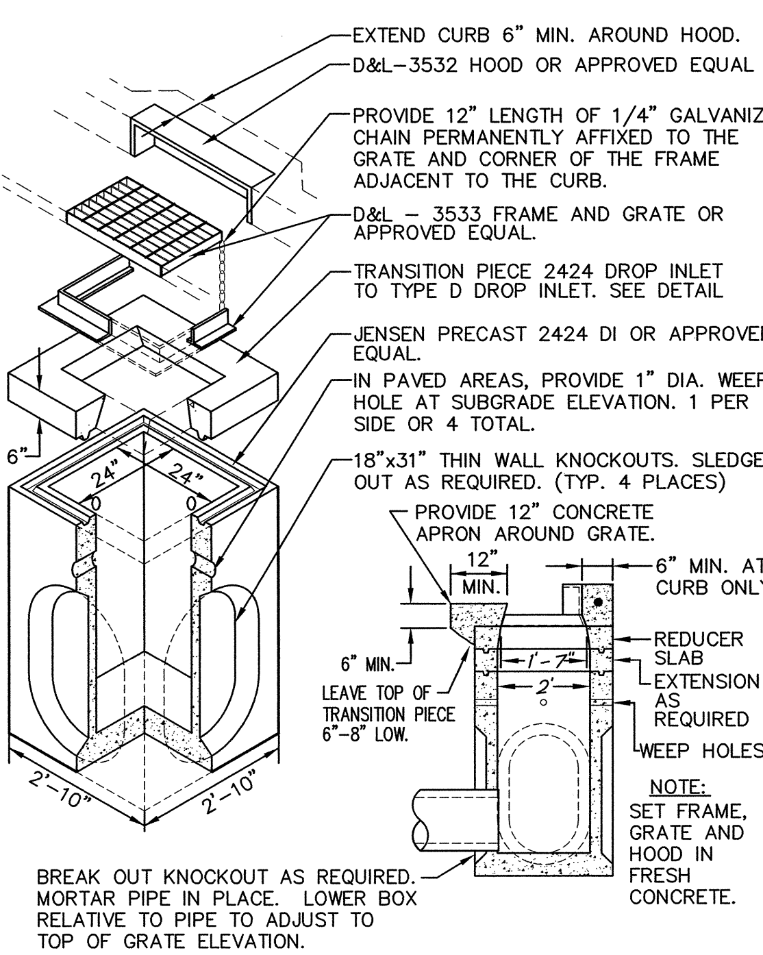
6 C6.1 CURB INLET NO SCALE
