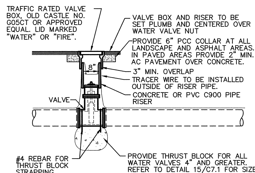
10 C6.1 WATER VALVE NO SCALE
