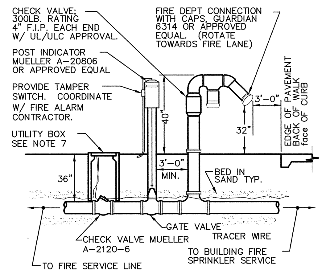
10 C6.1 WATER VALVE NO SCALE
