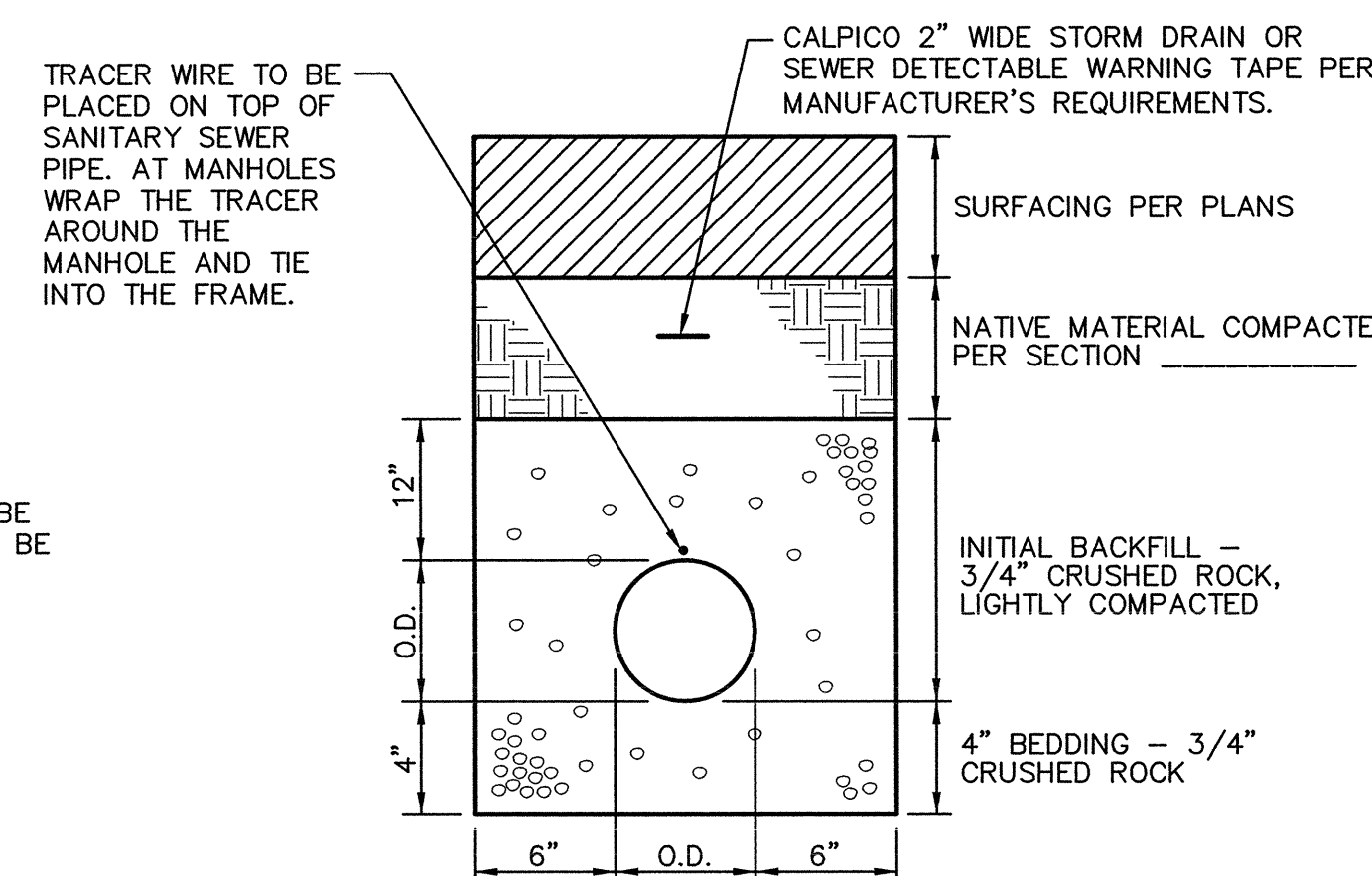
7 C6.1 STORM DRAIN AND SEWER TRENCH NO SCALE
