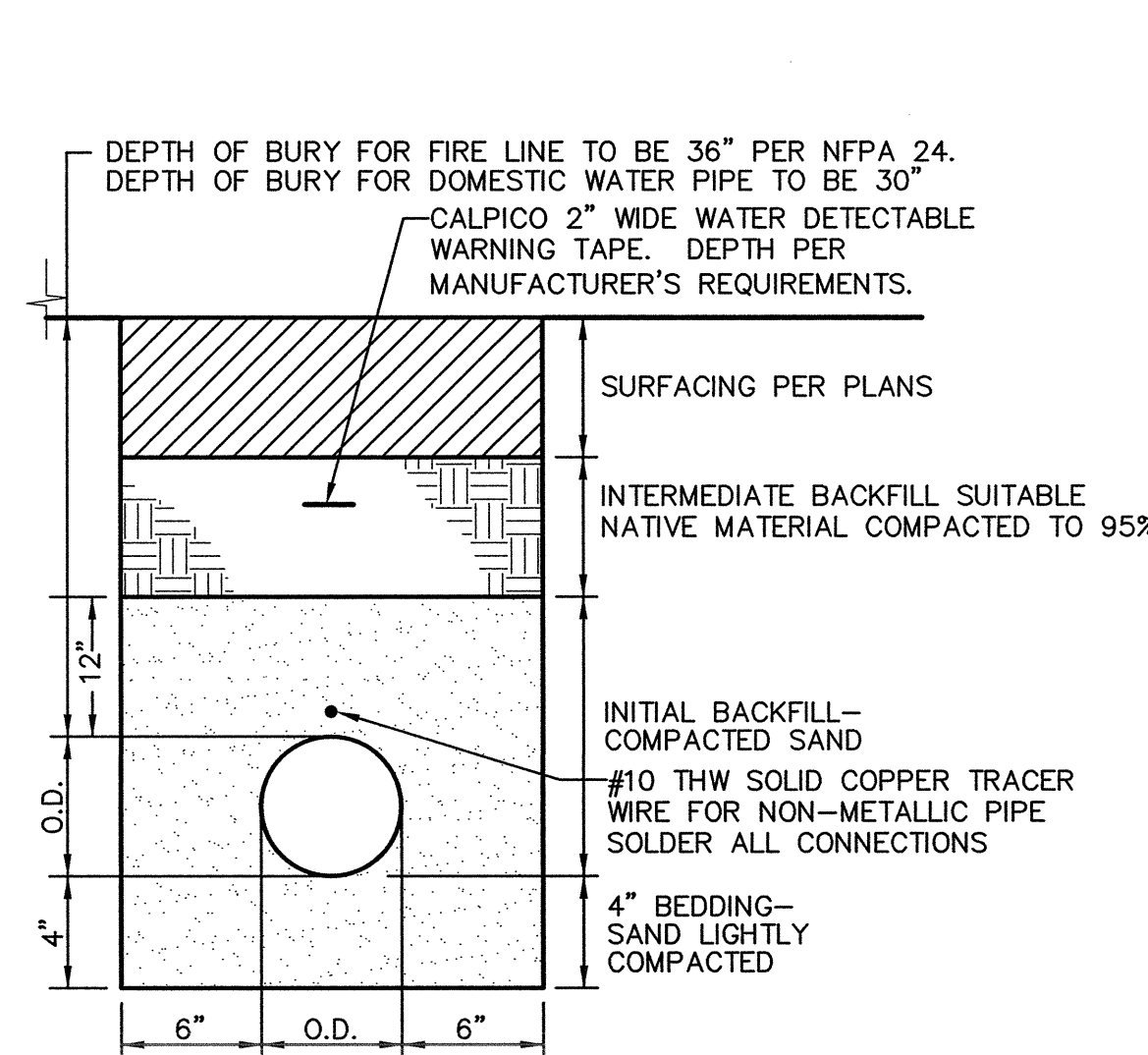
9 C6.1 WATER TRENCH NO SCALE
