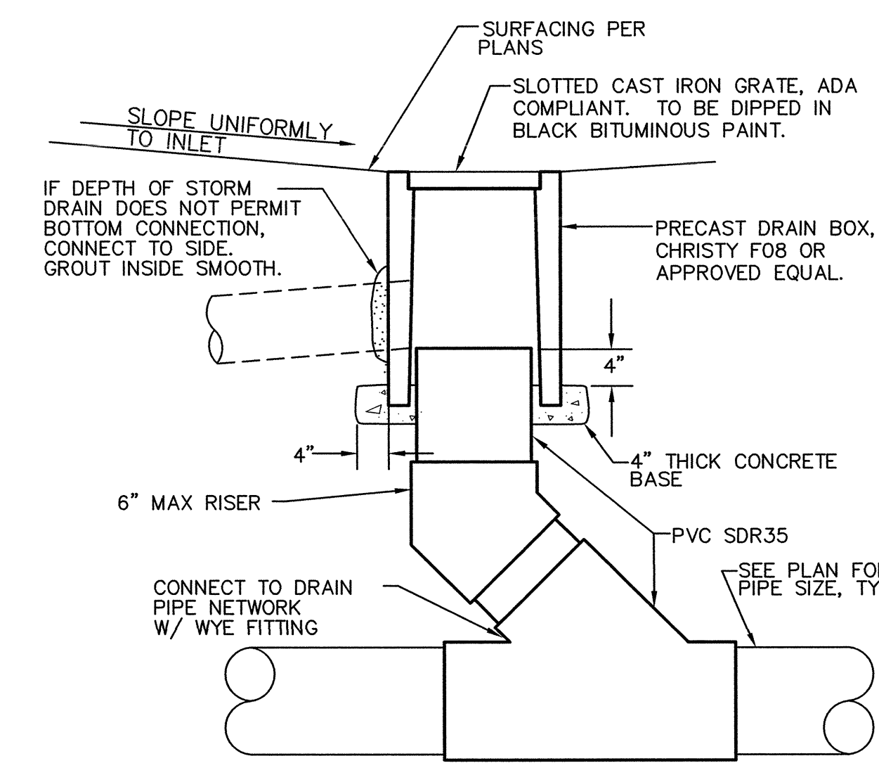
14 C6.1 AREA DRAIN NO SCALE
