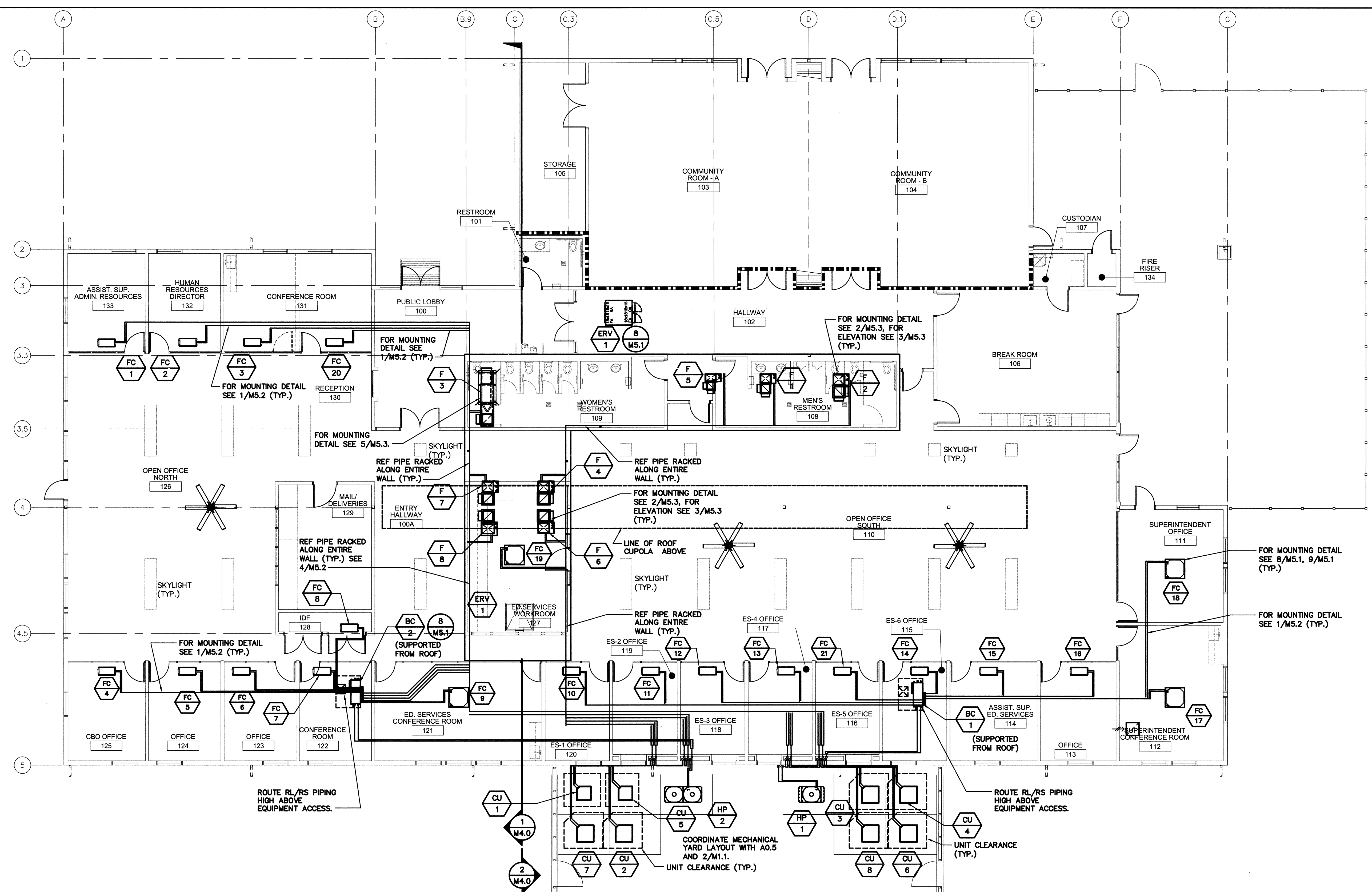
MECHANICAL REFRIGERANT PIPING FLOOR PLAN SCALE : 1/8"=1'-0"
