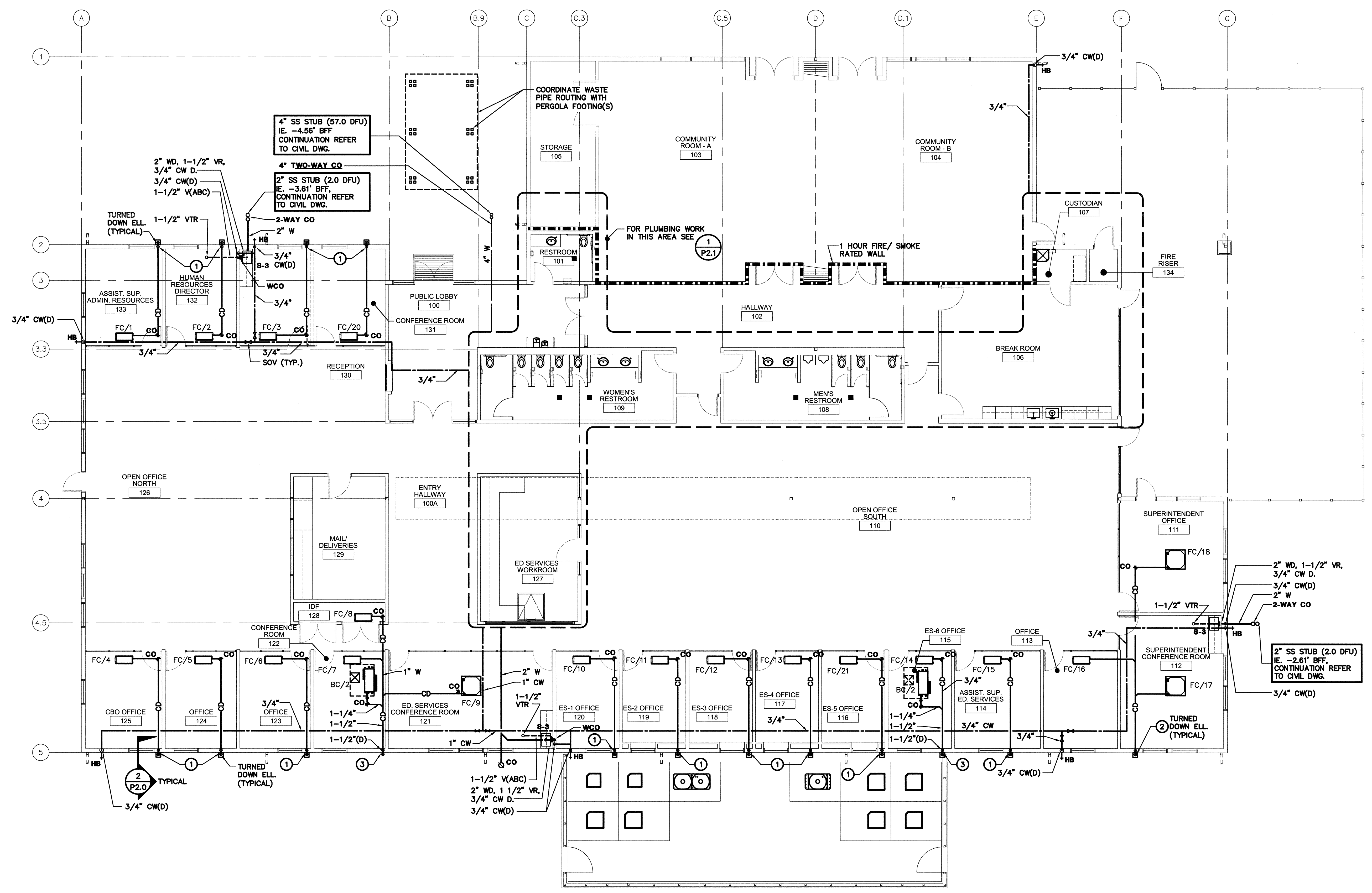
PLUMBING FLOOR PLAN SCALE : 1/8"=1'-0" 1 P2.0
