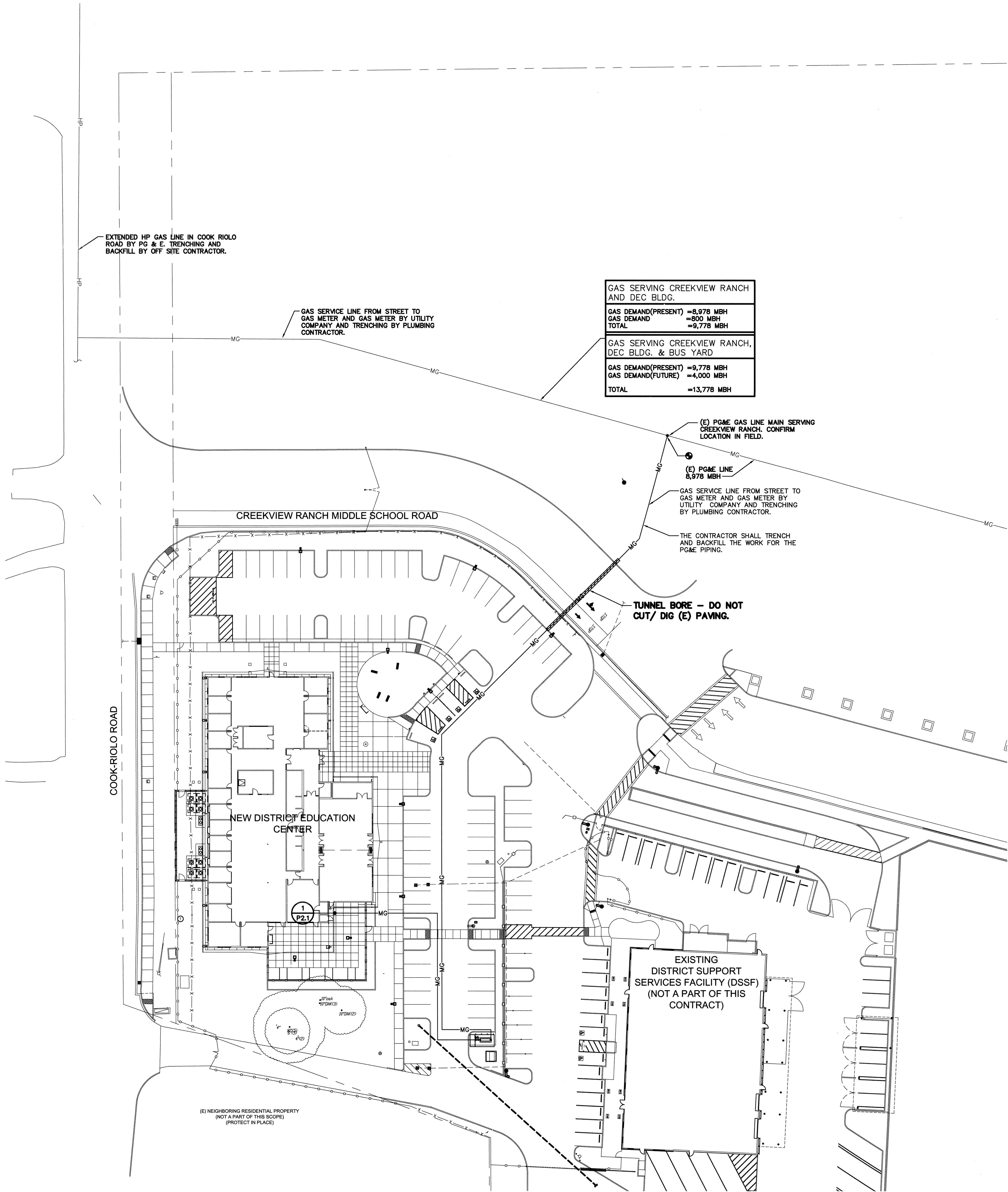
PLUMBING GAS SITE CONNECTION PLAN 1 SCALE : 1"=30'-0" NOTE. 1. SEE SHEET P1.0 FOR ADDITIONAL SITE PLUMBING INFORMATION.
