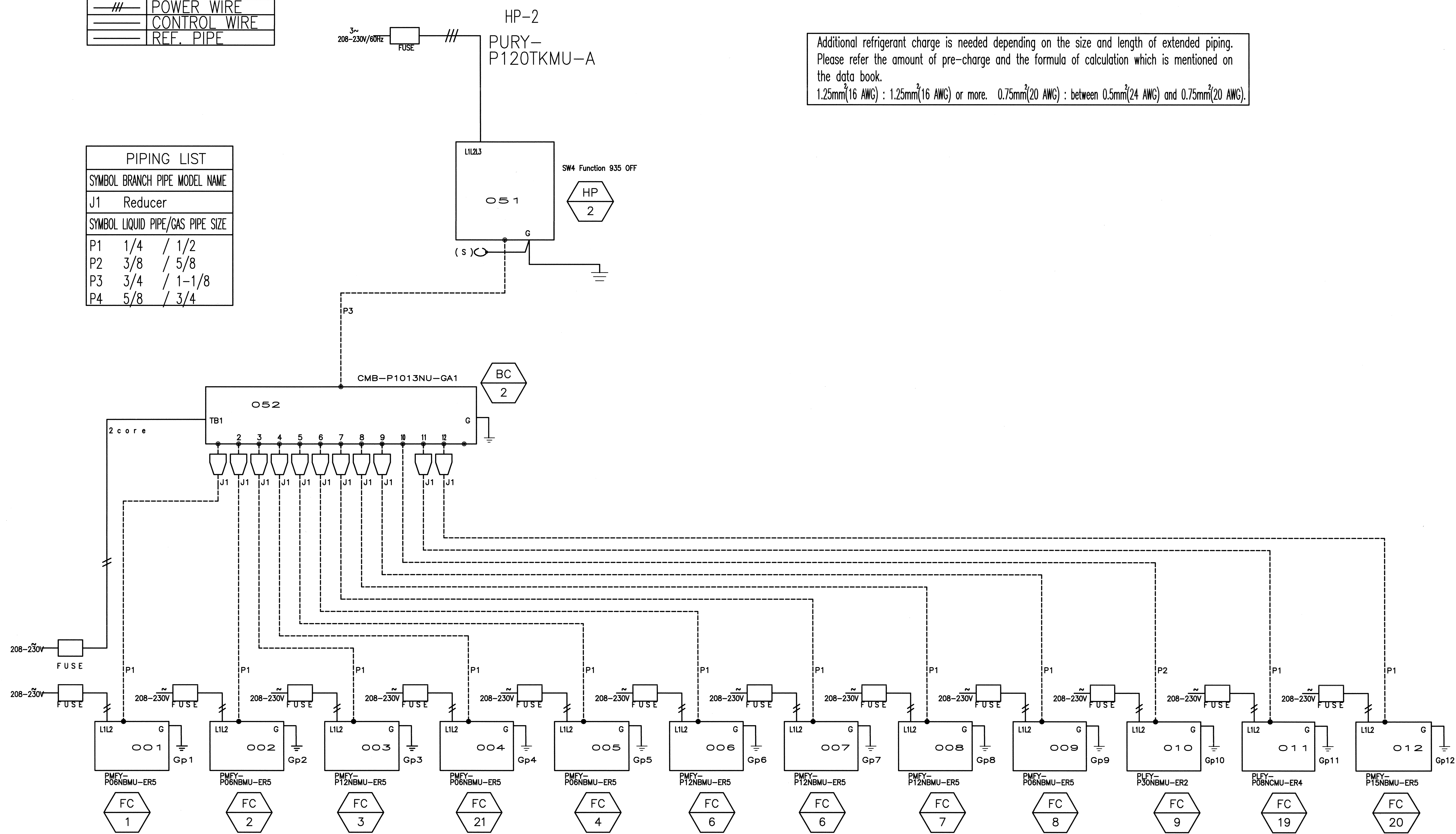
MECHANICAL CONTROL/ PIPING DIAGRAM 1 SCALE : M7.2
