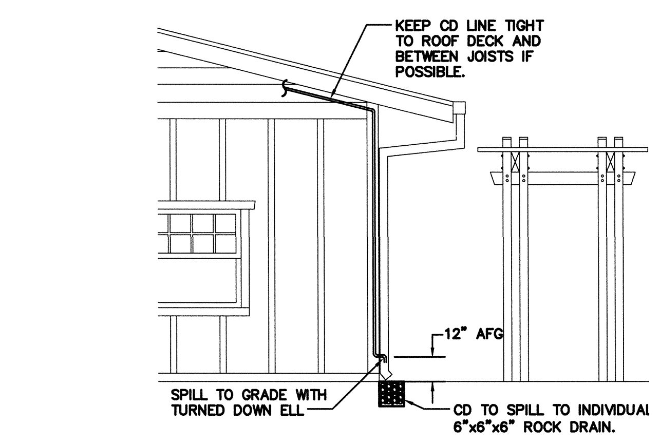
PLUMBING TYPICAL CONDENSATE DRAIN (CD) SPILL TO GRADE. SCALE : NONE 2 P2.0
