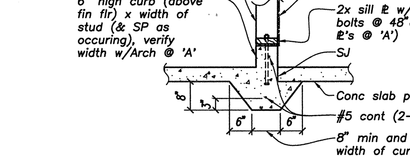
CURB DETAIL (13A)
