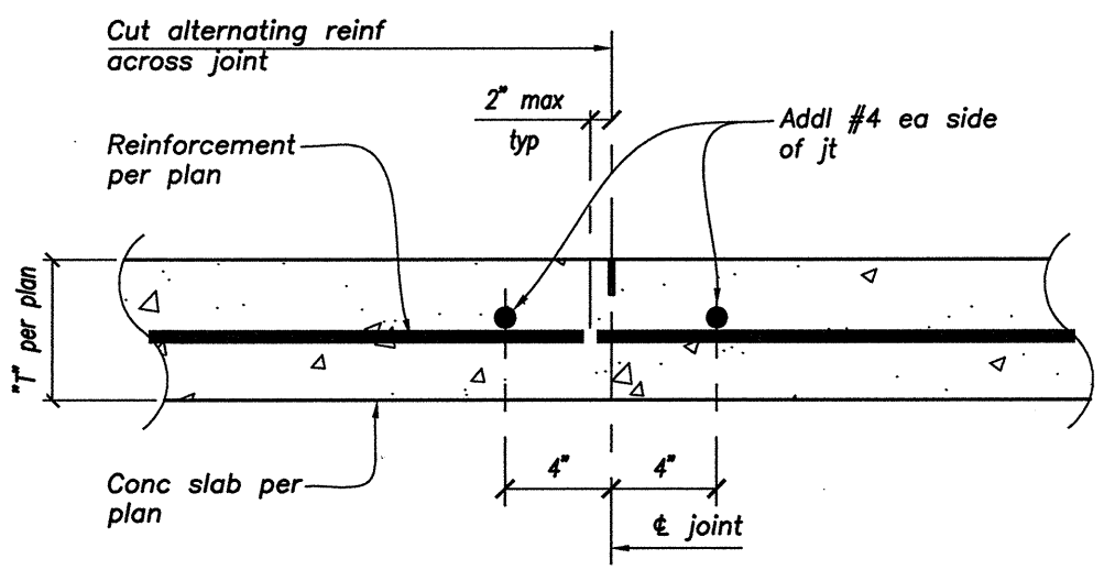
CONTRACTION JOINT IN SLAB (1)
