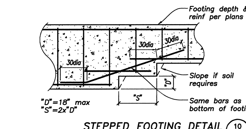
STEPPED FOOTING DETAIL (10)
