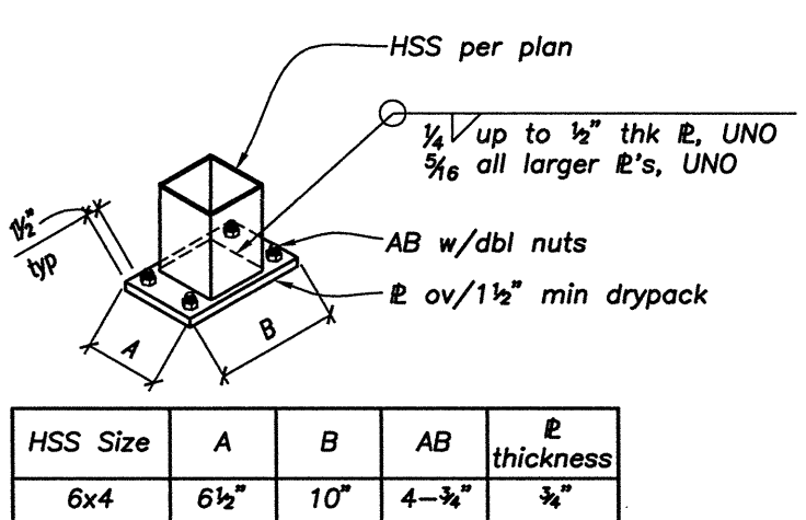
TYPICAL BASE PLATE DETAILS (23)
