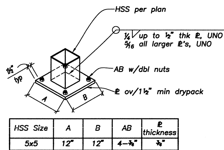
TYPICAL BASE PLATE DETAILS (22)
