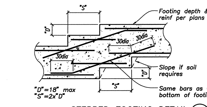
STEPPED FOOTING DETAIL (11)
