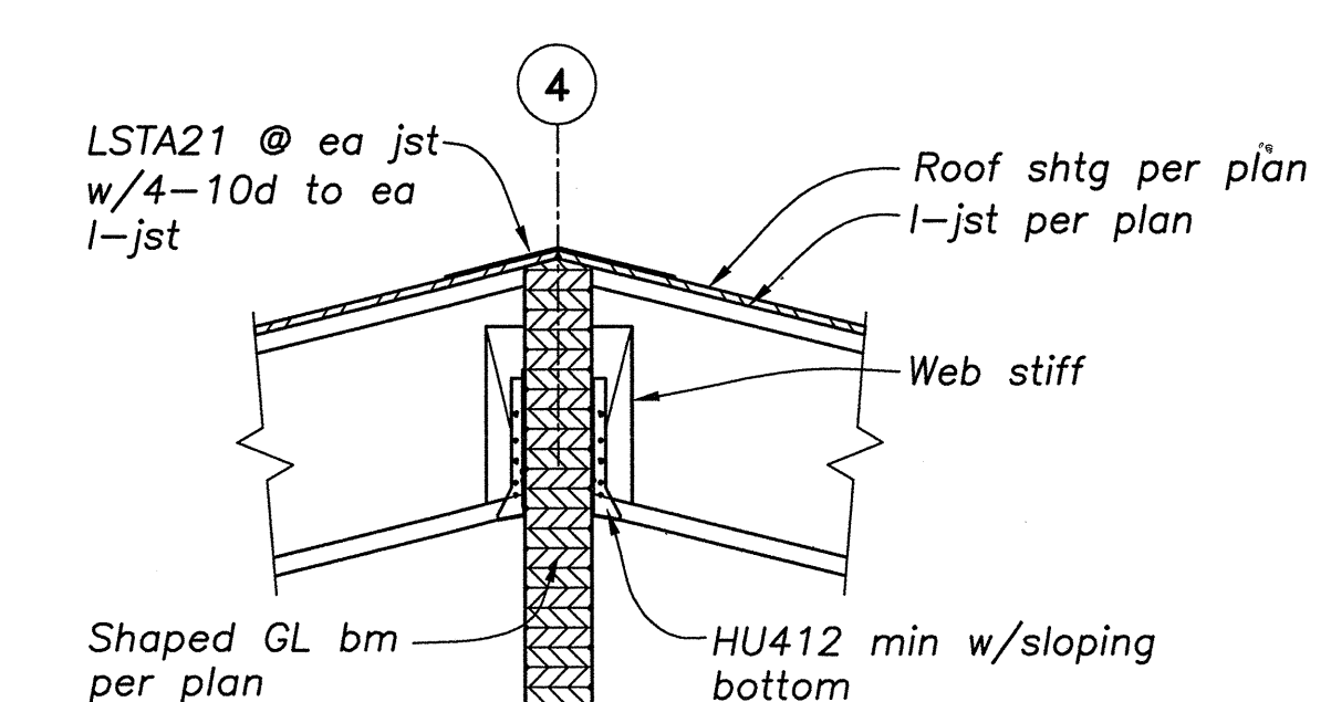
DETAIL 4 3/4"=1'-0" S4.2
