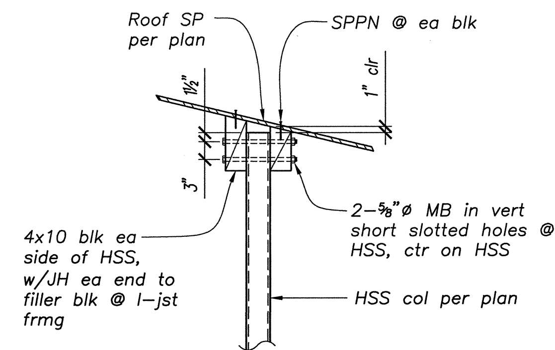
DETAIL 5 3/4\"/>
