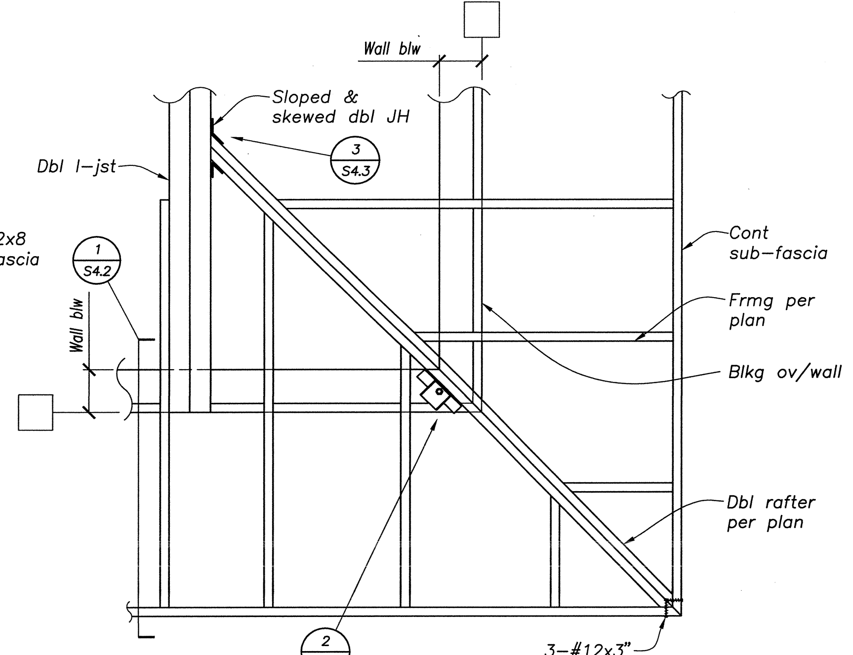
DETAIL 1 3/4" = 1'-0" S4.3
