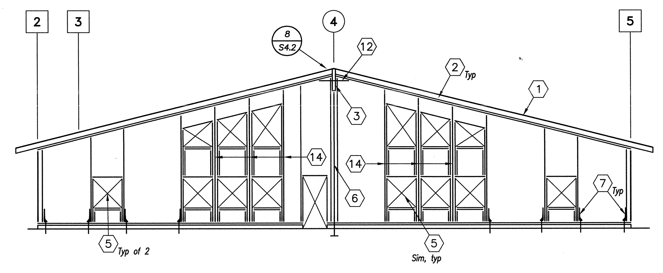
WALL FRAMING ELEVATION - LINE A \frac{1}{8}'' = 1'-0''
