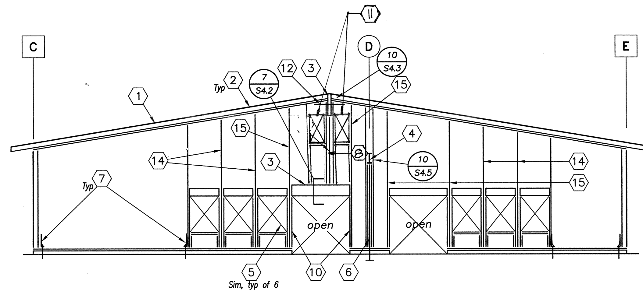
WALL FRAMING ELEVATION - LINE 1 1/8" = 1'-0"
