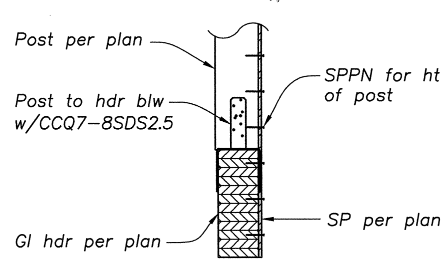
DETAIL 7 3/4"=1'-0" S4.2
