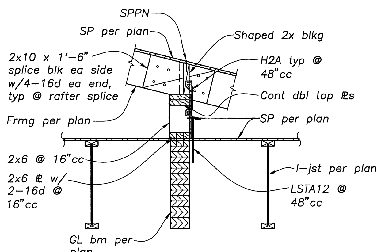
DETAIL 12 3/4" = 1'-0" S4.3
