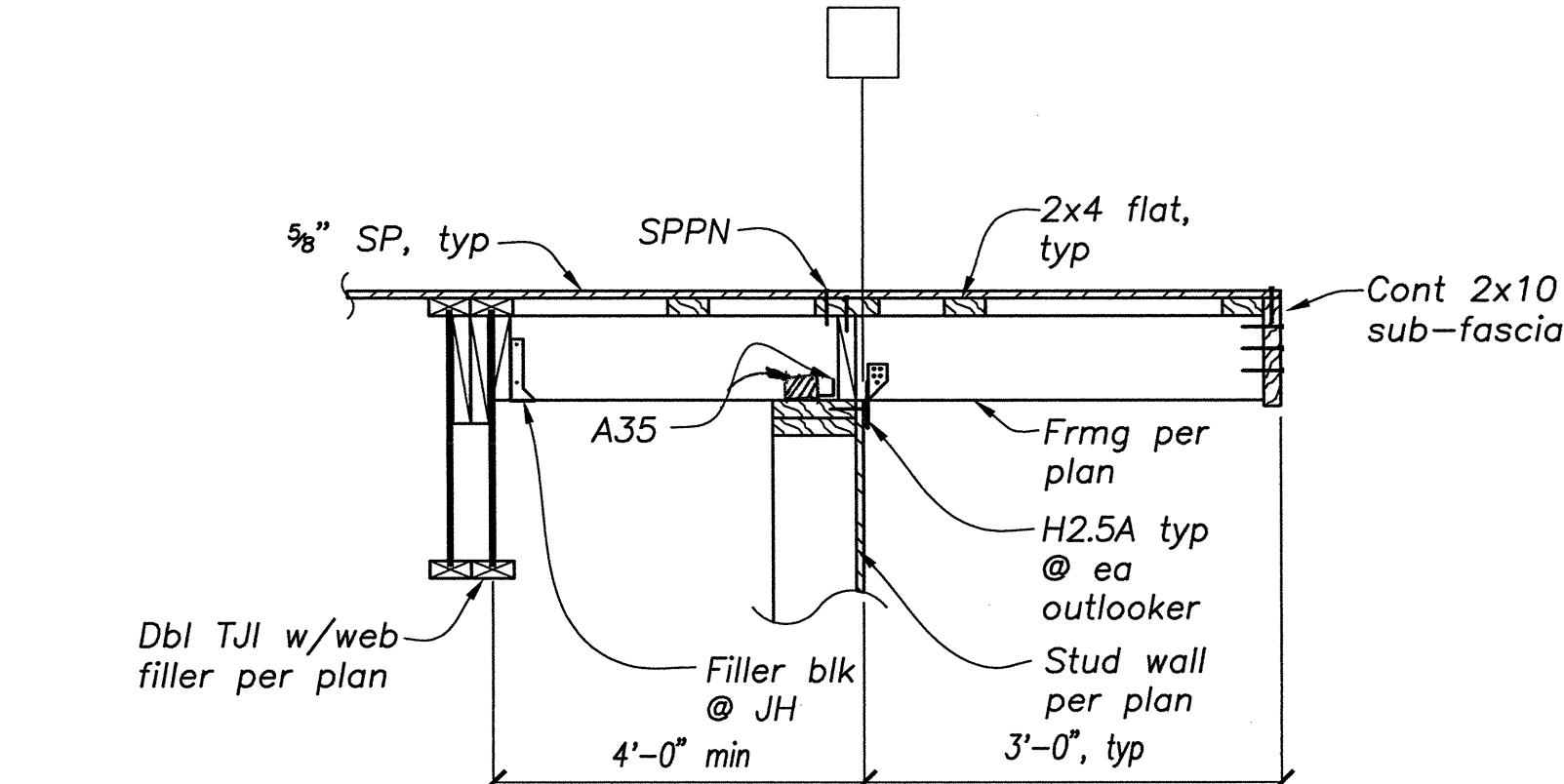
DETAIL 2 3/4"=1'-0" S4.2
