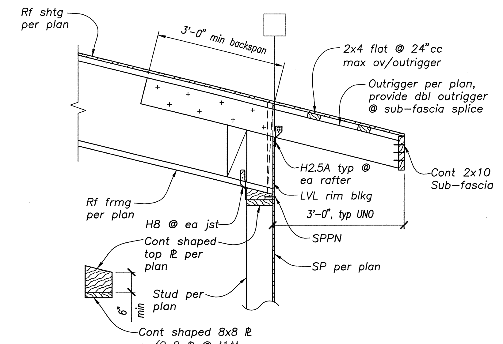
DETAIL 1 3/4"=1'-0" S4.2
