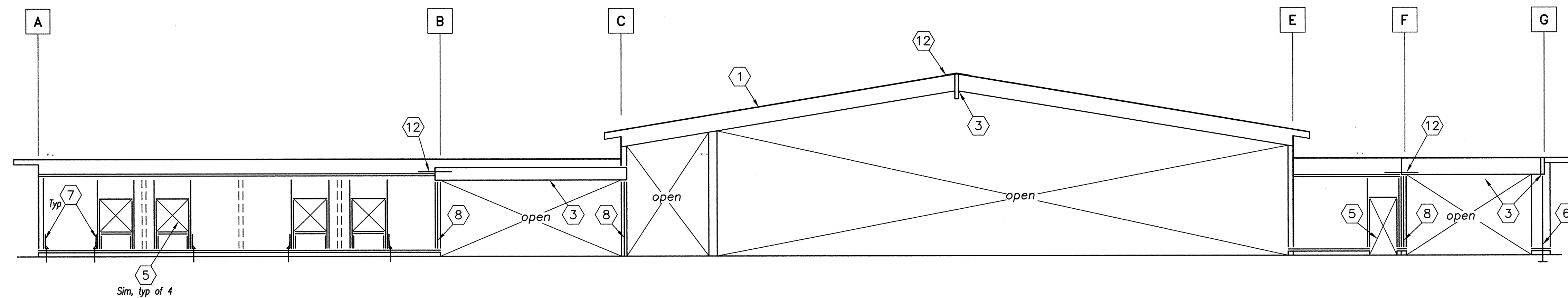
WALL FRAMING ELEVATION - LINE 2 1/8" = 1'-0"
