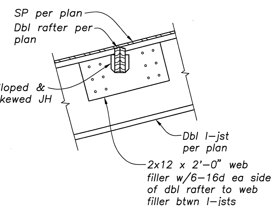
DETAIL 3 3/4" = 1'-0" S4.3
