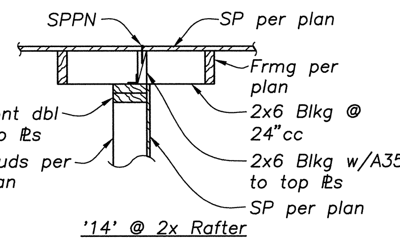
DETAIL 14 3/4" = 1'-0" S4.3
