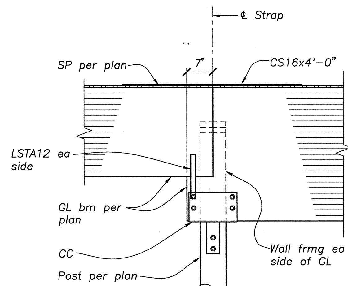
DETAIL 15 3/4"=1'-0" S4.2
