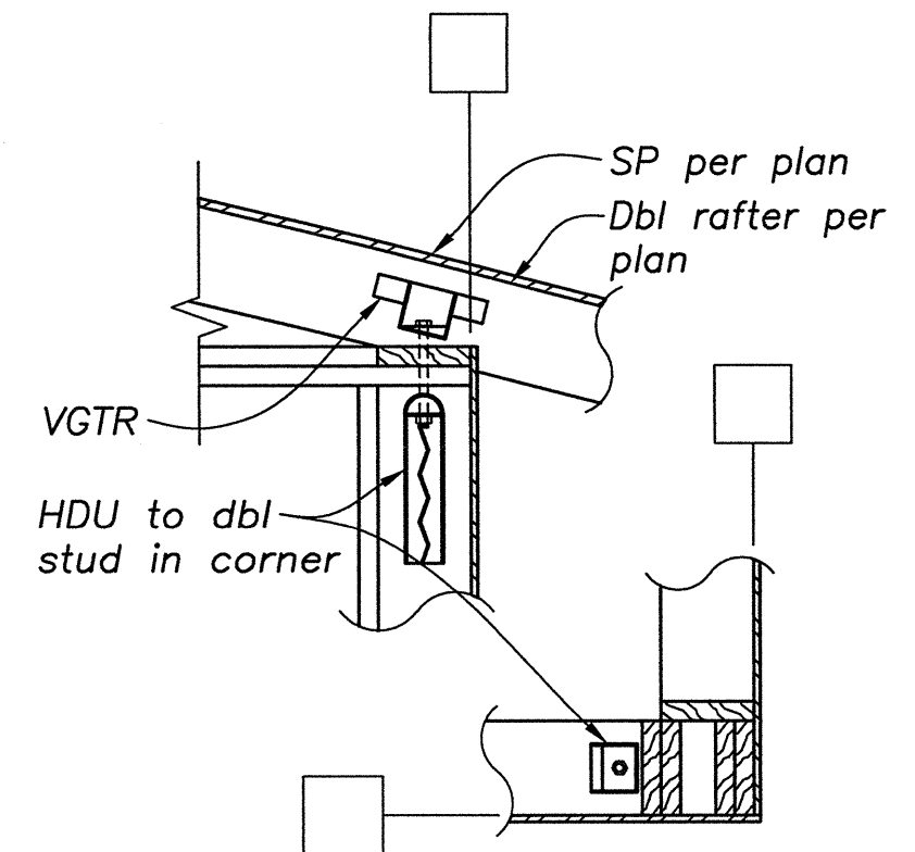
DETAIL 2 3/4" = 1'-0" S4.3
