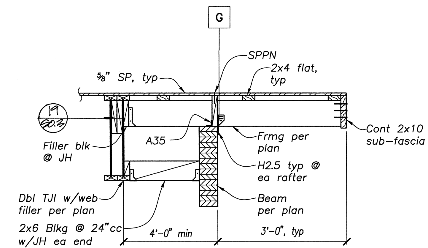
DETAIL 6 3/4"=1'-0" S4.2
