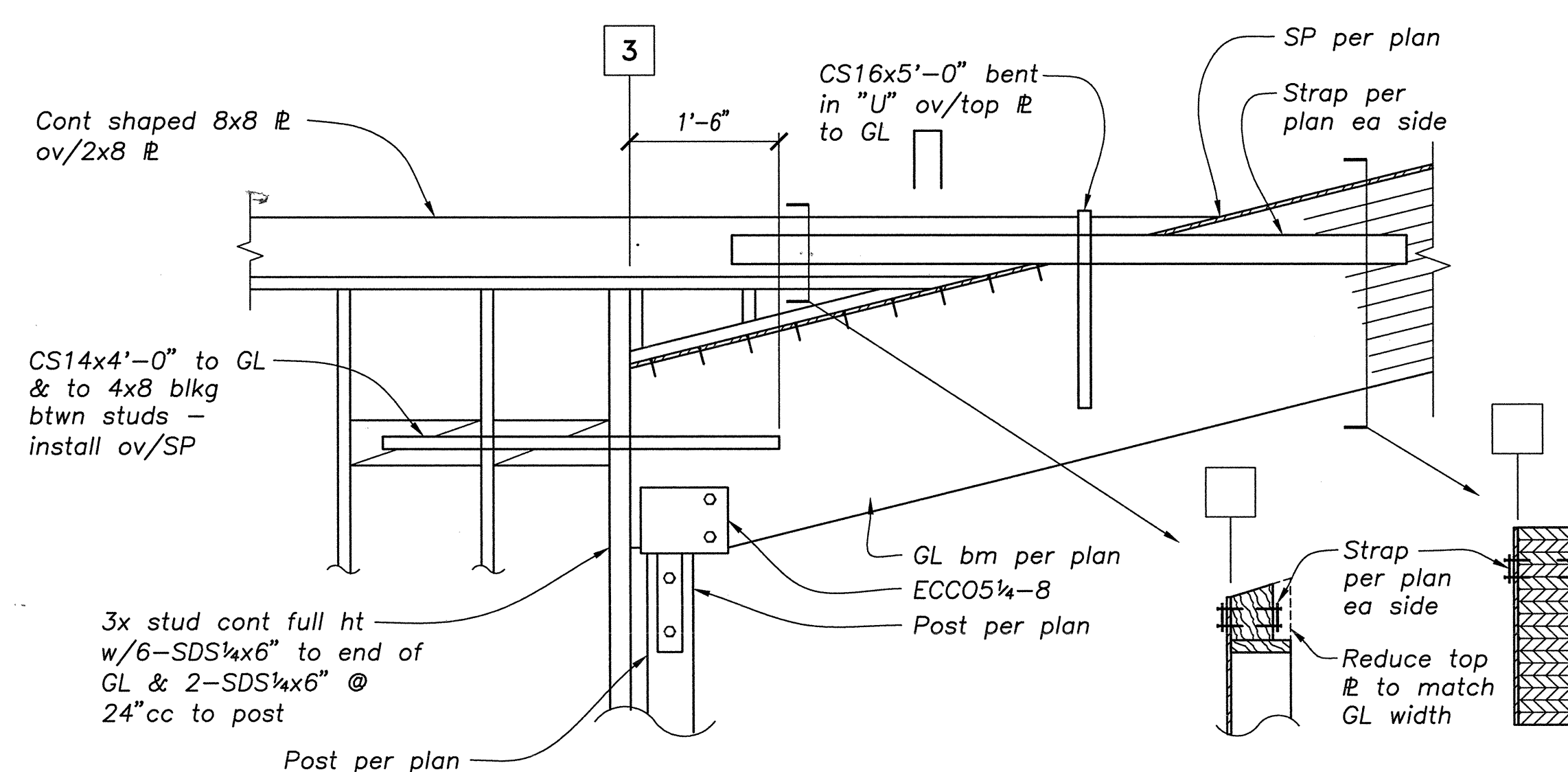
DETAIL 11 3/4"=1'-0" S4.2
