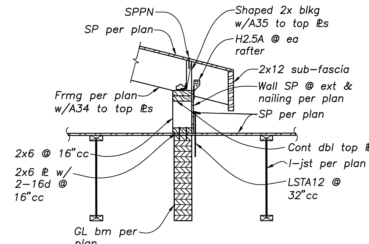
DETAIL 4 3/4" = 1'-0" S4.3
