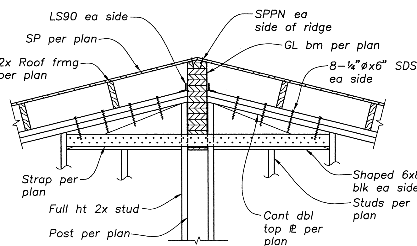
DETAIL 10 3/4" = 1'-0" S4.3
