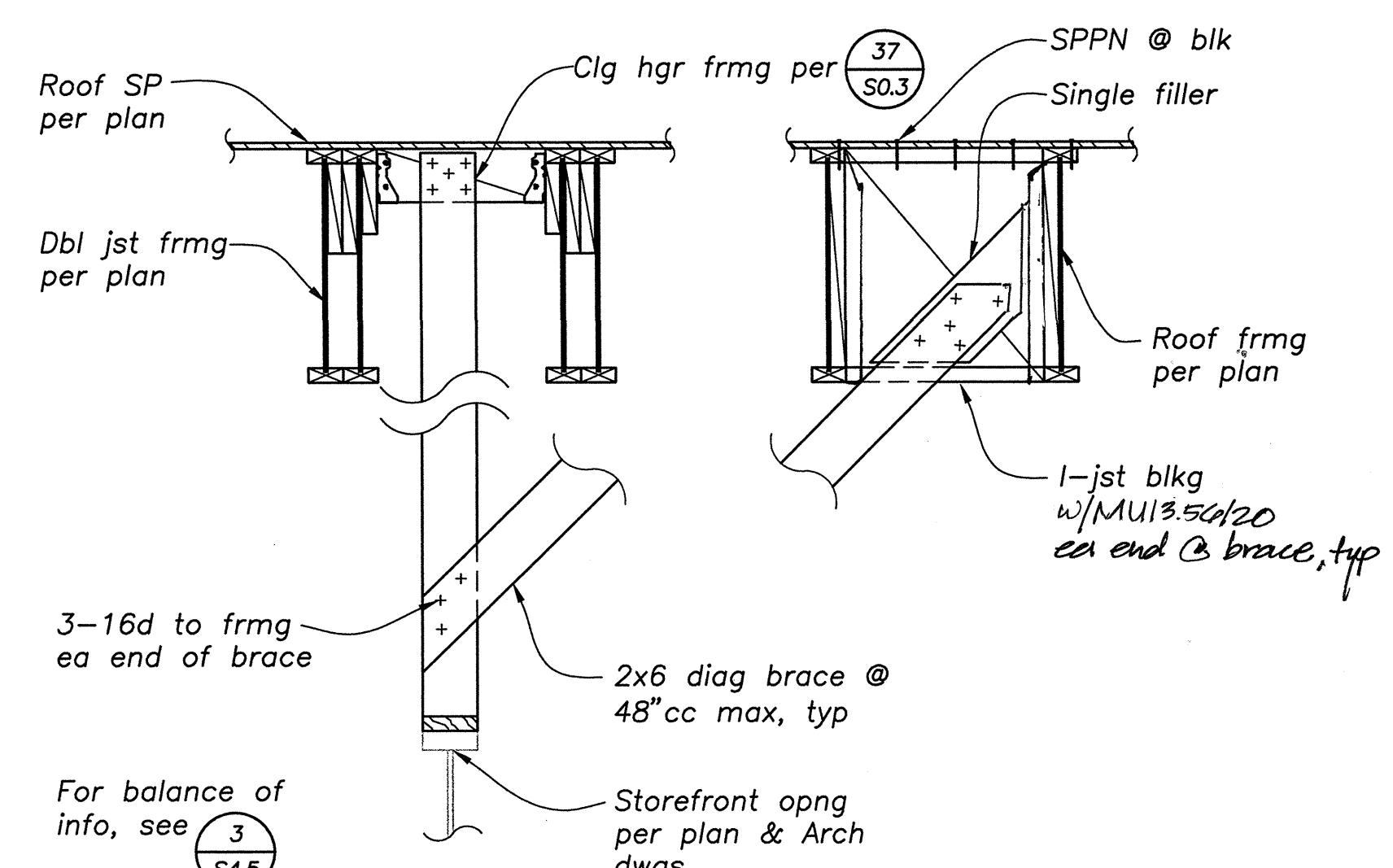
DETAIL 4 3/4\"/>
