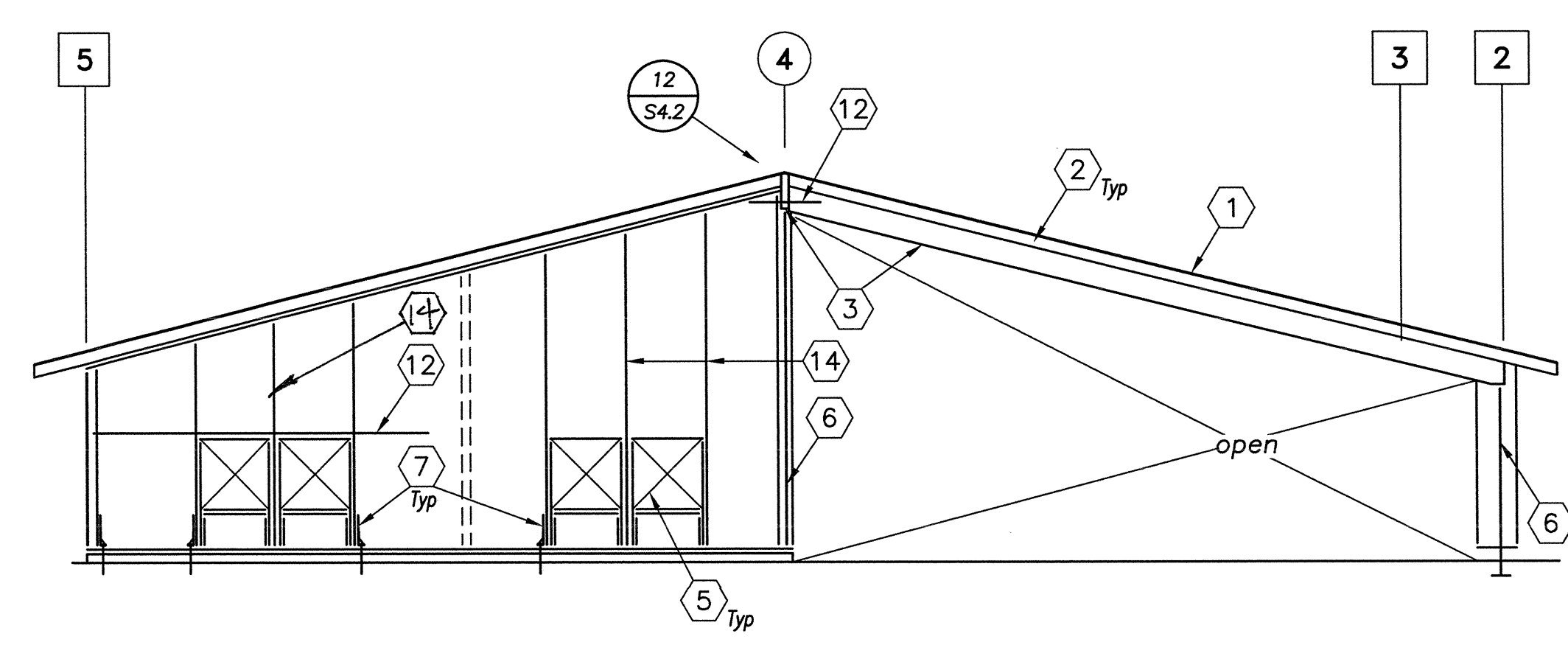
WALL FRAMING ELEVATION - LINE G \frac{1}{8}'' = 1'-0''
