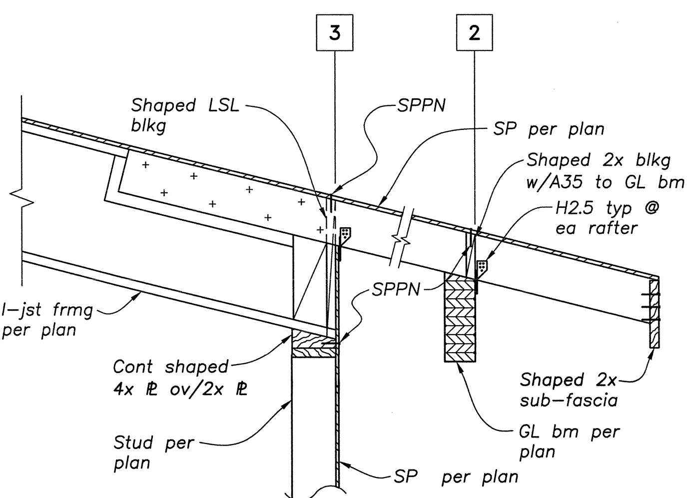
DETAIL 15 3/4" = 1'-0" S4.3
