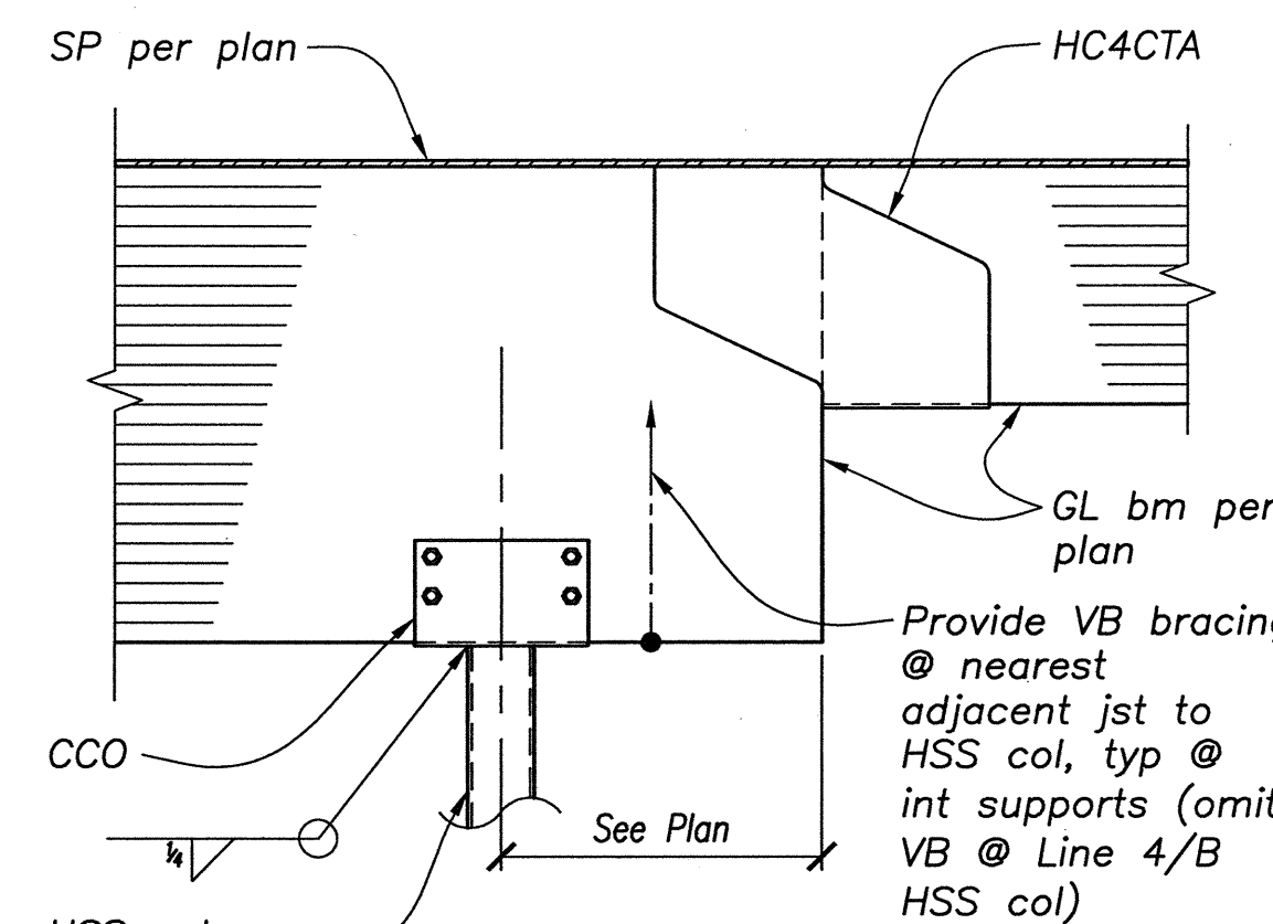
DETAIL 9 3/4"=1'-0" S4.2
