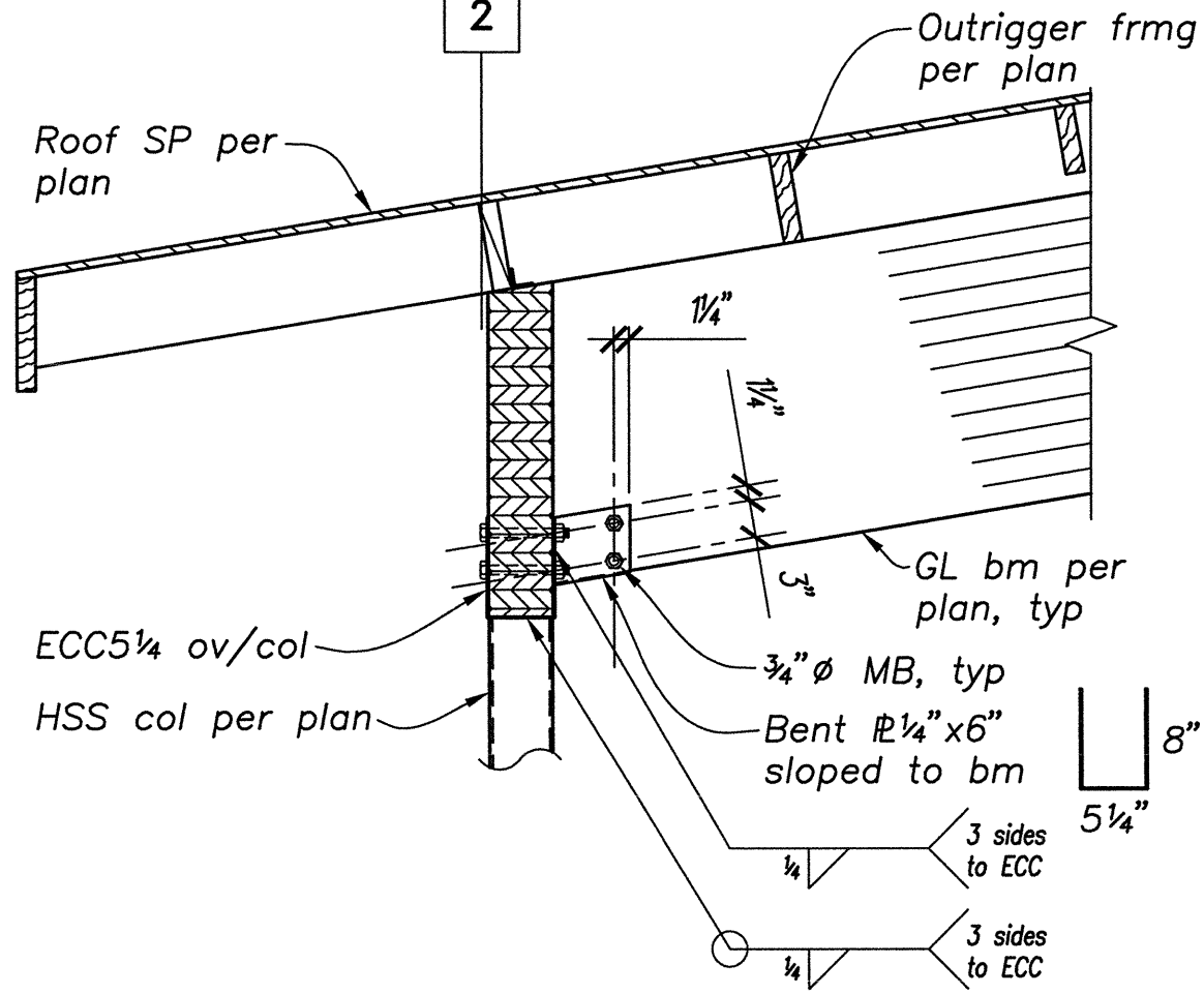
DETAIL 7 3/4" = 1'-0" S4.3
