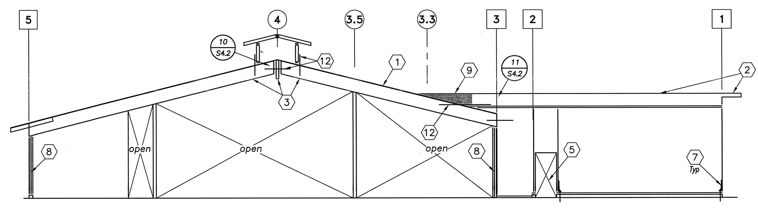
WALL FRAMING ELEVATION - LINE E \frac{1}{8}'' = 1'-0''
