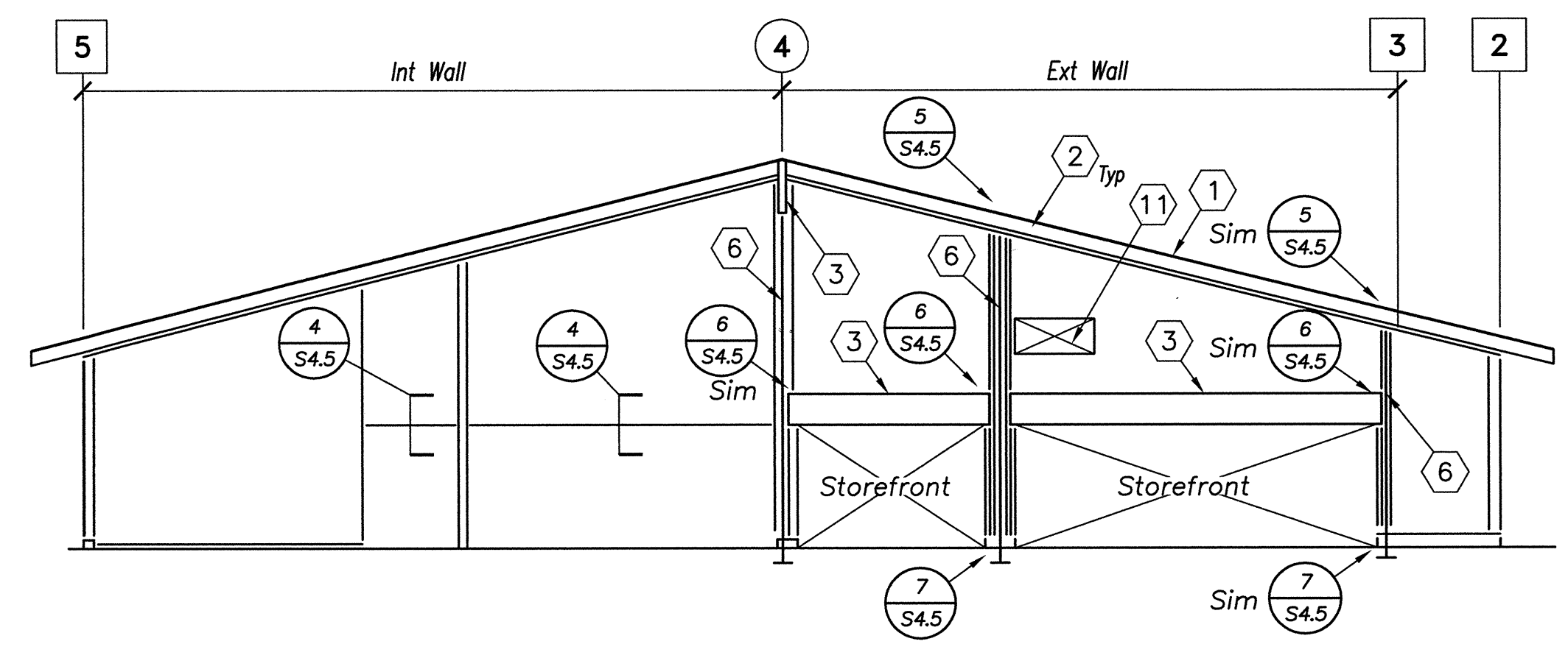
WALL FRAMING ELEVATION - LINE F \frac{1}{8}'' = 1'-0''
