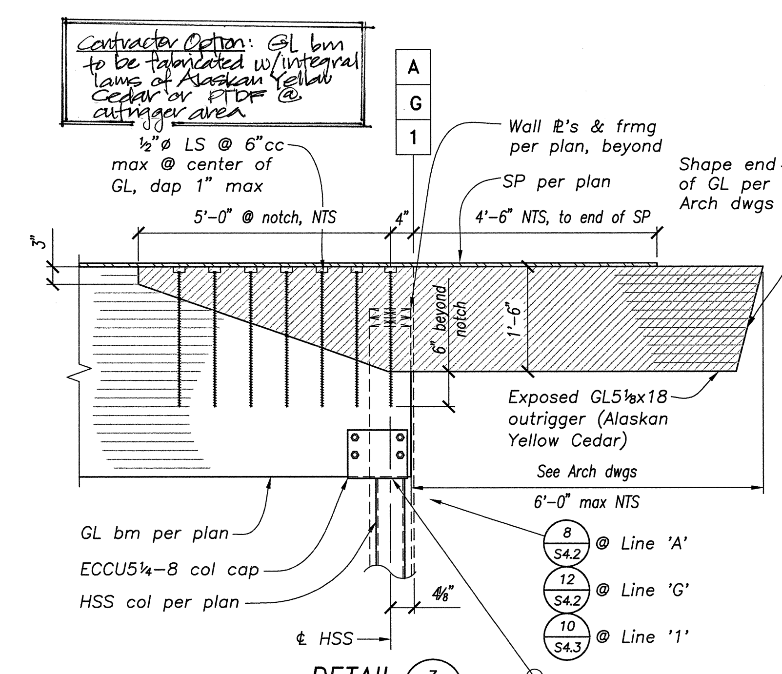
DETAIL 3 3/4"=1'-0" S4.2
