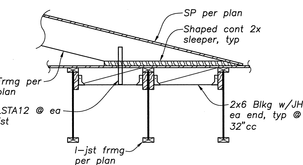
DETAIL 8 3/4" = 1'-0" S4.3
