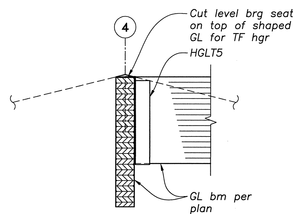
DETAIL 13 3/4"=1'-0" S4.2
