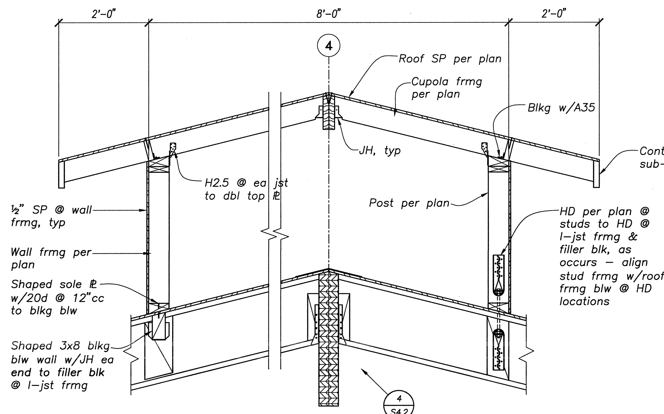
DETAIL 5 3/4" = 1'-0" S4.3
