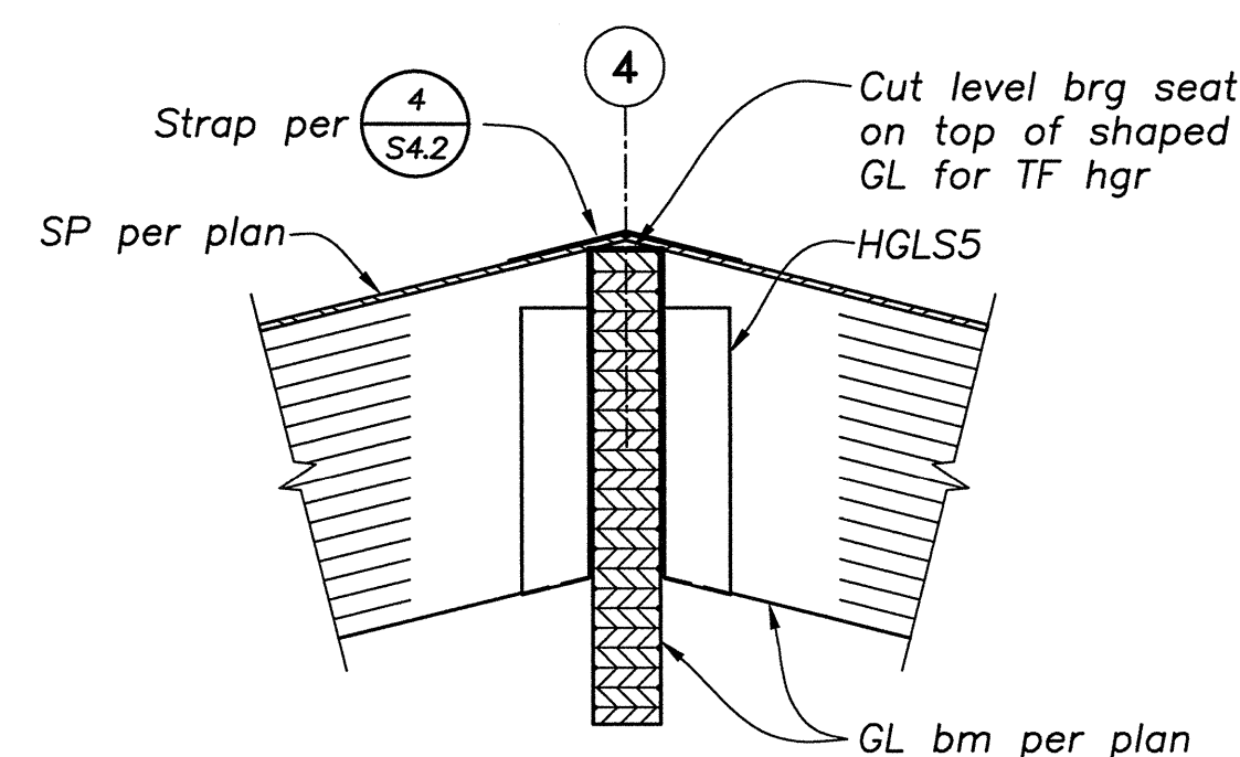
DETAIL 14 3/4"=1'-0" S4.2
