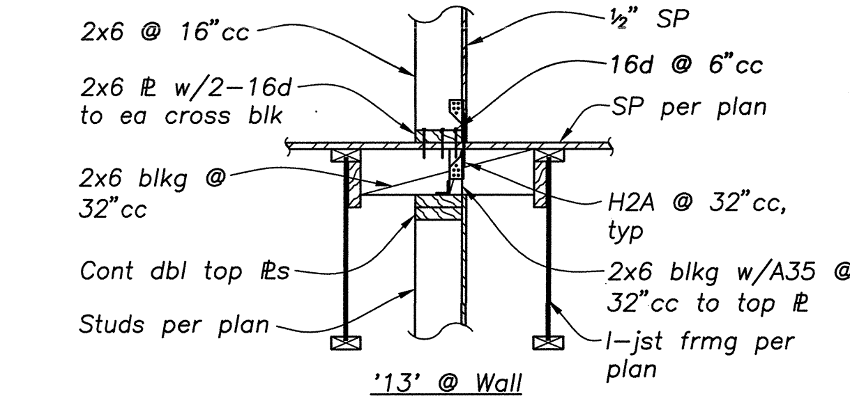
DETAIL 13 3/4" = 1'-0" S4.3
