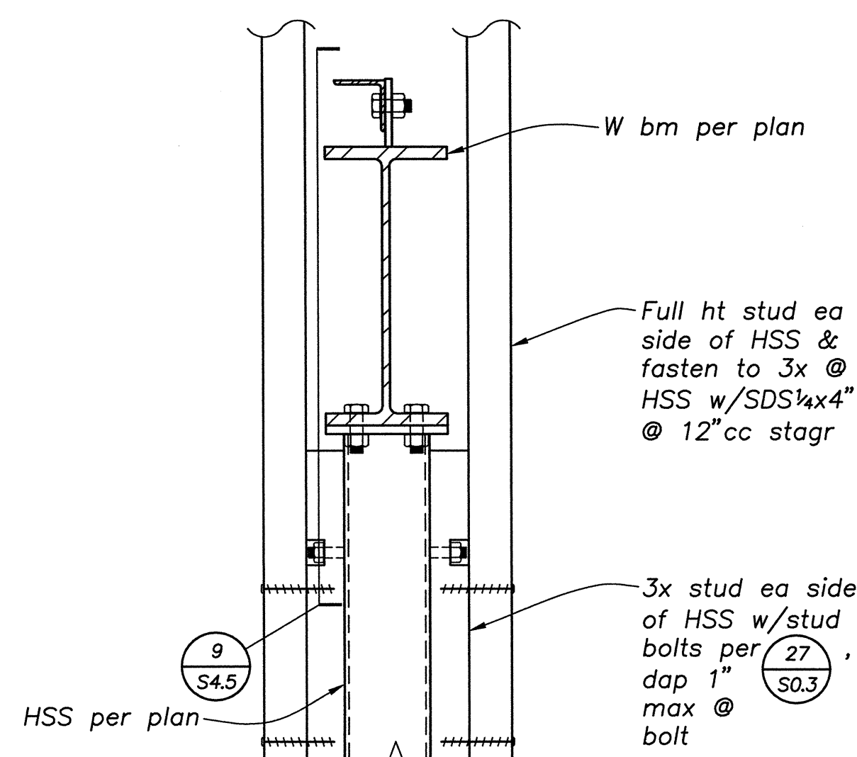
DETAIL 10 1 1/2\"/>
