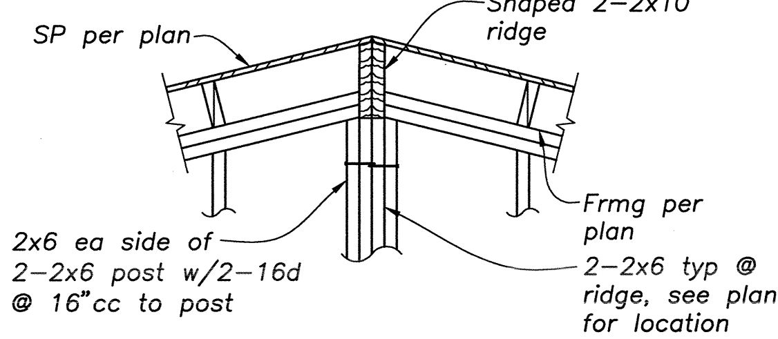
DETAIL 9 3/4" = 1'-0" S4.3
