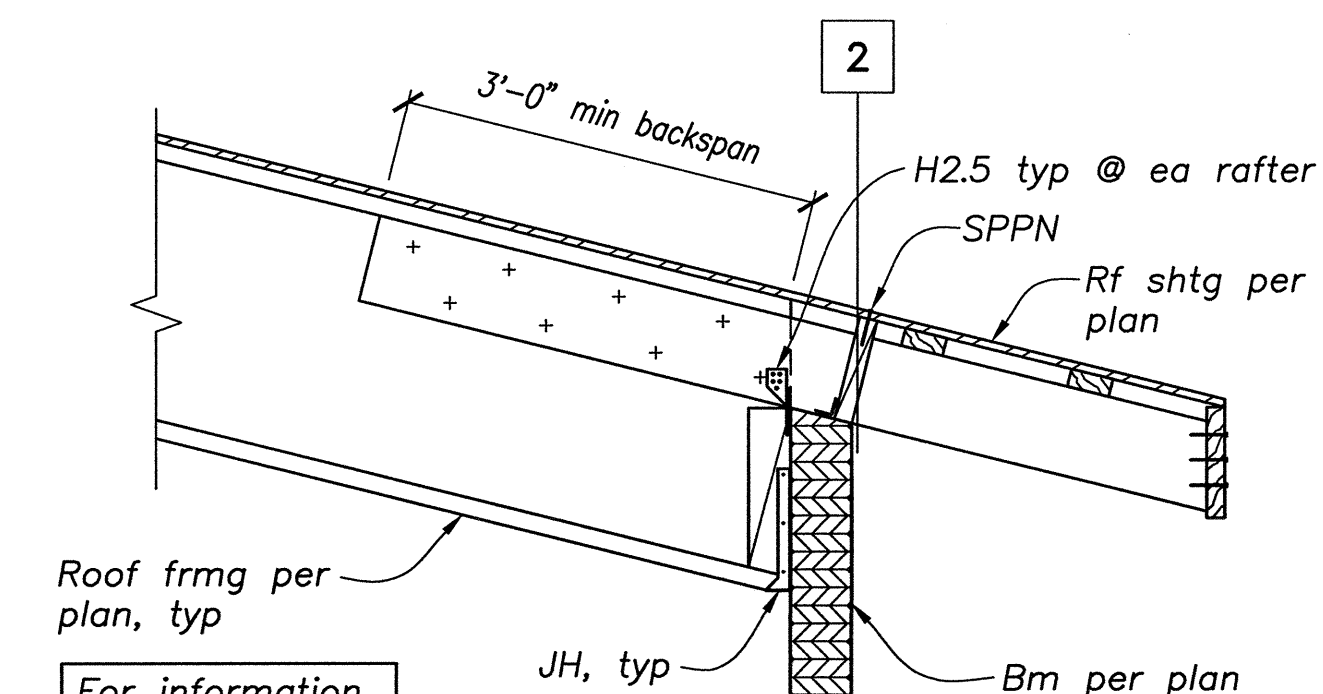
DETAIL 5 3/4"=1'-0" S4.2
