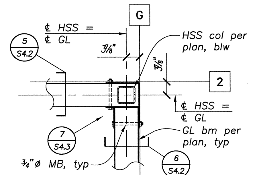
DETAIL 6 3/4" = 1'-0" S4.3
