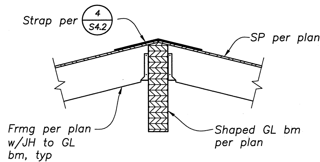
DETAIL 16 3/4" = 1'-0" S4.3
