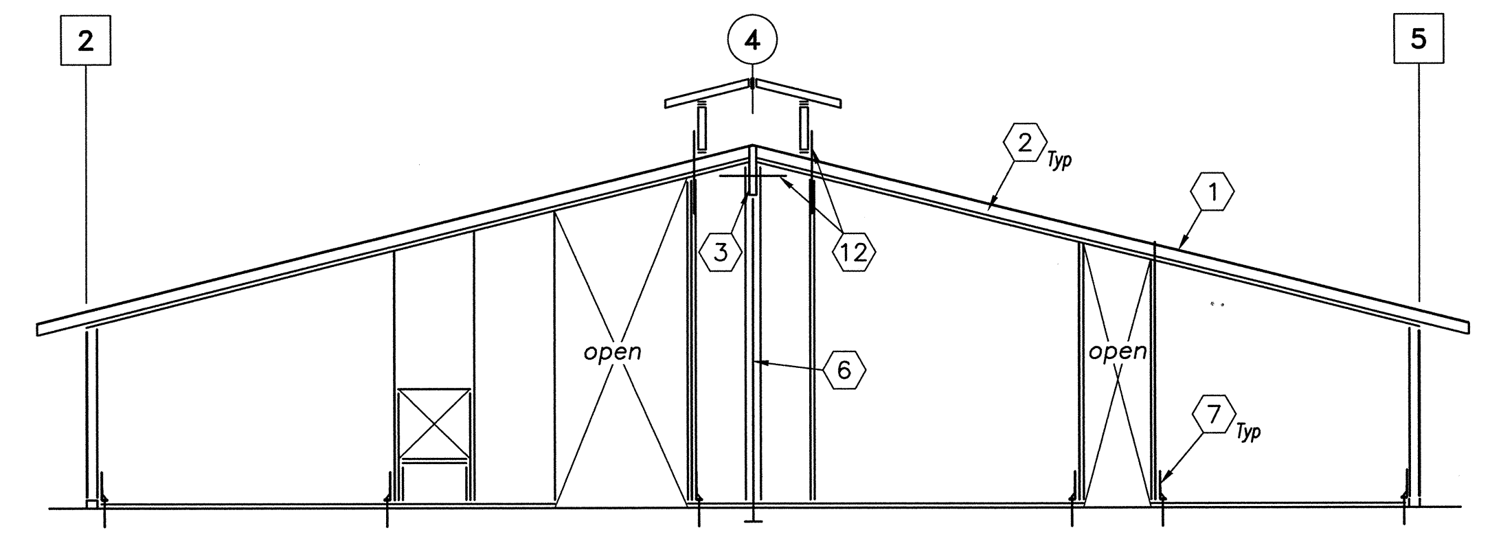
WALL FRAMING ELEVATION - LINE B \frac{1}{8}'' = 1'-0''
