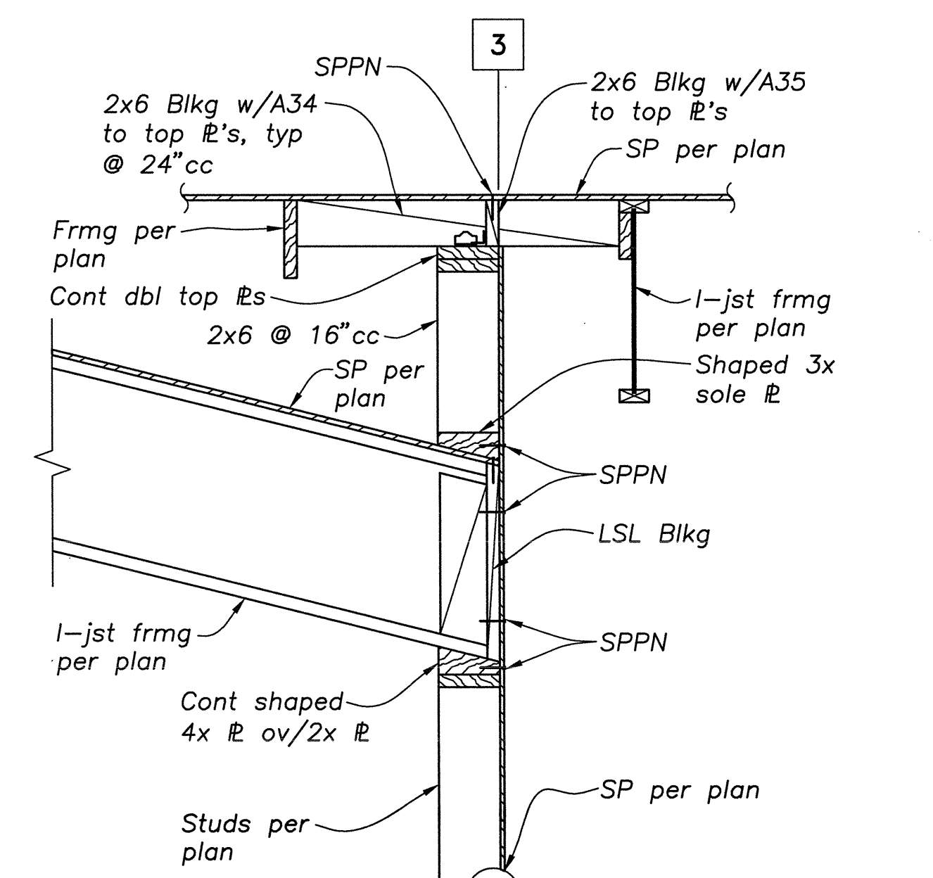
DETAIL 11 3/4" = 1'-0" S4.3
