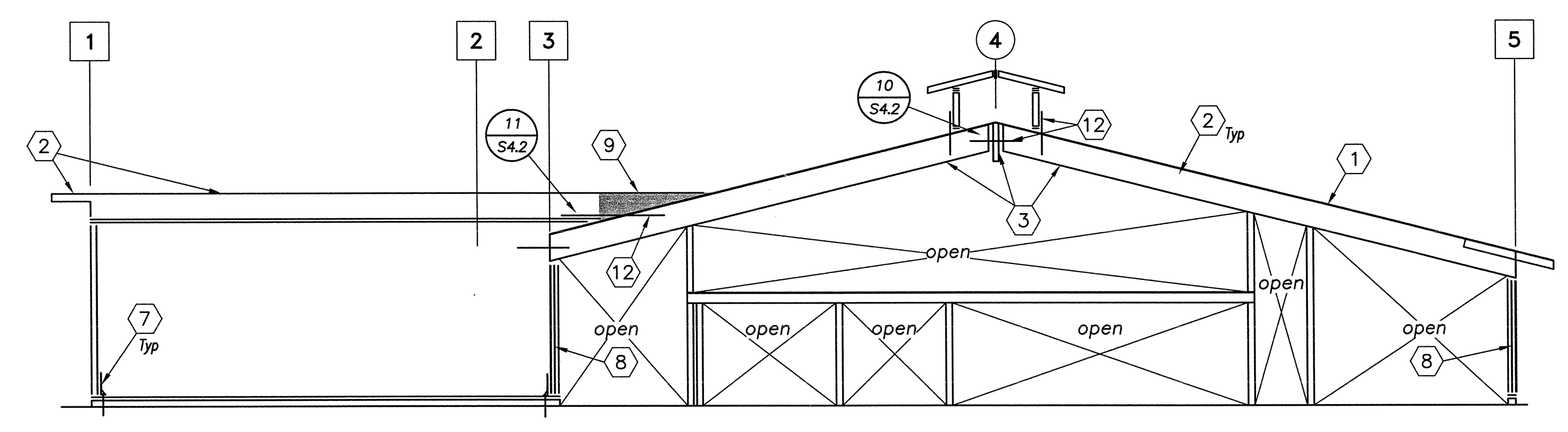
WALL FRAMING ELEVATION - LINE C \frac{1}{8}'' = 1'-0''
