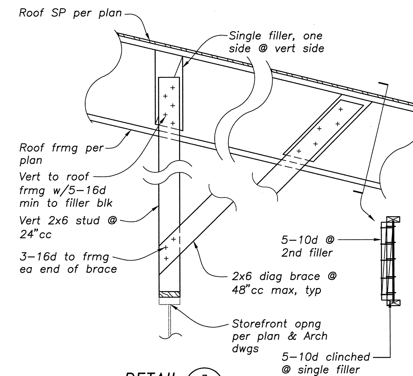
DETAIL 3 3/4\"/>
