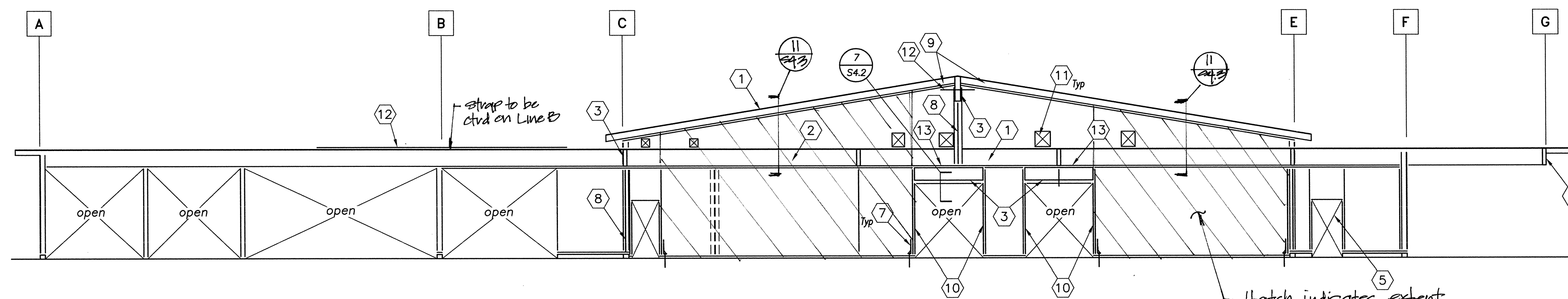
WALL FRAMING ELEVATION - LINE 3 1/8" = 1'-0"
