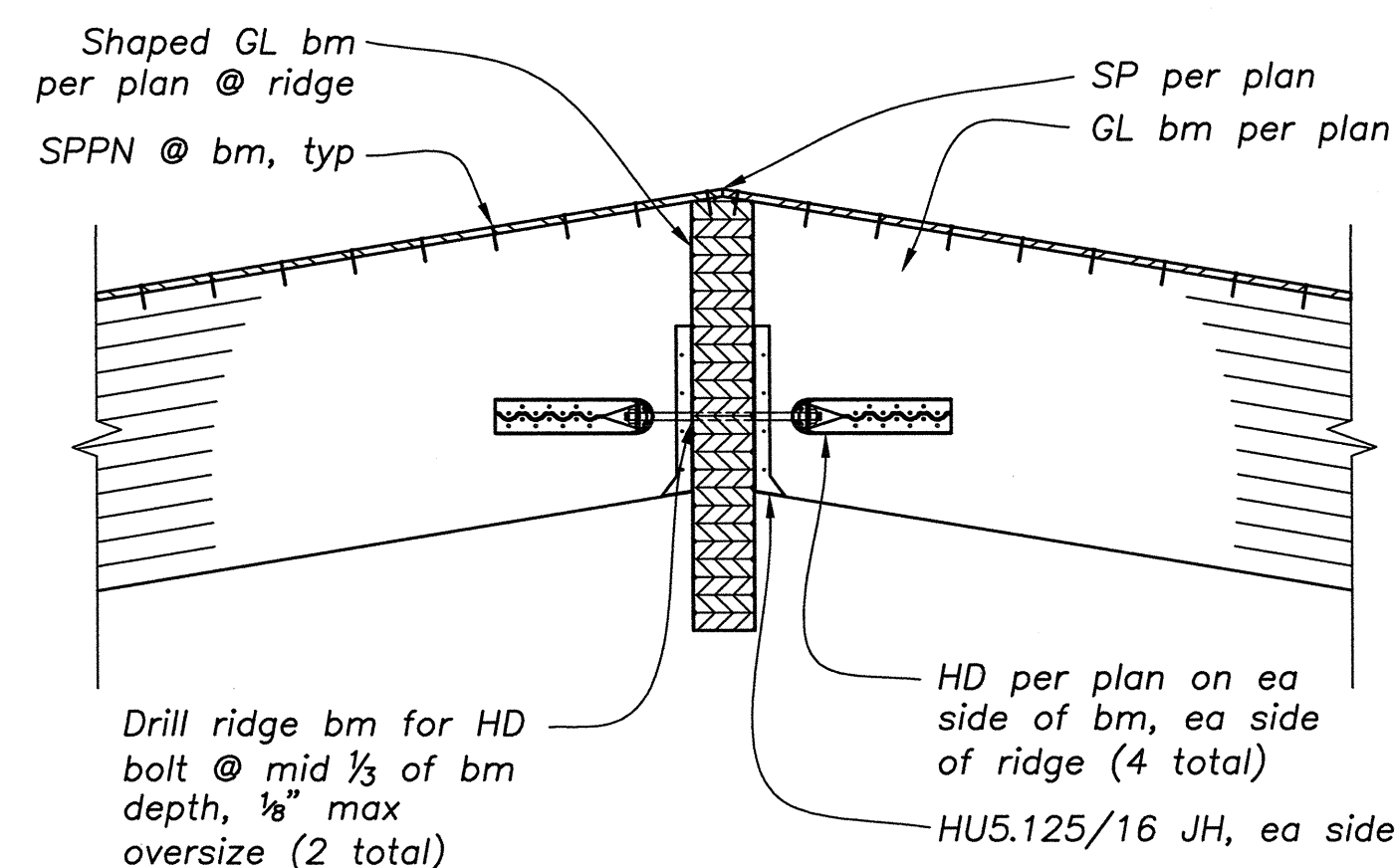
DETAIL 10 3/4"=1'-0" S4.2
