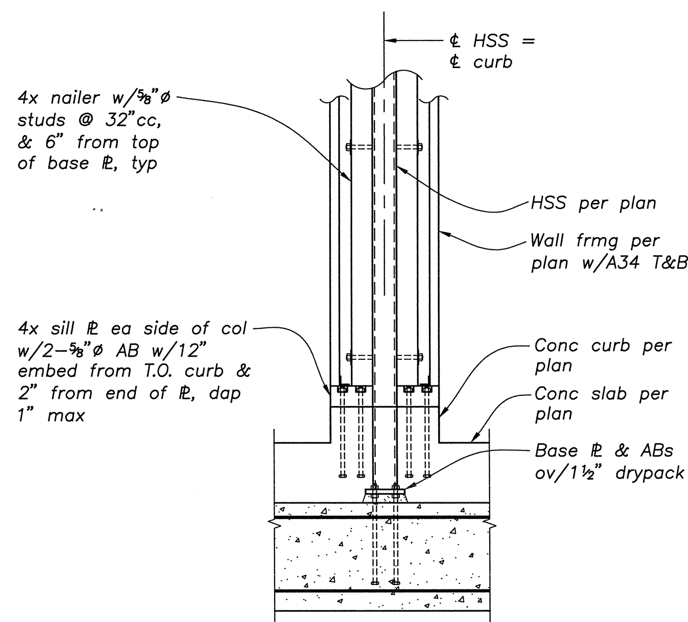
DETAIL 7 3/4\"/>
