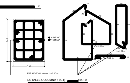
DETALLE COLUMNA 1 (C1)
