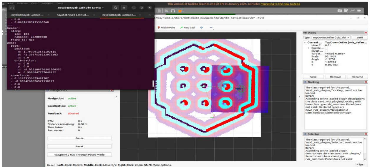
Figure 3: Robot navigating to Goal 1; global path shown in blue
