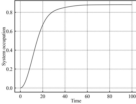
Figure 6: System occupation evolution computed from dynamical map Equation 10
