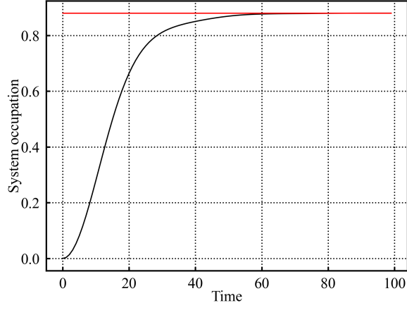
Figure 3: System occupation evolution computed from correlation evolution
