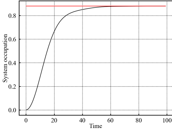
Figure 2: System occupancy over time with red line representing analytical thermalization value
