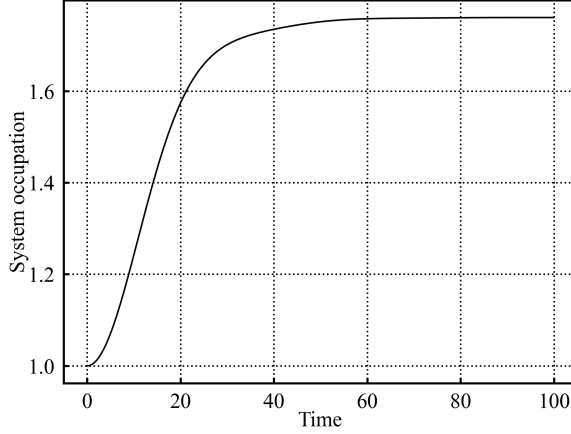
Figure 5: System occupation evolution computed from dynamical map after minor fix
