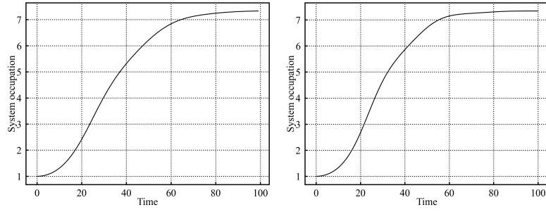
Figure 4: System evolution from occupied state propagated by dynamical map for \Delta t = 1, 0.1 respectively
