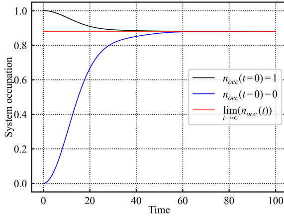
Figure 7: System occupation evolution computed using dynamical map for both occupied and unoccupied starts
