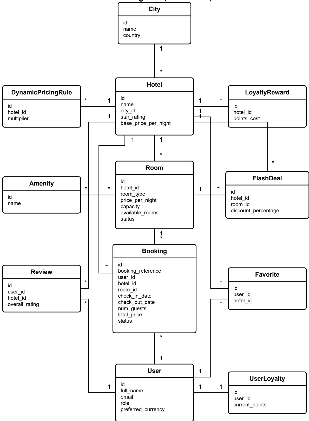
Class Diagram (HotelLink)
