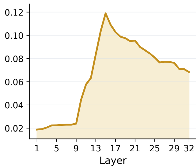
Consistency
