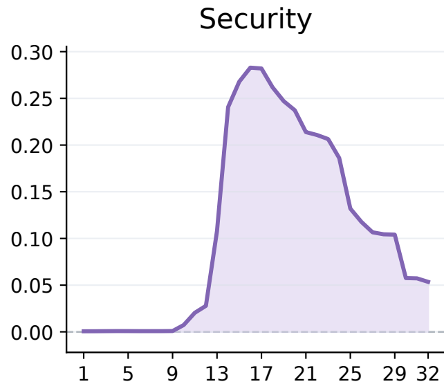
Discriminability
