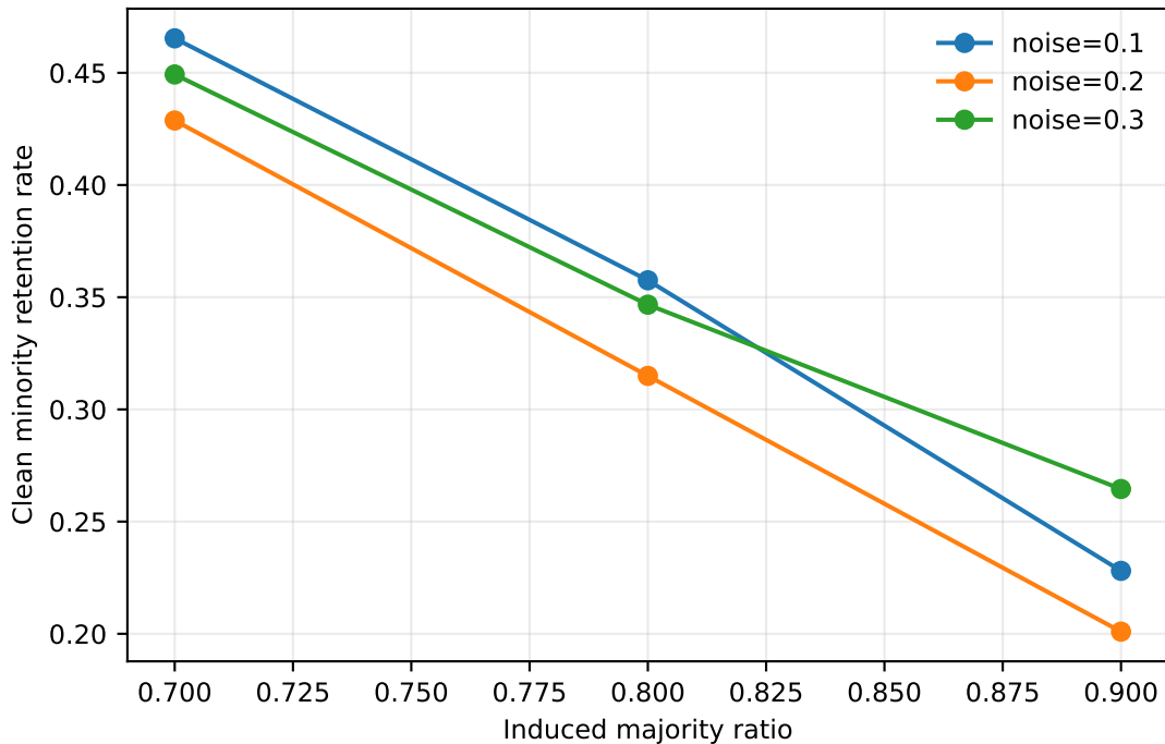
PMLB clean minority evidence falls with imbalance severity
