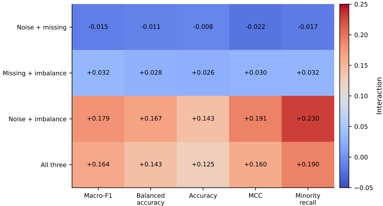
Interaction effects across evaluation metrics
