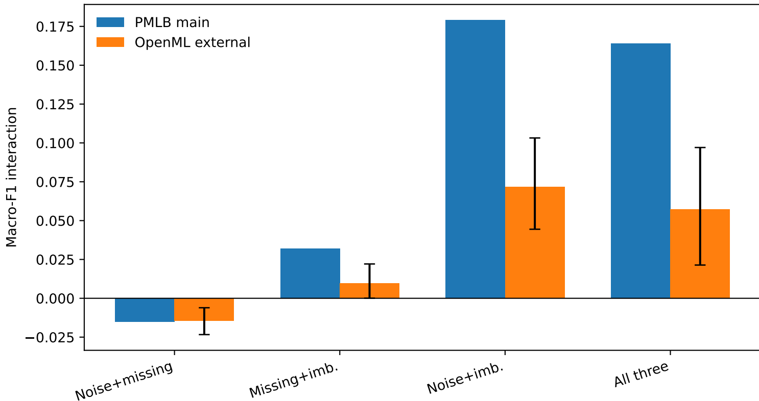
Main benchmark vs independent OpenML replication
