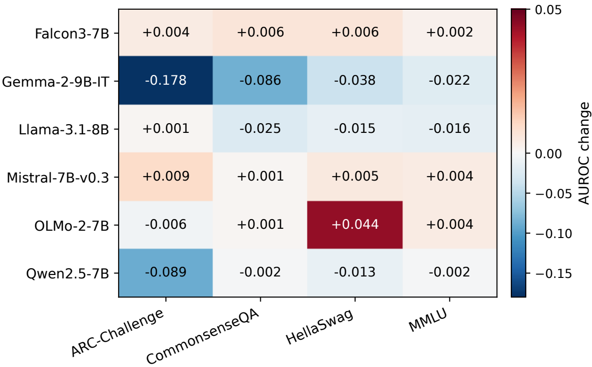
Seed-averaged AUROC change: full-vector augmentation - compact baseline
